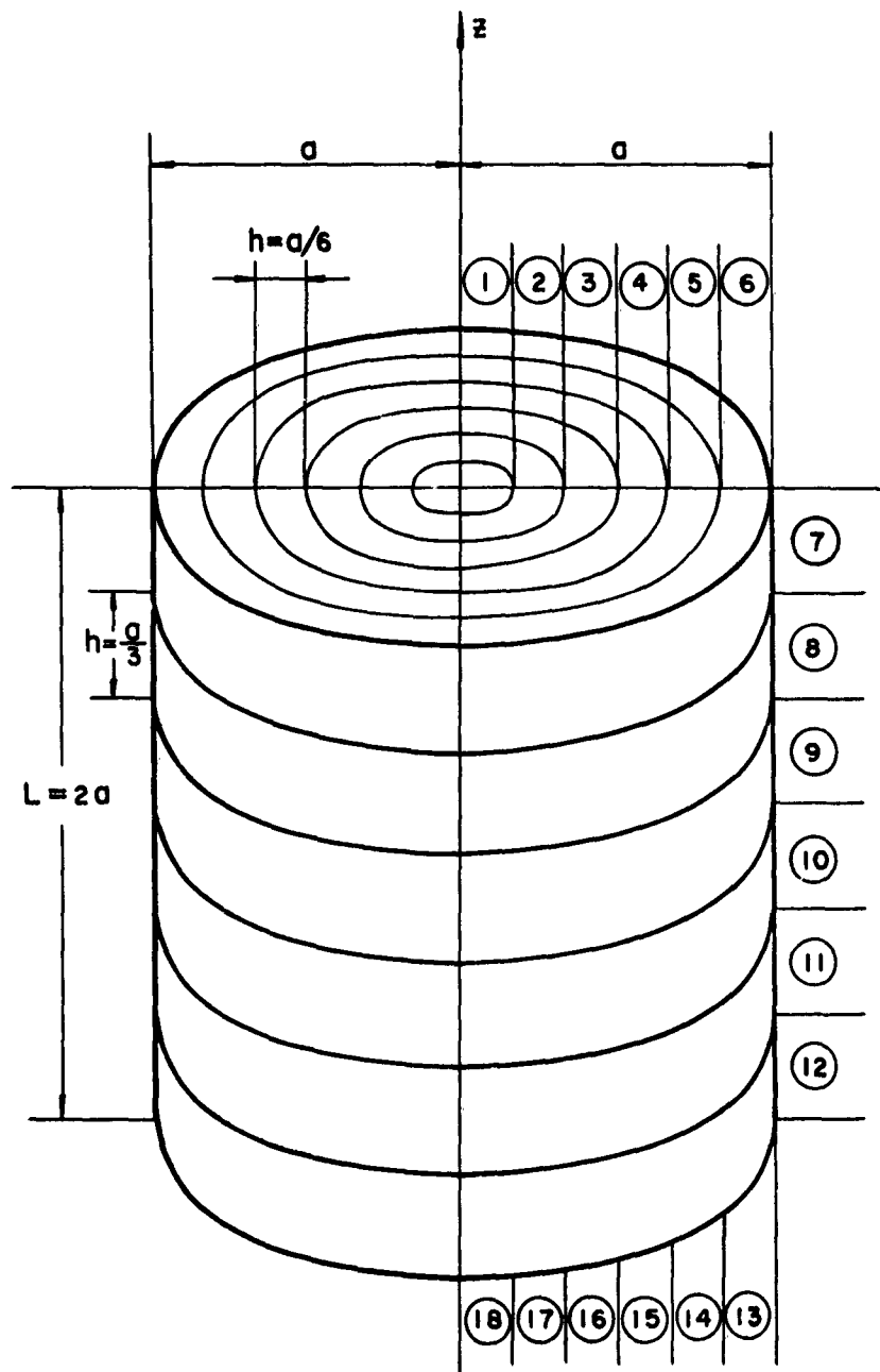
FIG. III-2 CYLINDER GEOMETRY
