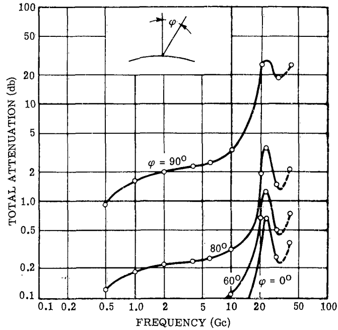
FIGURE 5. ONE-WAY TOTAL ATTENUATION THROUGH THE ATMOSPHERE BY OXYGEN AND WATER VAPOR [10]
