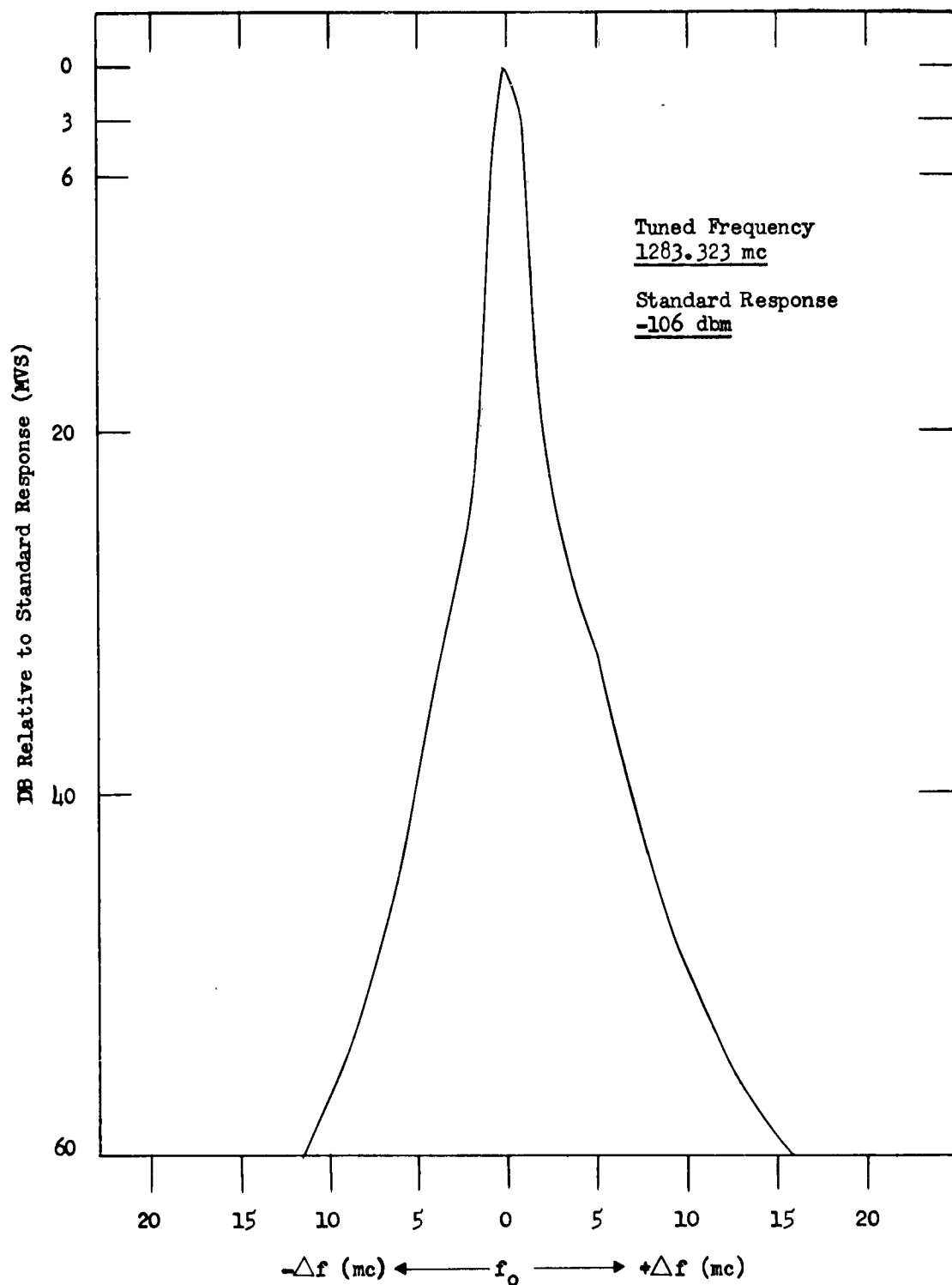
Figure 3.3.5.4 Normal Receiver Selectivity Curve - 9.0 usec Pulse
