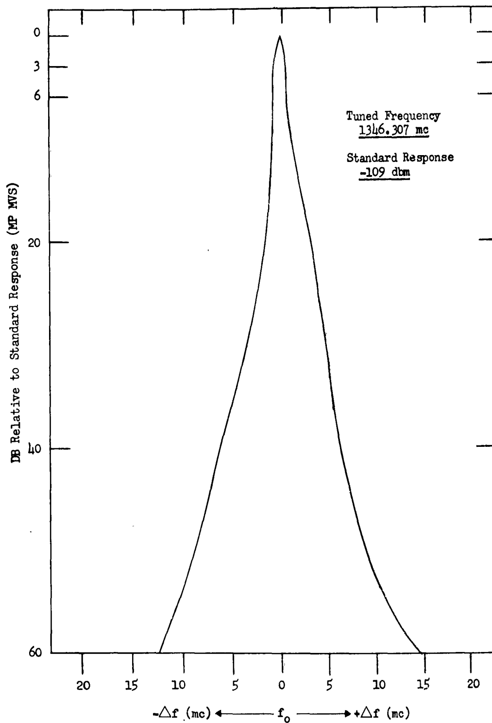
Figure 3.3.5.18 Normal Receiver Selectivity Curve - 30.0 usec Pulse
