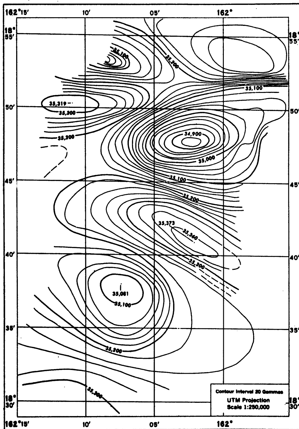
FIGURE 18 DEVELOPMENT AREA 2 MAGNETIC TOTAL INTENSITY CONTOUR CHART
