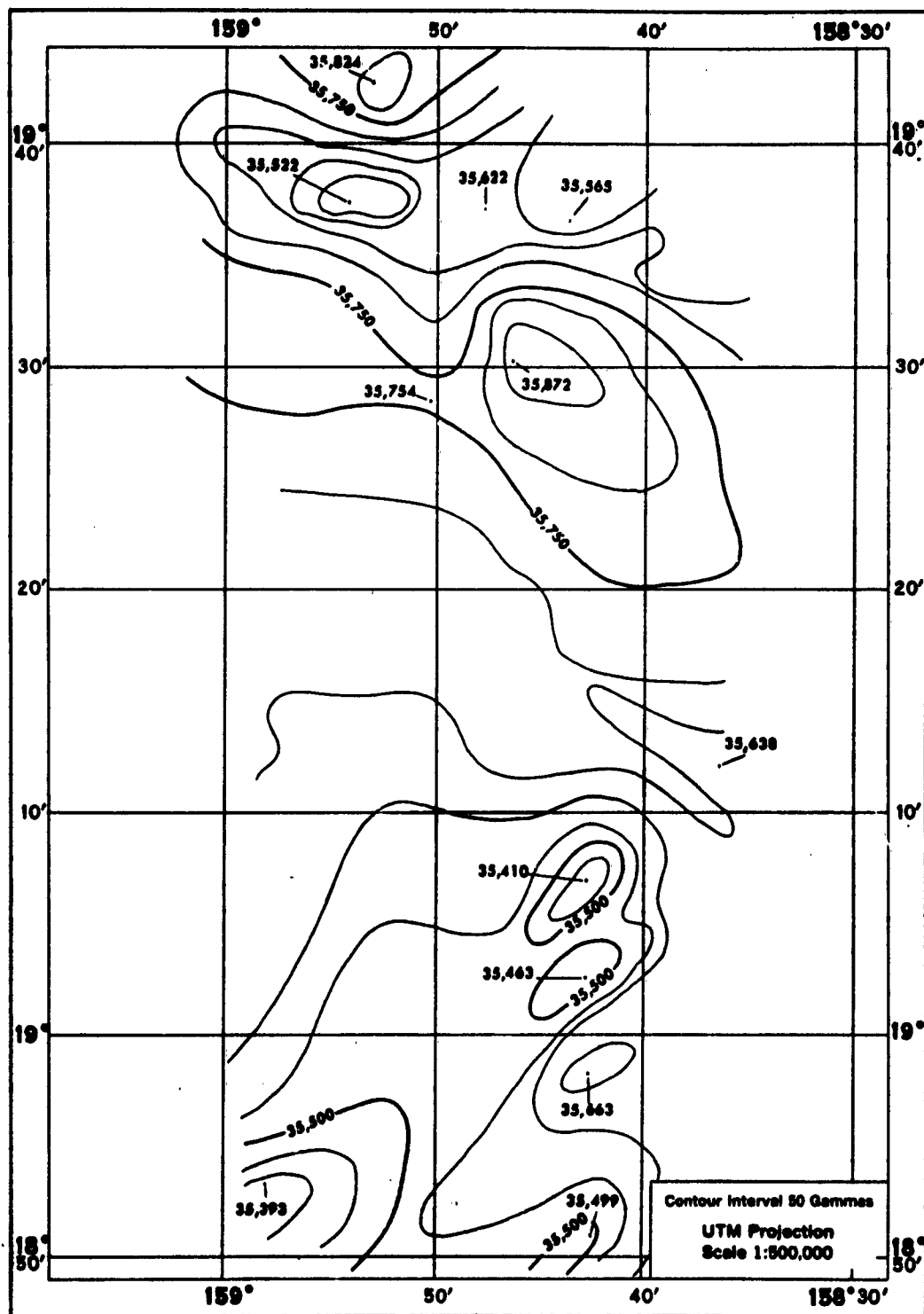
FIGURE 36 DEVELOPMENT AREA 8 MAGNETIC TOTAL INTENSITY CONTOUR CHART
