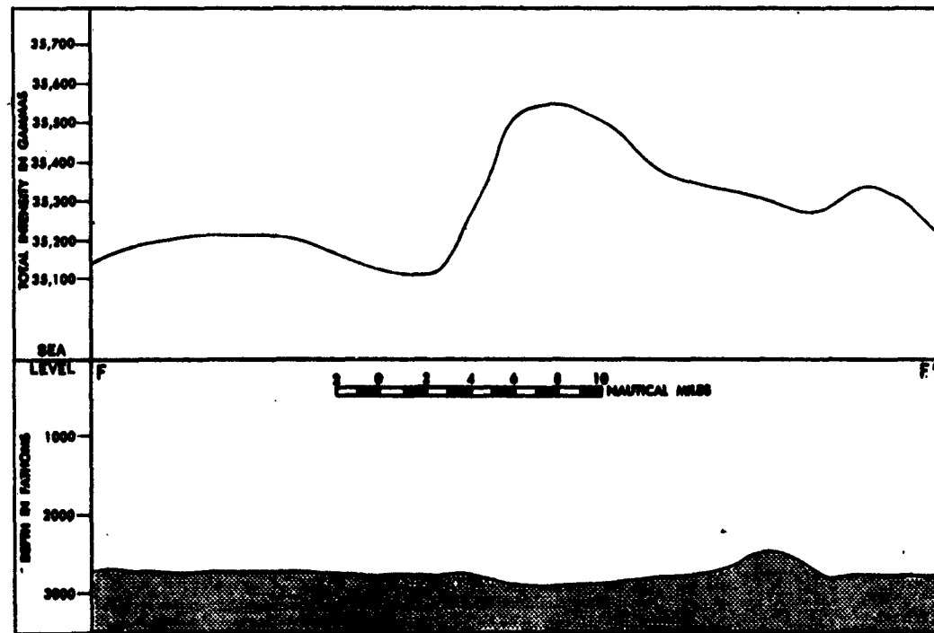
FIGURE 12 MAGNETIC AND BATHYMETRIC PROFILES F-F'
