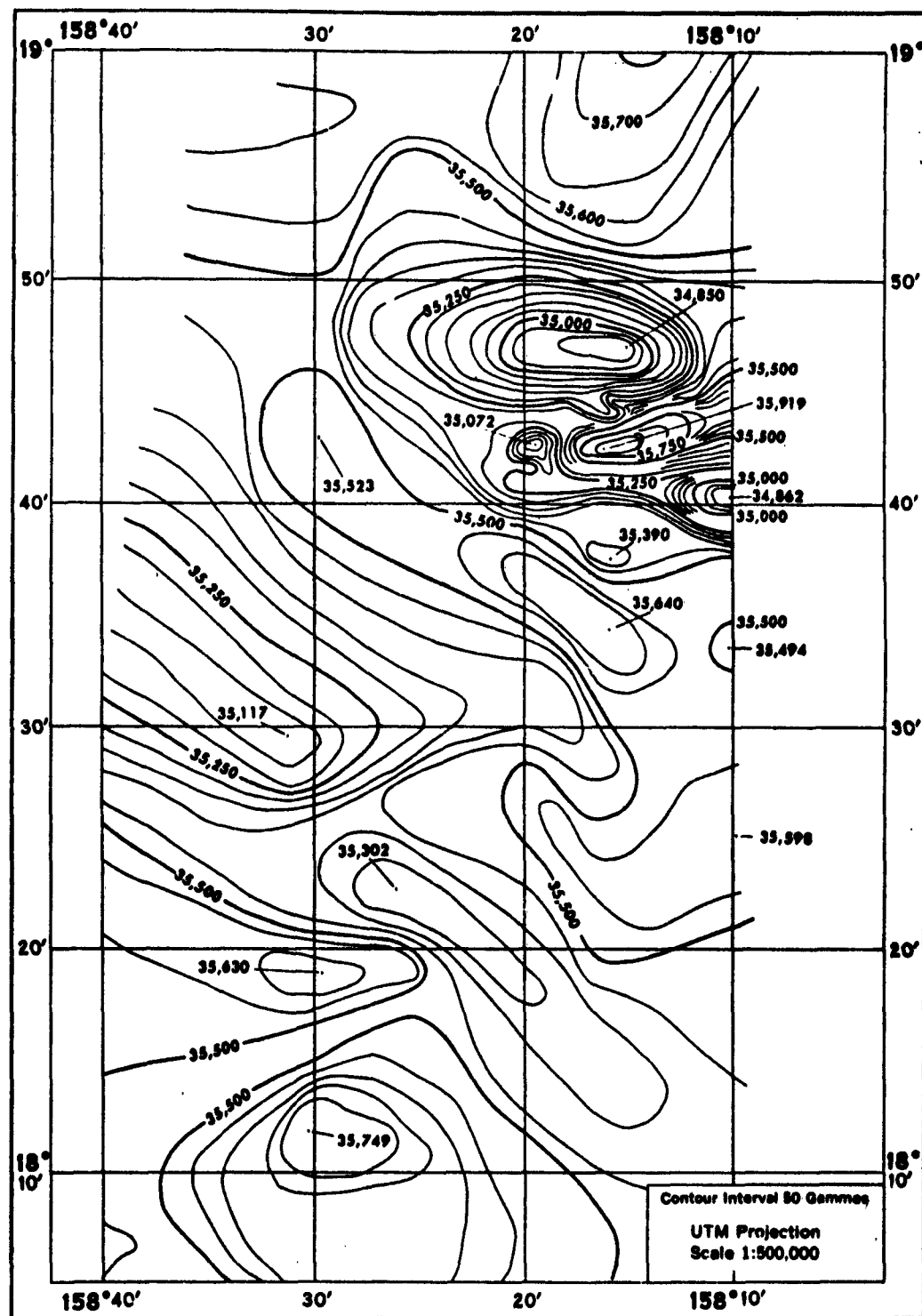
FIGURE 33 DEVELOPMENT AREA 7 MAGNETIC TOTAL INTENSITY CONTOUR CHART
