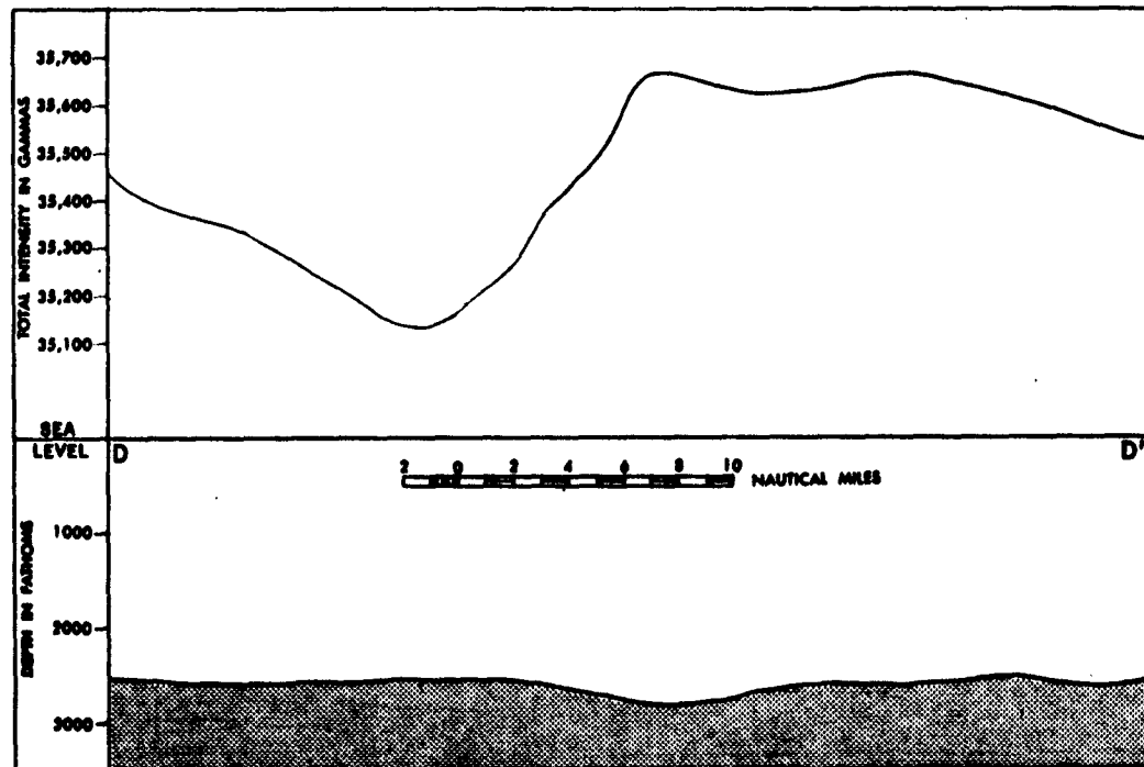
FIGURE 10 MAGNETIC AND BATHYMETRIC PROFILES D-D'
