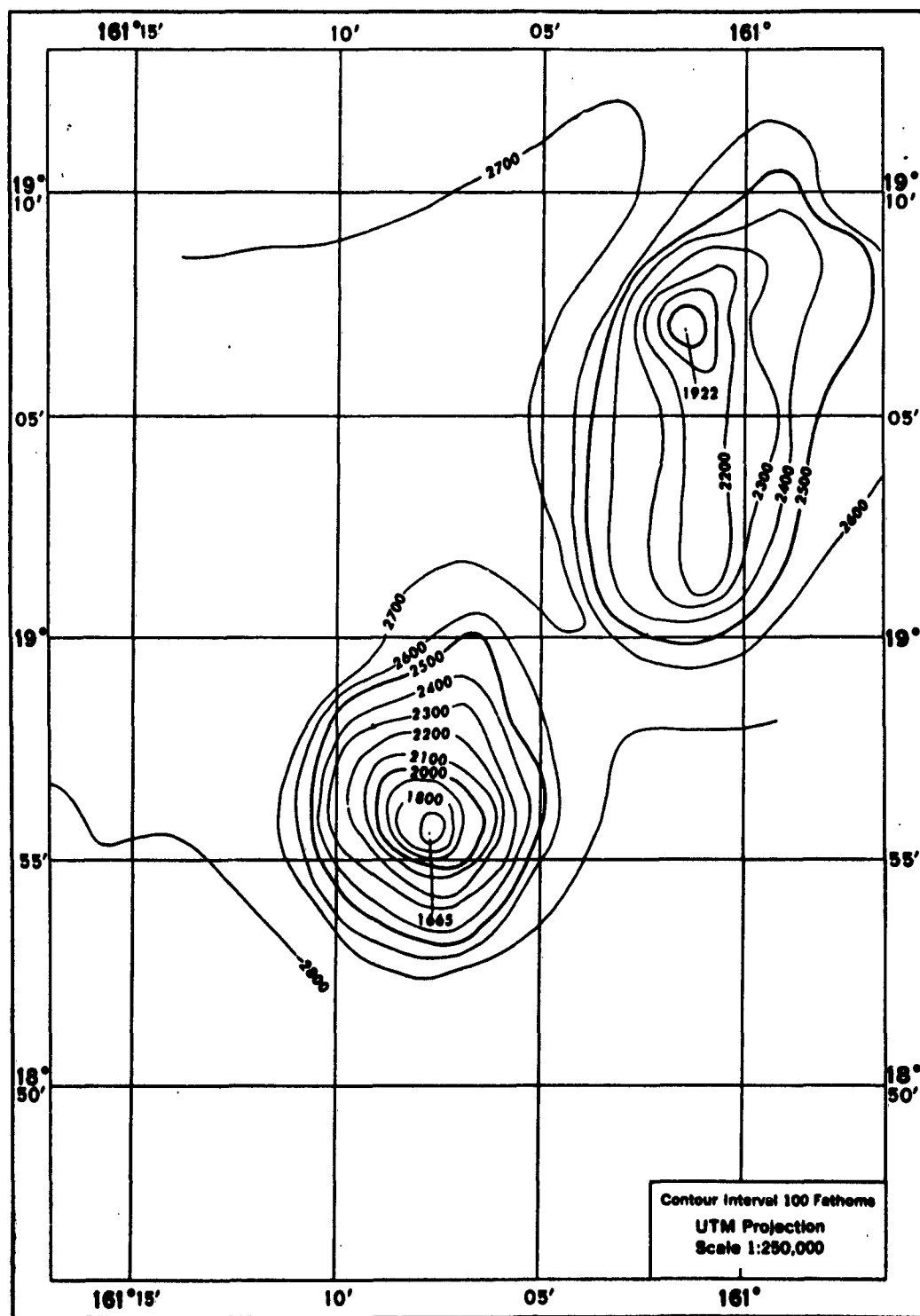
FIGURE 22 DEVELOPMENT AREA 3 BATHYMETRIC CONTOUR CHART
