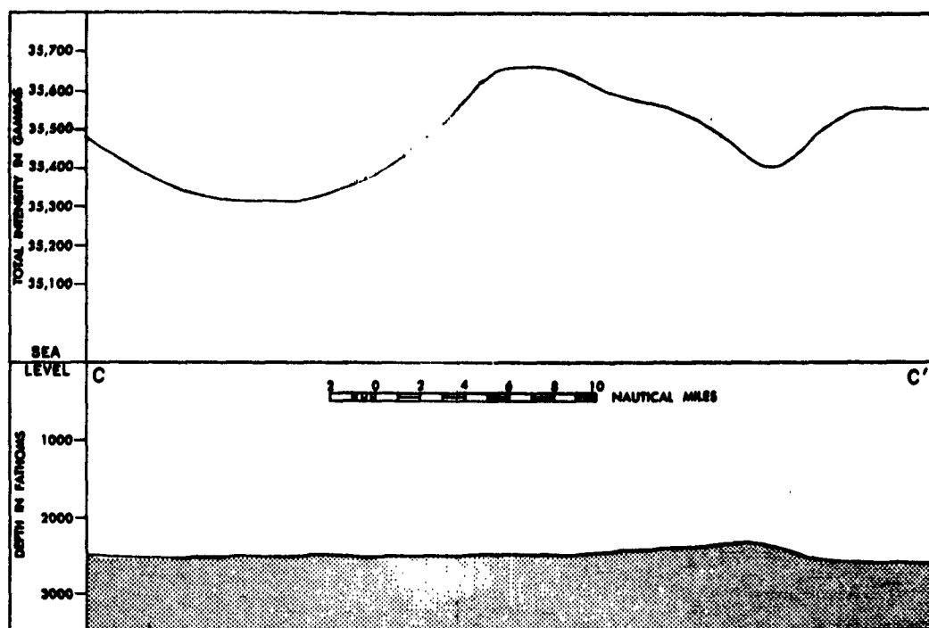
FIGURE 9 MAGNETIC AND BATHYMETRIC PROFILES C-C'
