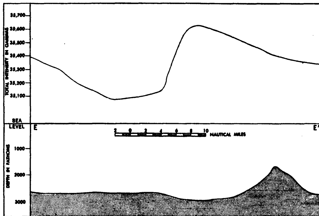
FIGURE 11 MAGNETIC AND BATHYMETRIC PROFILES E-E'
