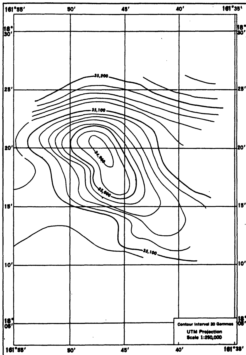
FIGURE 15 DEVELOPMENT AREA 1 MAGNETIC TOTAL INTENSITY CONTOUR CHART
