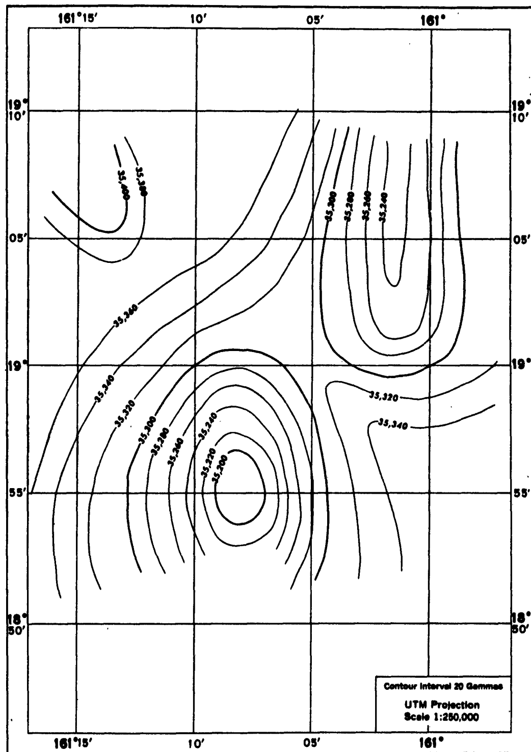
FIGURE 21 DEVELOPMENT AREA 3 MAGNETIC TOTAL INTENSITY CONTOUR CHART
