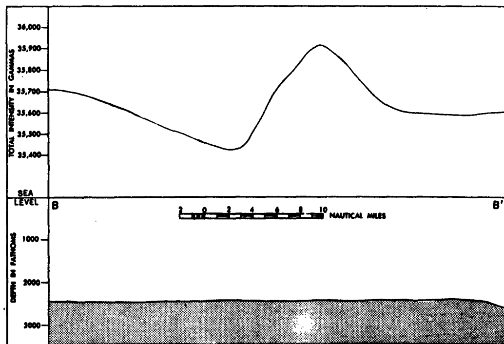
FIGURE 8 MAGNETIC AND BATHYMETRIC PROFILES B-B'
