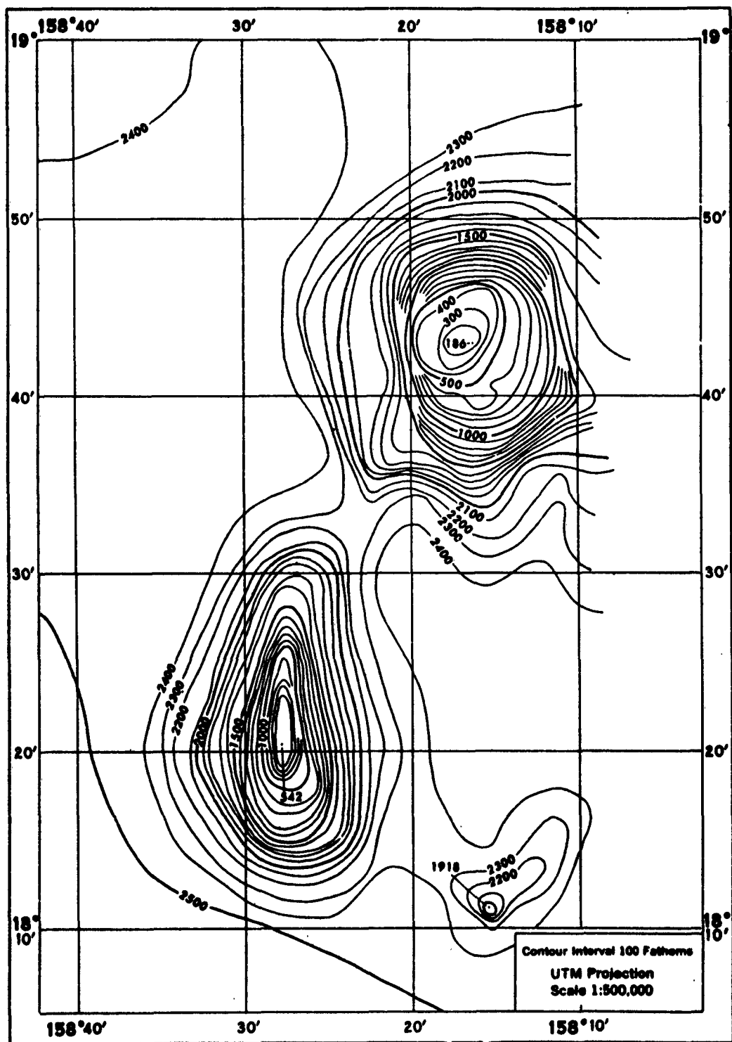
FIGURE 34 DEVELOPMENT AREA 7 BATHYMETRIC CONTOUR CHART
