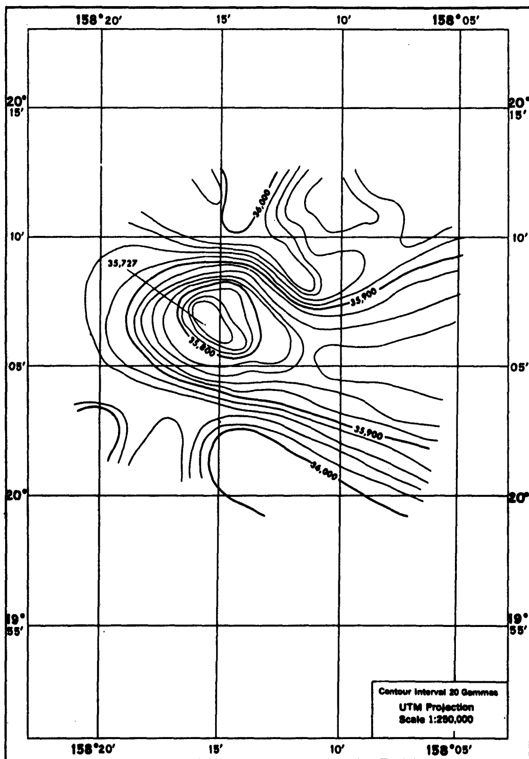
FIGURE 24 DEVELOPMENT AREA 4 MAGNETIC TOTAL INTENSITY CONTOUR CHART
