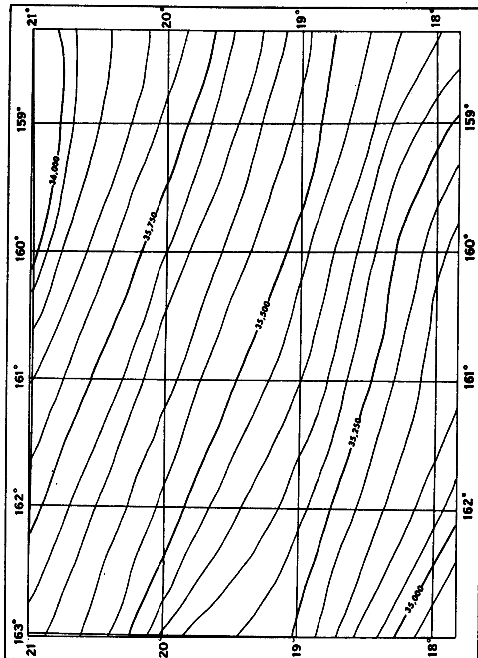
FIGURE 6 COMPUTED REGIONAL MAGNETIC INTENSITY CONTOUR CHART UTM Projection Contour Interval 50 Gammas
