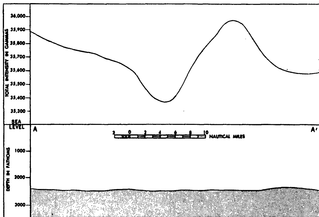
FIGURE 7 MAGNETIC AND BATHYMETRIC PROFILES A-A'
