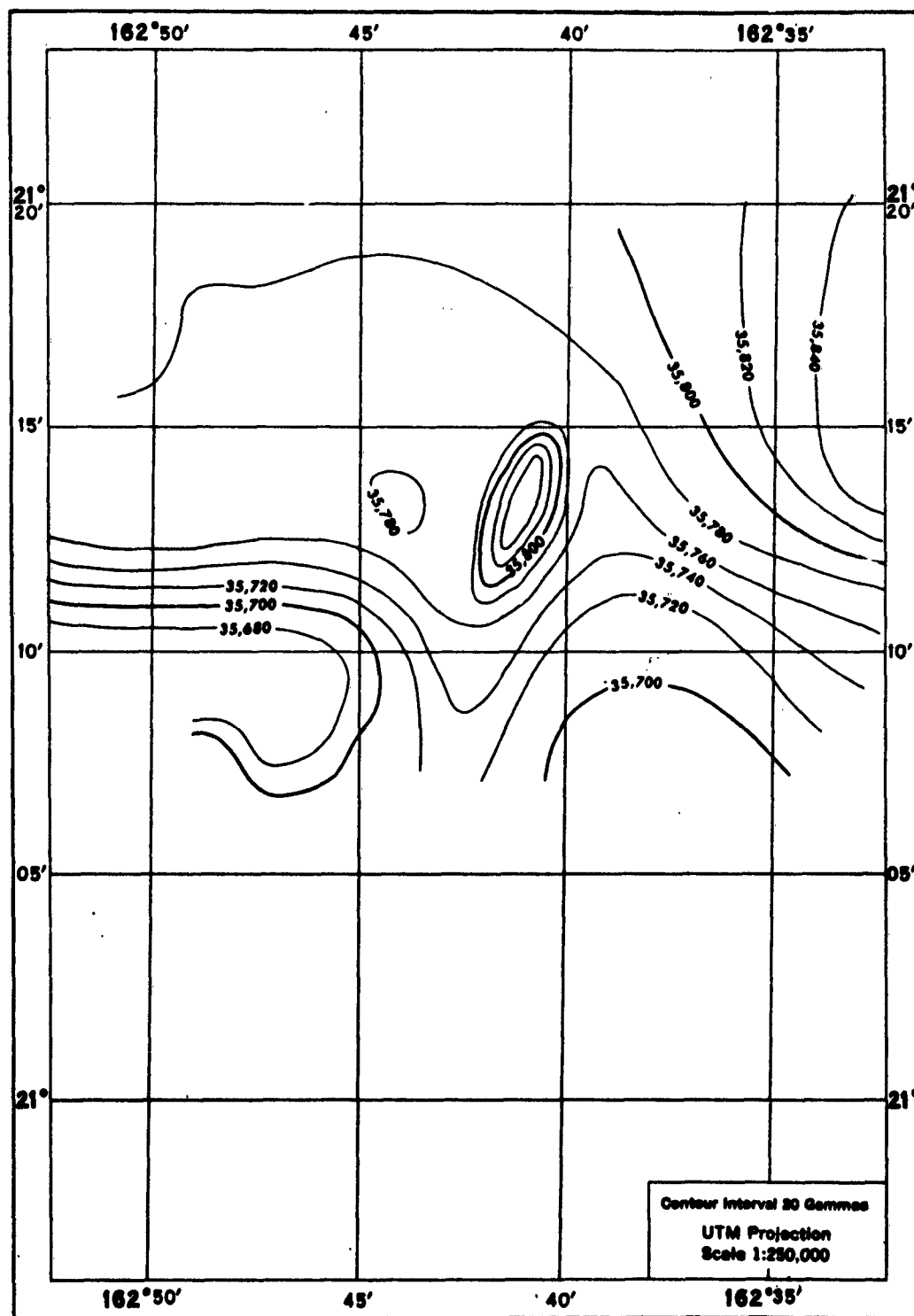
FIGURE 30 DEVELOPMENT AREA 6 MAGNETIC TOTAL INTENSITY CONTOUR CHART
