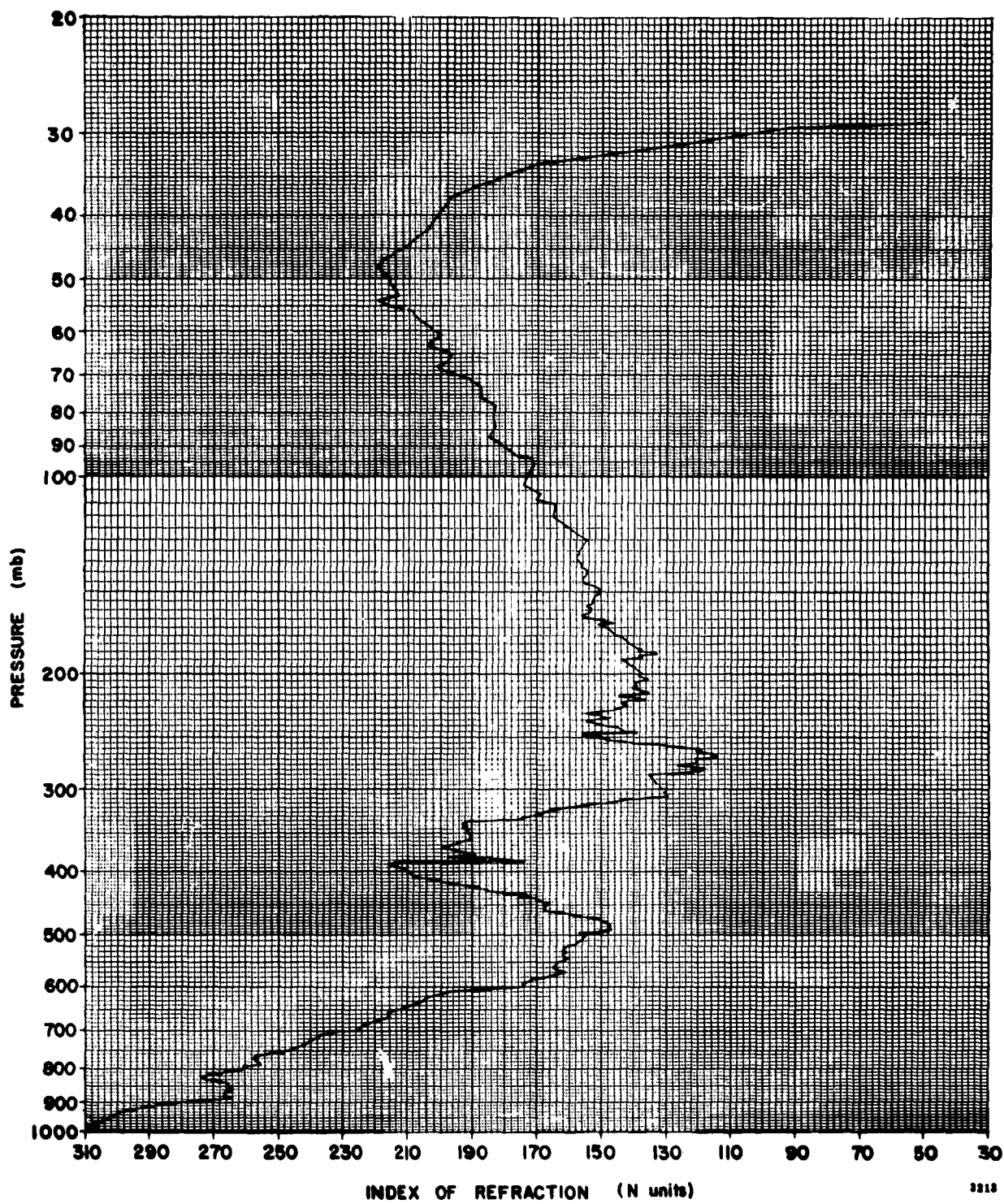
Figure 5. Refractometer Data
