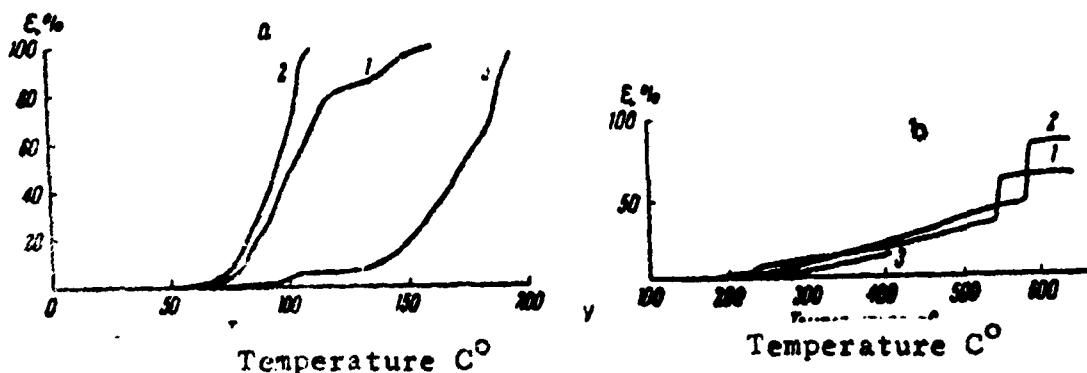
Fig. 1. Thermomechanical curves of polymers; a -- before heating; b -- after heating at 200°
