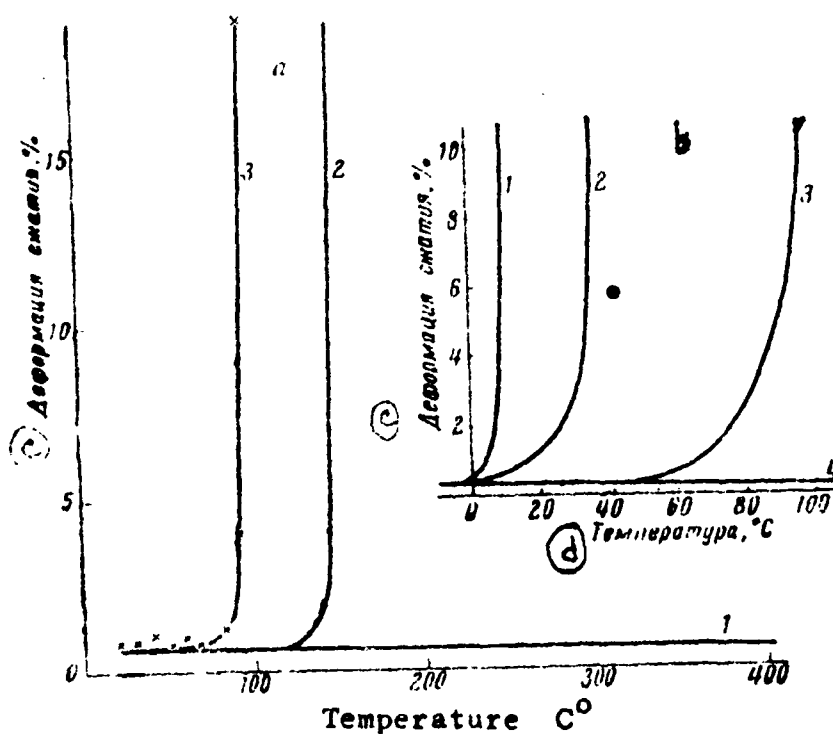
Figure 1. Thermomechanical curves.
