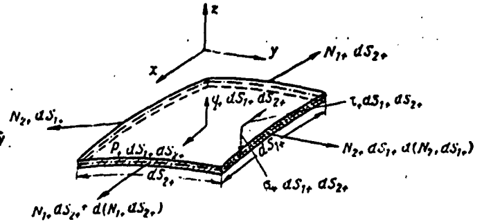
Fig. 4. An element of the outer supporting layer of a three-layer shell.
