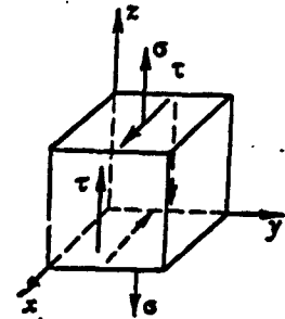
Fig. 6. Model of the stressed state of the filler.
