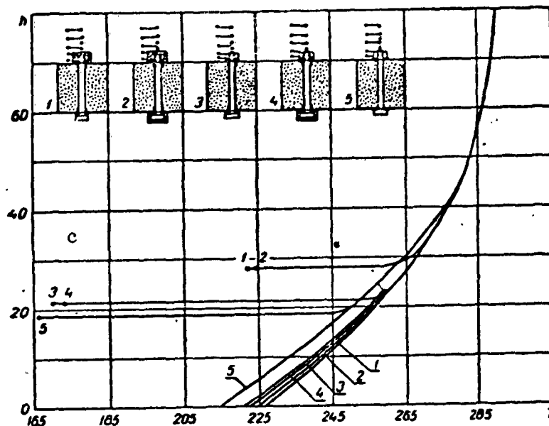
Fig. 2 (continued). b) Different heat bridge structures of the same material (carbon steel) on the air side: 1-5) types of heat bridges, the temperature on the projections of which is shown by the corresponding numbers on the horizontals. c) Different insulation structures at the ends of heat bridges all of the same material: 1-5) types of insulating structures, the temperature on the projections of which is shown by the corresponding numbers on the horizontals.
