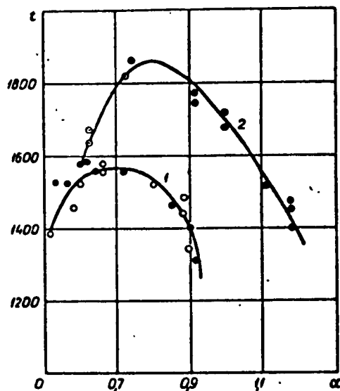
Fig. 2. Dependence of temperature in circulation zone t ( ^{\circ}\text{C} ) on the excess air ratio \alpha : 1) for rod d = 4 mm (the curve is plotted in conformity with the characteristic of the initial mixture); 2) for conical stabilizer d = 5 mm.
