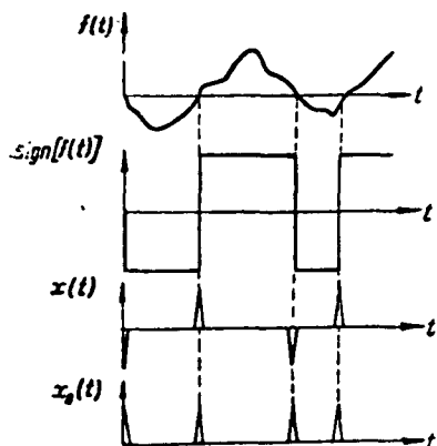
Fig.1. Transformation of input signal in measuring device. We will examine a circuit relay function and pulse, which correspond to zeros of output function. diagram of a correlation velocity measuring f(t) -signal at output of phototransmitter; \text{sign}[f(t)] -relay function at output of for device (fig.2). The signals coming from ming line; x(t) -differentiated pulses; x_0(t) -output signal of converter (monop photomultipliers FP_1 and FP_2 are amplified lar pulses which correspond to zeros of output function).
