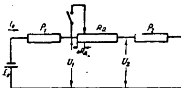
Fig.2. Equivalent electric circuit to determine changes in values at the initial moment of the transient process.
