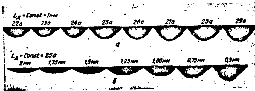
Fig. 1. Lateral microsections of plates fused with tungsten electrode in an Argon medium at various arc current (a) and at its various length (b).
