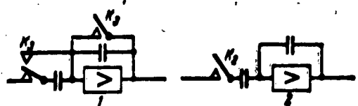
Fig.8. Arrangements of memory devices.
