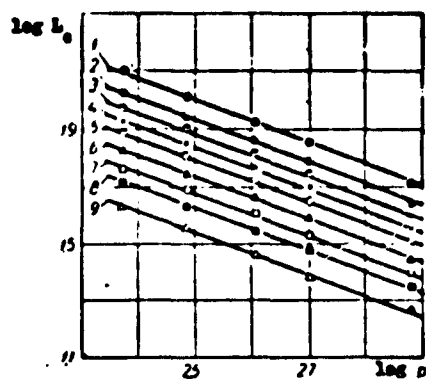
Fig. 2. The dependence of the averaged values of the length of the combustion zone L_c (mm) on the pressure p (mm Hg) in logarithmic coordinates for various ranges of variation of CO_2 content (%): 1) from 1 to max.; 2) from 2 to max.; 3) from 3 to max.;... (Slope of straight lines n = -0.75 ; Re = 8000 )
