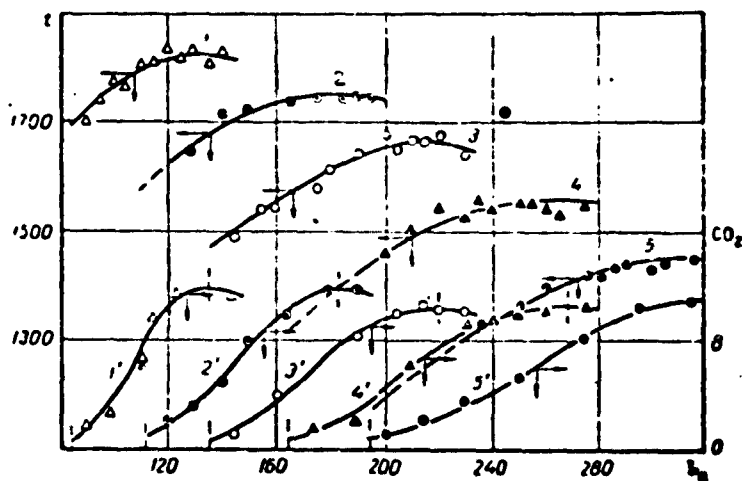
Fig. 1. The relationship between the length of the combustion zone L_c (mm), the temperature t ( ^{\circ}\text{C} ), and the \text{CO}_2 content (%) for pressures in a pressure chamber at \text{Re} = 8000 : 1,1') 760; 2,2') 500; 3,3') 400; 4,4') 304; 5,5') 235 mm Hg.
