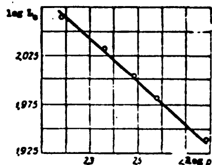
Fig. 3. The dependence of the length of the combustion zone L_c (mm) on the pressure p (mm Hg) when W = \text{constant} , p varies from 610 to 152.2 mm Hg, Re varies from 16,000 to 4000, CO_2 varies from 1% to maximum, n = -0.25 .
