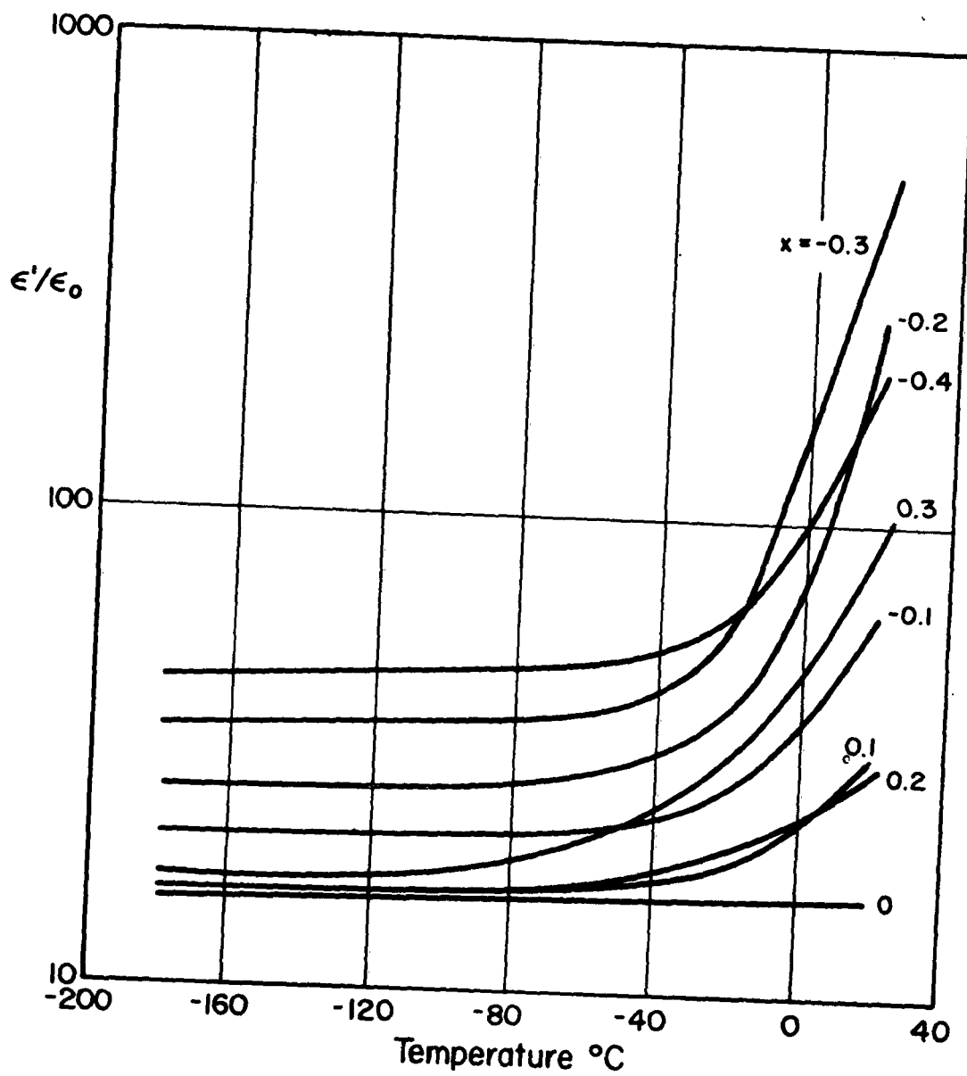
Fig. 3.5. Dielectric constant vs. temperature for series (3+x)\text{Y}_2\text{O}_3 \cdot (5-x)\text{Fe}_2\text{O}_3 . Measurements at 1000 cps.
