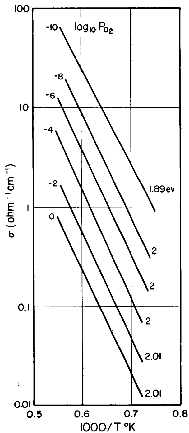
Fig. 9. 12. Conductivity of \text{TiO}_2 as a function of reciprocal temperature for various oxygen pressures. Activation energy ranges from about 1.9 to 2 eV.
