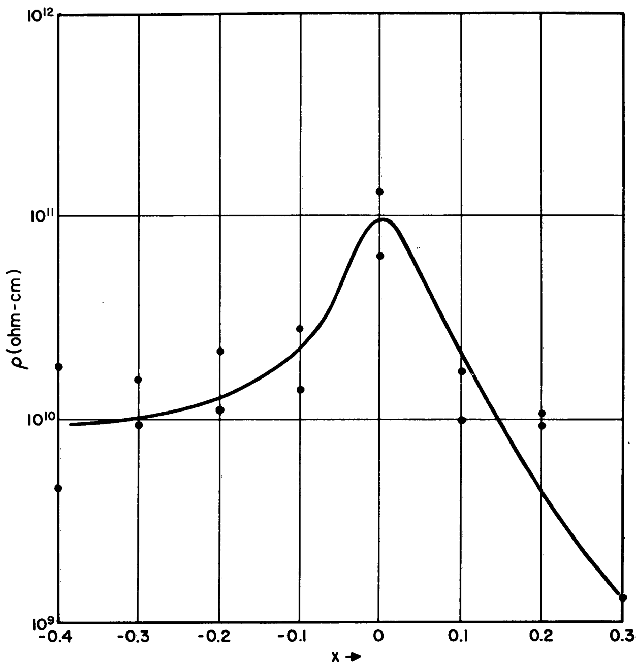
Fig. 3.1. D-c resistivity for series (3+x)\text{Y}_2\text{O}_3 \cdot (5-x)\text{Fe}_2\text{O}_3 at 100^\circ\text{C} . Data shown are for two samples of each composition.
