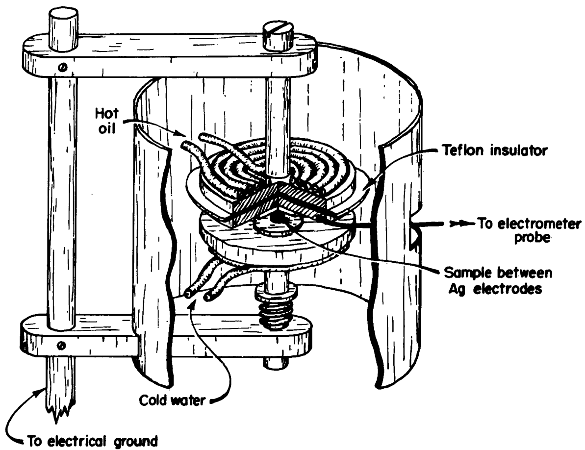
Fig. 3. 4. Sample holder for resistivity and thermoelectric measurements.
