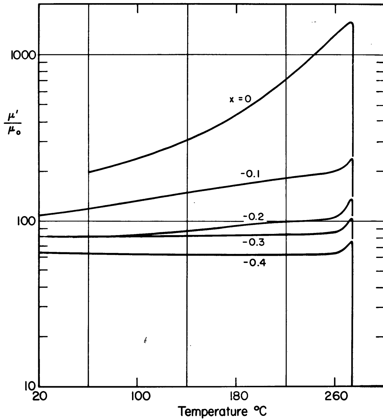
Fig. 4.13. Initial permeability vs, temperature at 1 kc for series (3 + x)Y_2O_3 \cdot (5 - x)Fe_2O_3 ; x \leq 0 .
