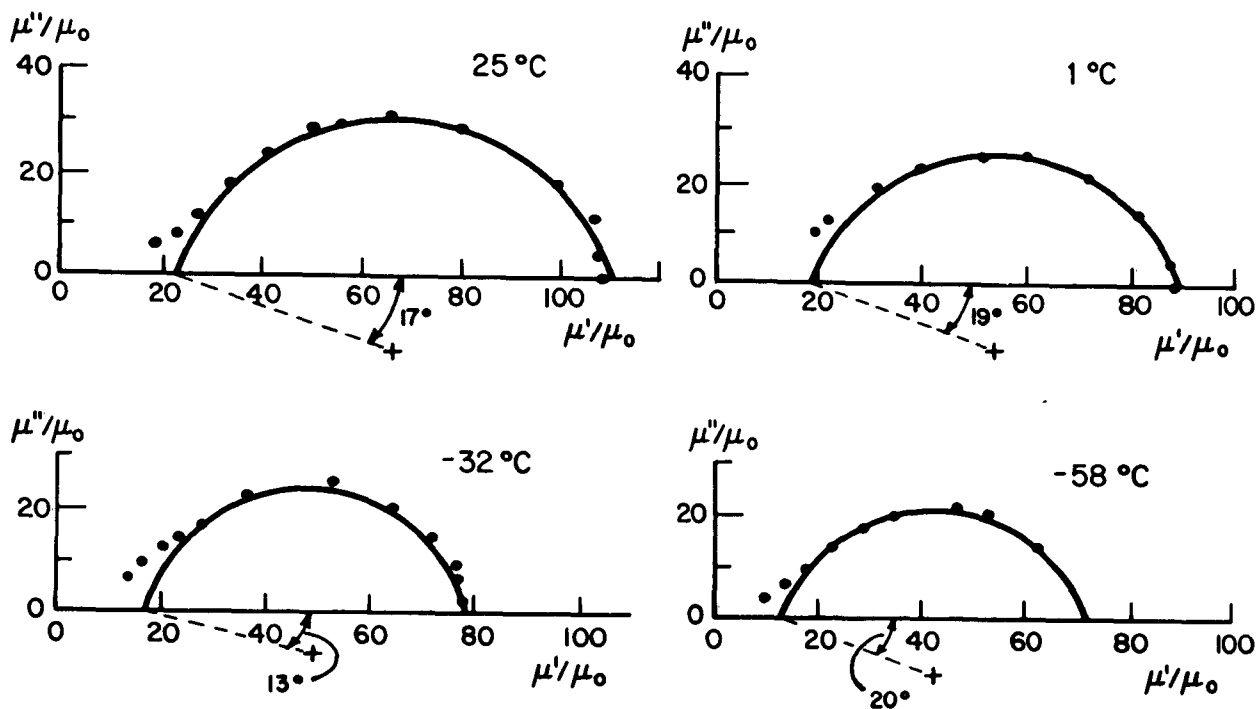
Fig. 4.10. Cole-Cole plots for polycrystalline YIG at several temperatures.
