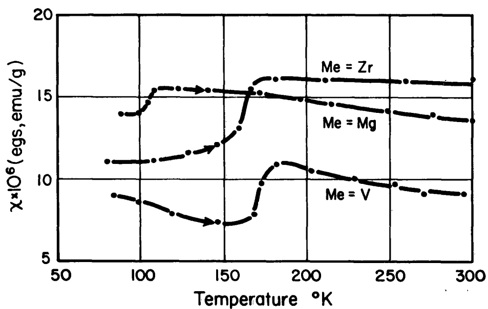
Fig. 9. 5. Susceptibility as a function of temperature for compositions \text{Me}_{0.04}\text{V}_{1.96}\text{O}_3 fired at 1360^{\circ}\text{C} .
