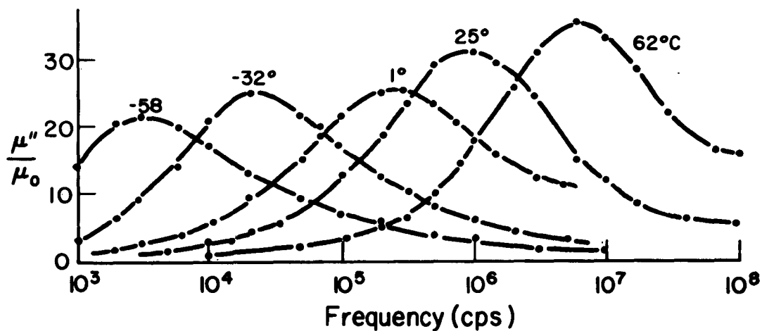
Fig. 4. 3. Magnetic-loss spectra of polycrystalline YIG at several temperatures.
