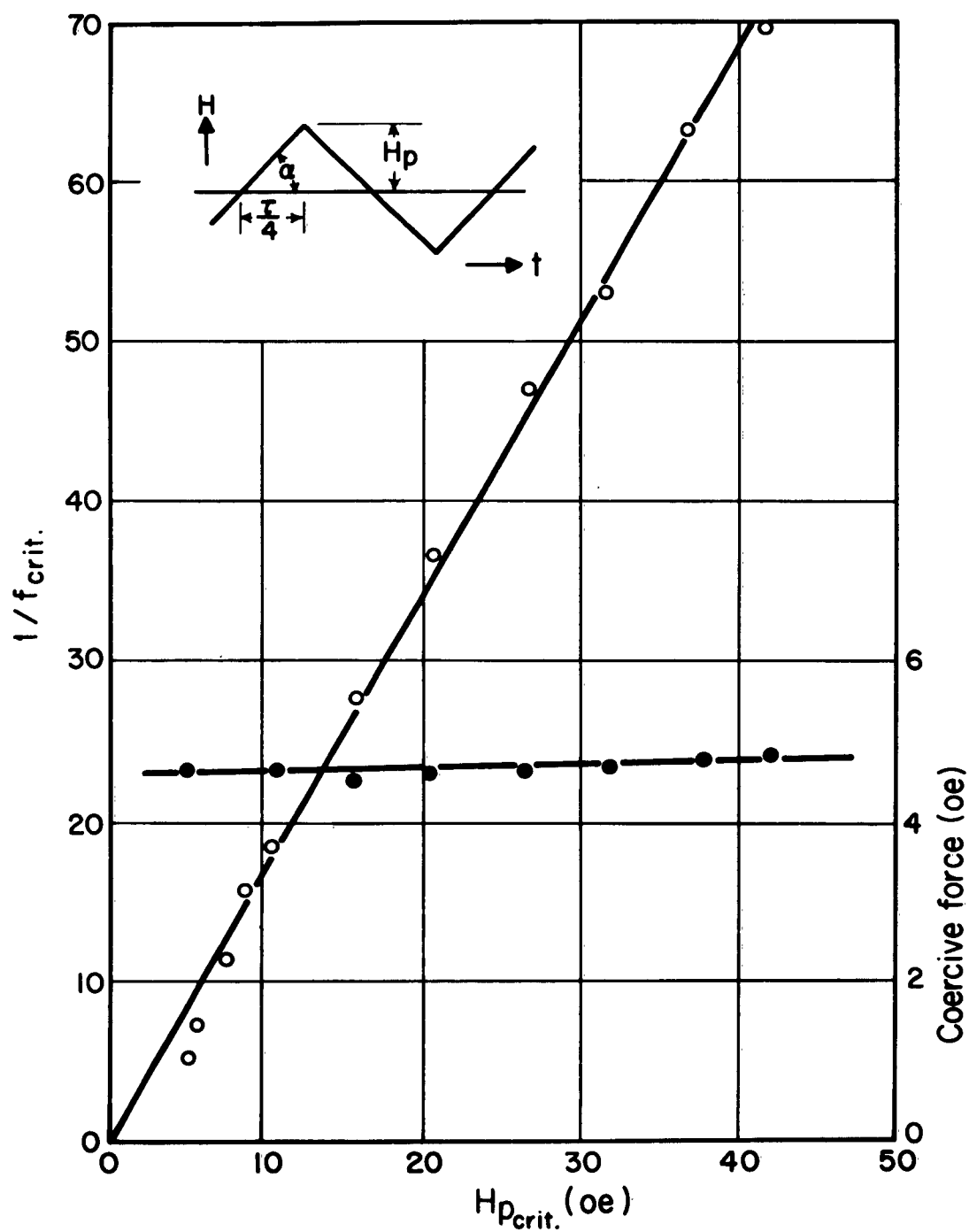
Fig. 6.5. Critical frequency and coercive field for polycrystalline YIG at -196^{\circ}\text{C} . Excitation wave form is shown in inset.
