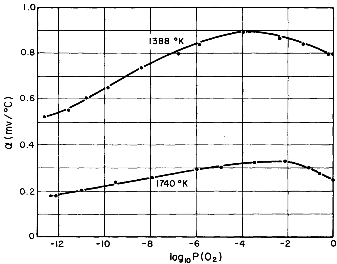
Fig. 9.11. Thermoelectric power of TiO_2 as a function of oxygen pressure (in atmospheres).
