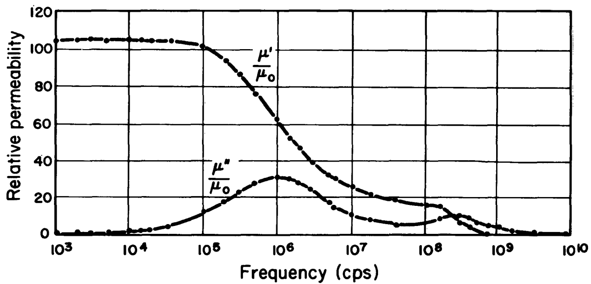
Fig. 4. 1. Complex initial permeability spectrum of ceramic YIG at room temperature.
