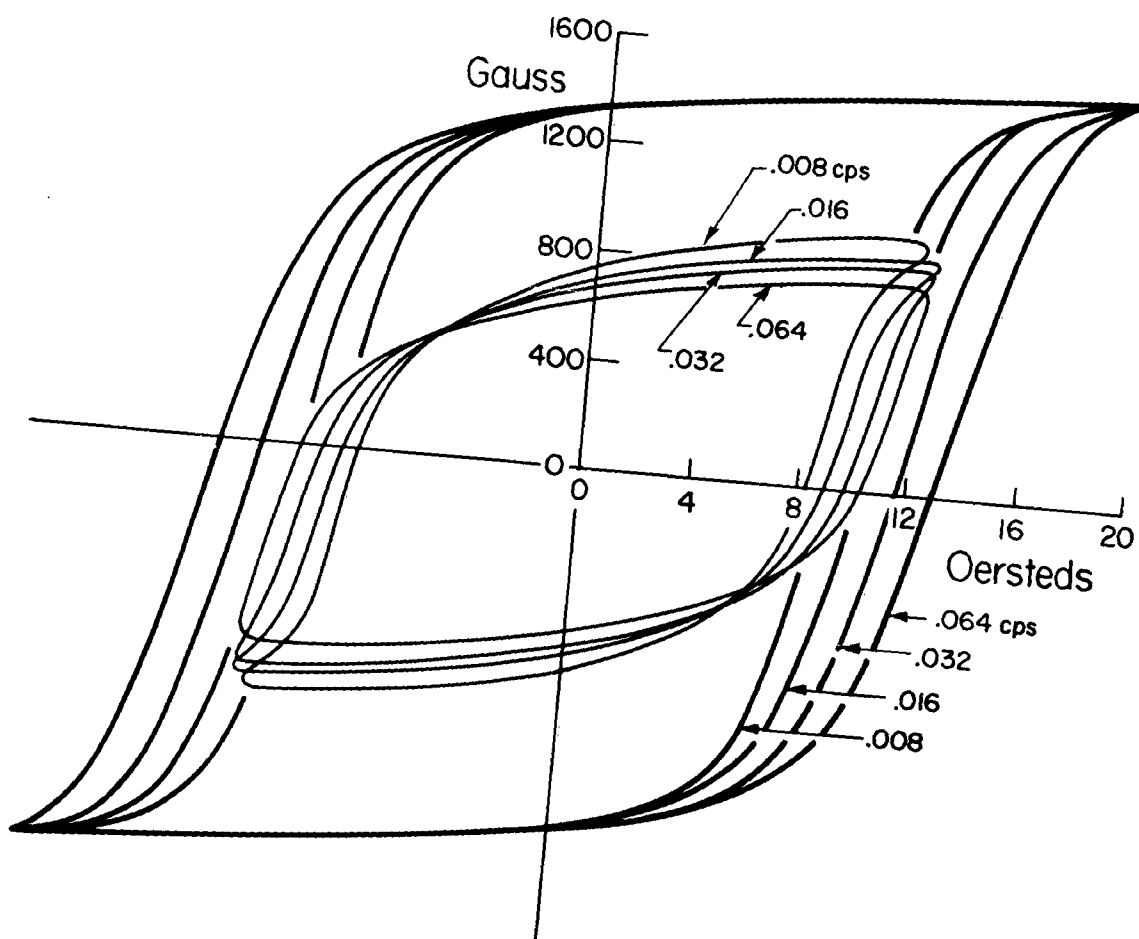
Fig. 6.6. Hysteresis loops for a YIG sample at -195^{\circ}\text{C} . Frequency below threshold for dynamic squareness. Sinusoidal current excitation.
