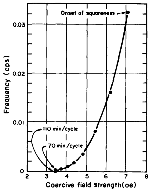
Fig. 6.7. Dependence of coercive force upon frequency for YIG sample at frequencies below threshold for dynamic squareness.
