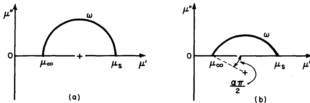
Fig. 4.9. Cole-Cole plots: (a) single relaxation time constant; (b) distribution of relaxation times.
