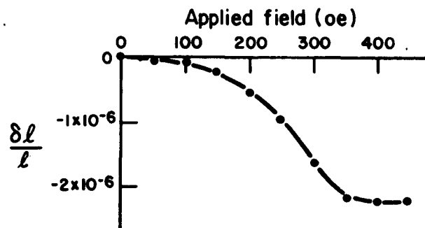
Fig. 8.2. Magnetostriction in [111] for single crystal (110) -plane disk of YIG.
