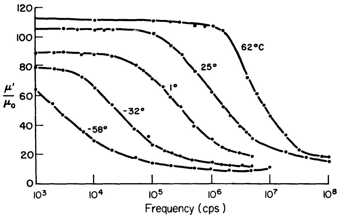
Fig. 4. 2. Permeability spectra of polycrystalline YIG at several temperatures.
