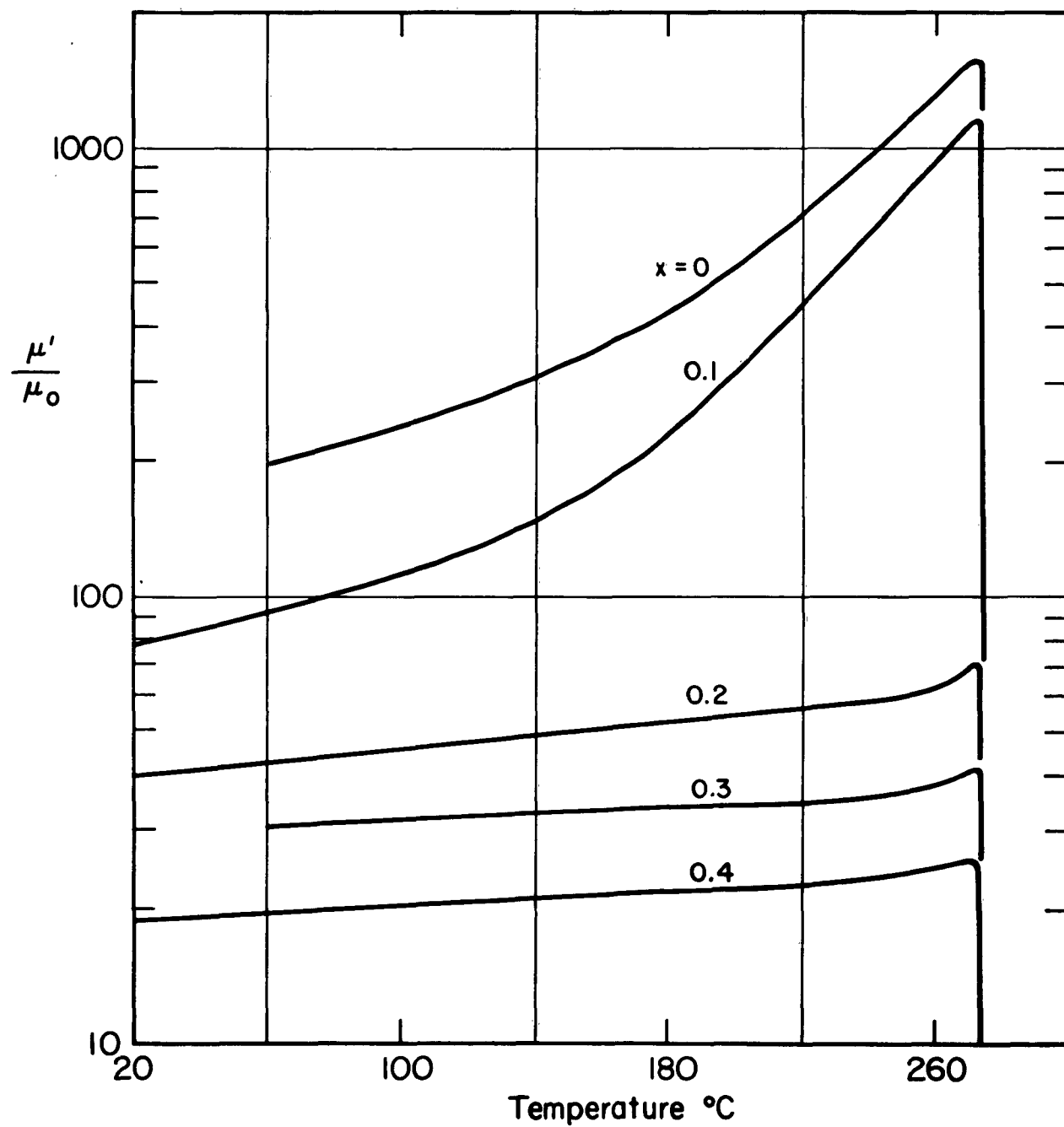
Fig. 4.12. Initial permeability vs. temperature at 1 kc for series (3+x)\text{Y}_2\text{O}_3 \cdot (5-x)\text{Fe}_2\text{O}_3 ; x \geq 0 .
