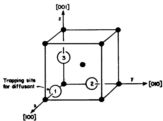
Fig. 6.10. Crystal structure employed in dynamic squareness model.
