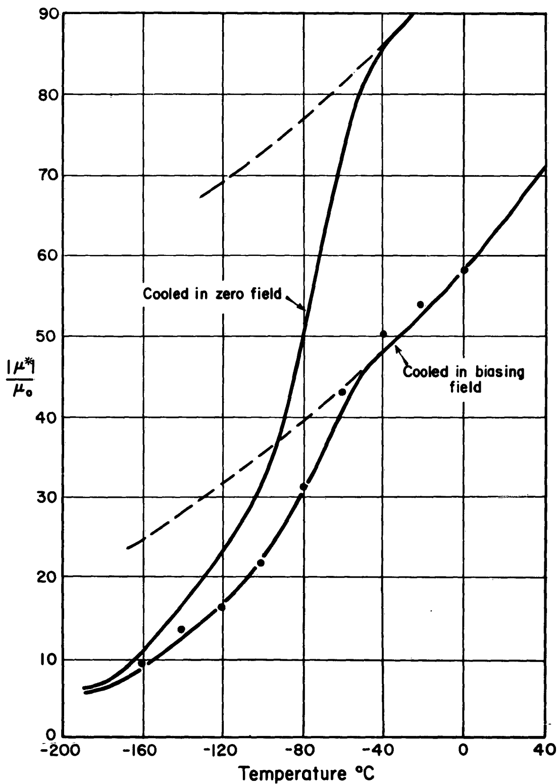
Fig. 4. 11. Permeability of ceramic YIG at 1 kc as a function of temperature. Curves are experimental; points are calculated from Eq. 4. 24.
