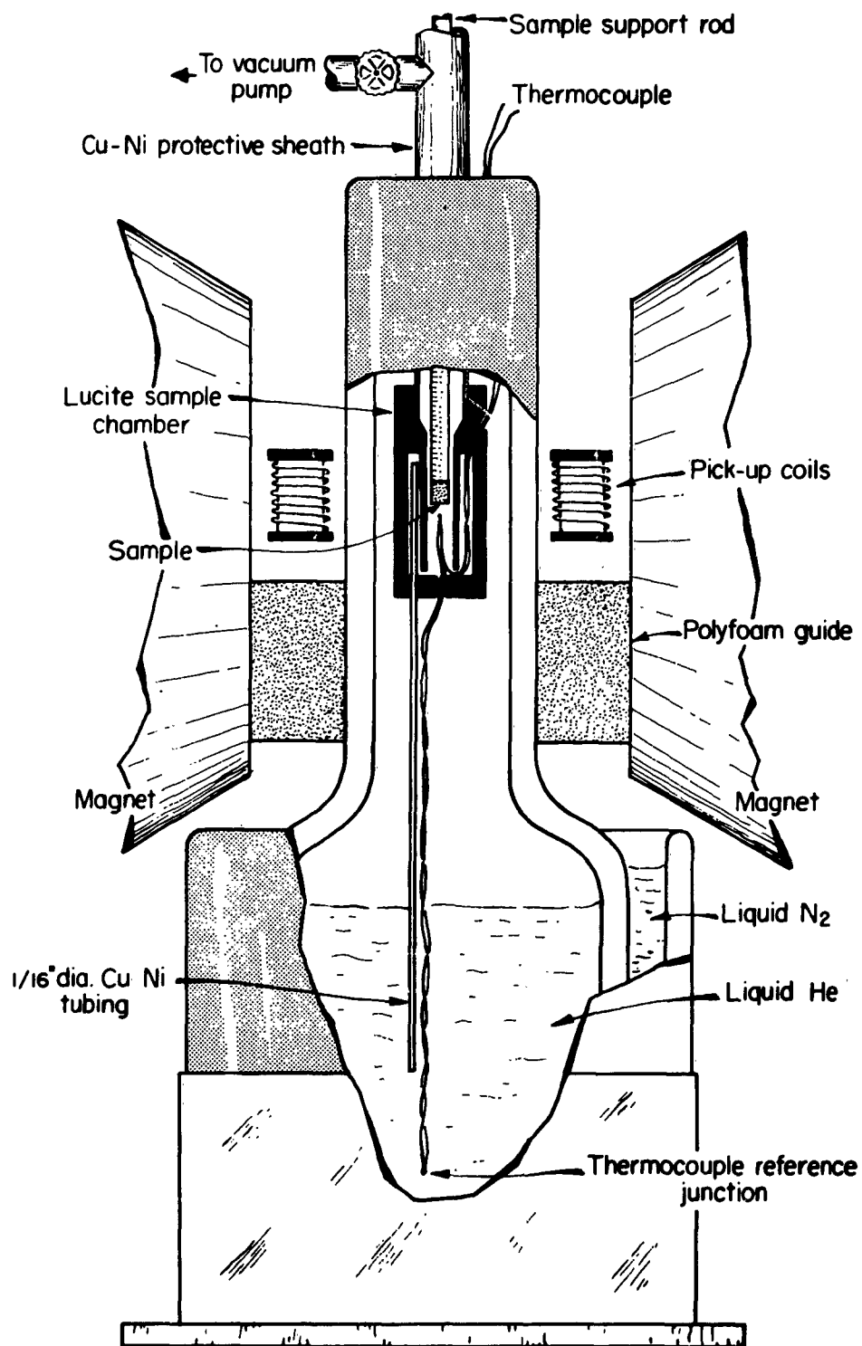
Fig. 10.4 - Auxiliary apparatus for measurement over range 4-55°K
