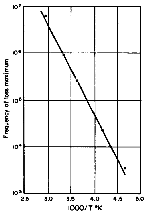
Fig. 4. 4. Frequency of magnetic loss maximum as a function of reciprocal temperature (YIG).
