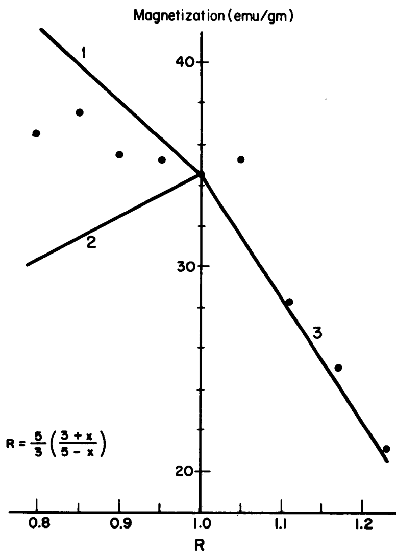
Fig. 2.2. Saturation magnetization of ceramic garnets at -196^{\circ}\text{C} . Points are experimental; curve (1) is based on the assumption that excess iron precipitates as magnetite; for curve (2) excess iron is assumed to precipitate as hematite; for (3) excess yttrium precipitates as \text{YFeO}_3 .
