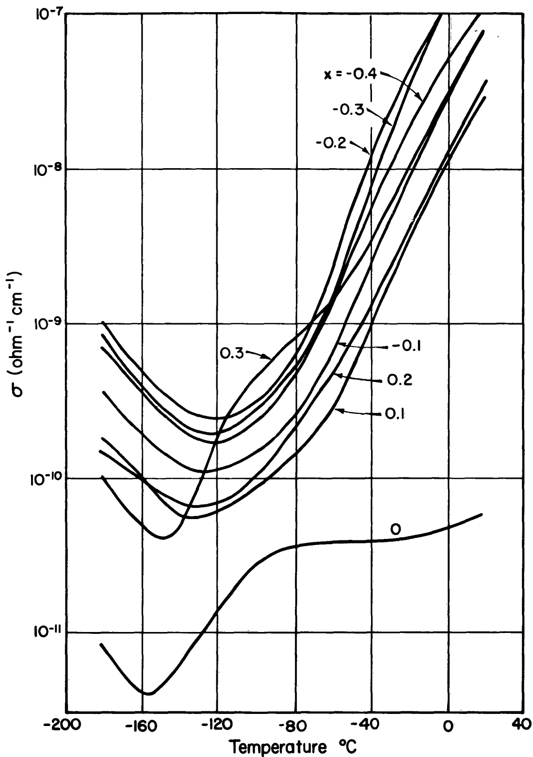
Fig. 3.6. Dielectric conductivity vs. temperature for series (3+x)\text{Y}_2\text{O}_3 \cdot (5-x)\text{Fe}_2\text{O}_3 at 1000 cps.
