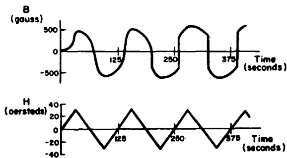
Fig. 6.8. Buildup of dynamic squareness in YIG.
