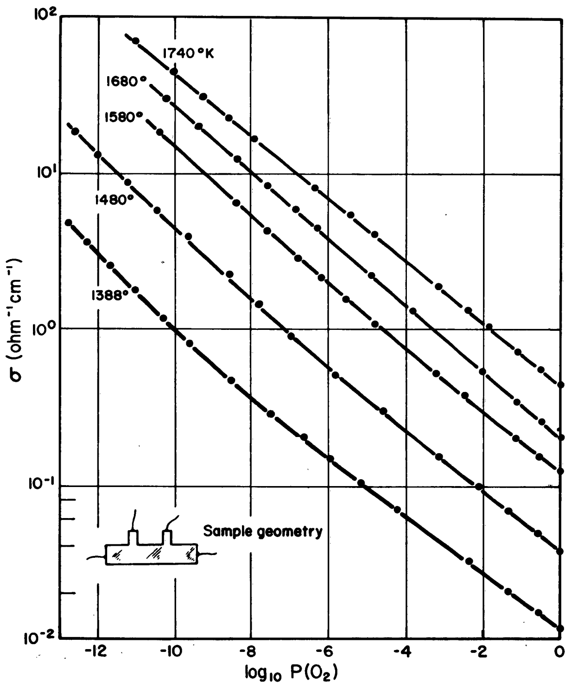
Fig. 9.10. Conductivity isotherms for \text{TiO}_2 as a function of partial pressure of oxygen (in atmospheres).
