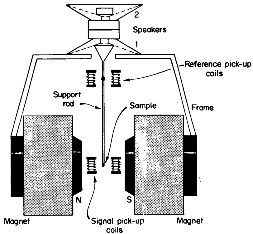
Fig. 10.2 - Basic mechanical features of vibrating sample magnetometer
