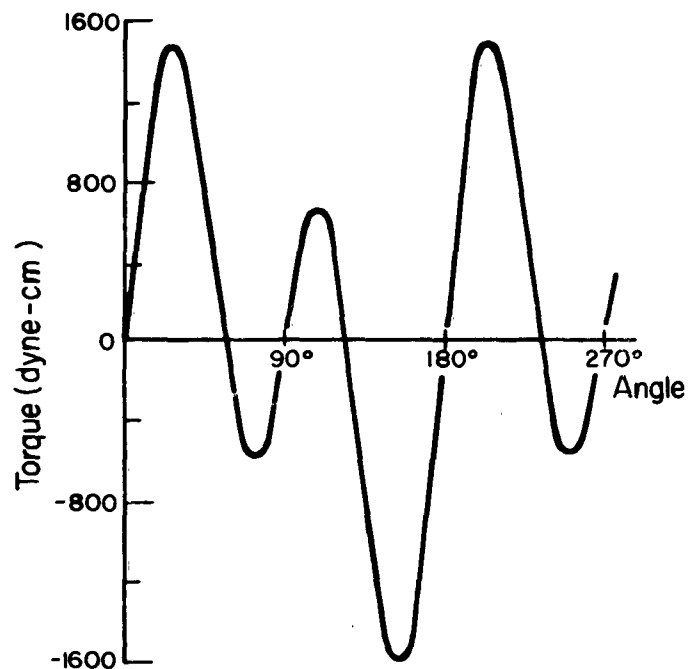
Fig. 10. 6. Torque vs. angle from [100] direction for a nickel crystal in the (110) plane at 20°C.
