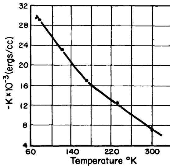
Fig. 10. 7. First order anisotropy constant of YIG.
