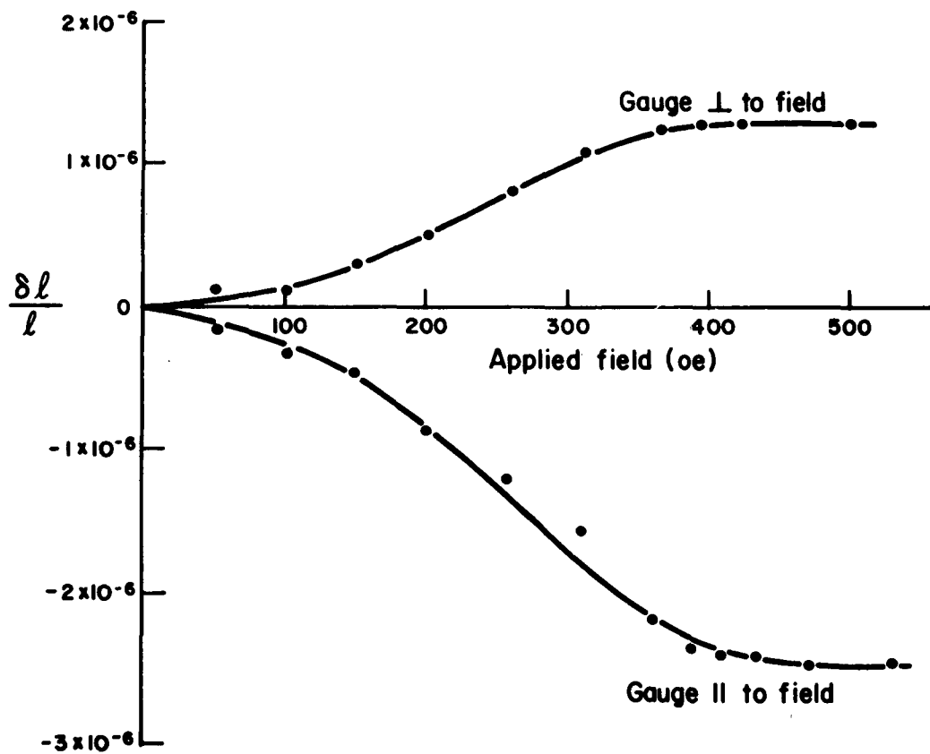
Fig. 8.3. Magnetostriction measurements on polycrystalline YIG disk at 25^{\circ}\text{C} .
