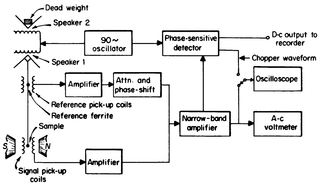
Fig. 10.1 - Block diagram of vibrating sample magnetometer
