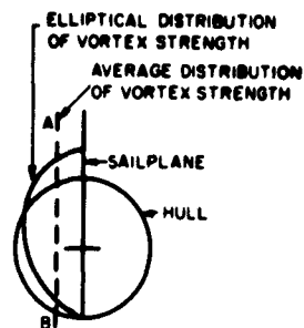
Figure 4a - Hull-Sailplane Vortex Distribution
