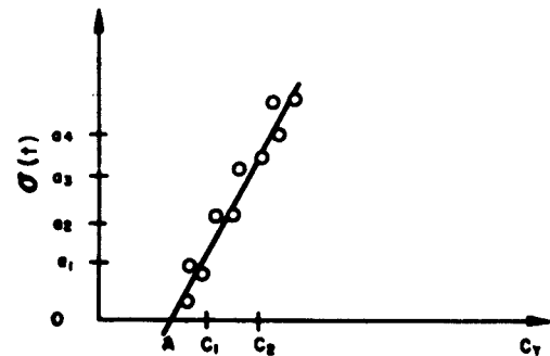
Figure 8 - Intensity of Shear Load versus Mean Lateral Force
