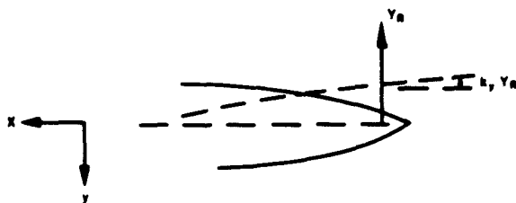
Figure 3a - Rudder Rotation Associated with Force Y_R
