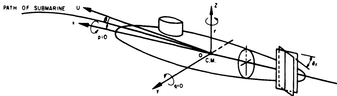
Figure 1a - Coordinate System
