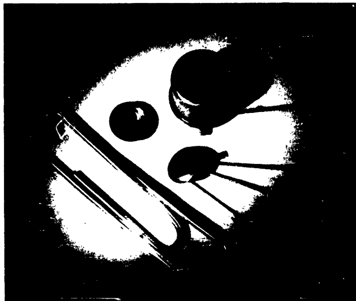
Figure 6-9. TO-46 Header and Cap of Task 18-6 (Magnification 5x) Adjacent to a 1 1/4 inch Paper Clip (Standard TO-5 Transistor also shown)
