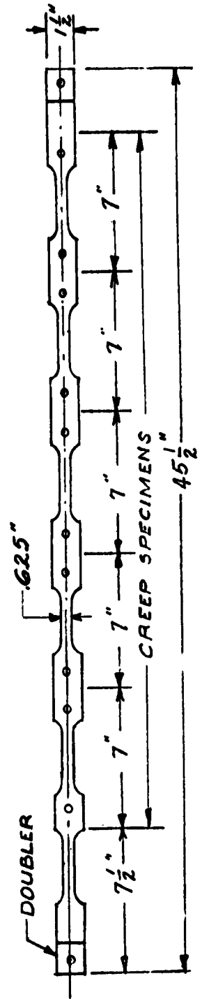
TANDEM CREEP SPECIMENS FOR MEASURING CREEP STRAIN DURING AND MECHANICAL PROPERTIES AFTER CREEP EXPOSURE
