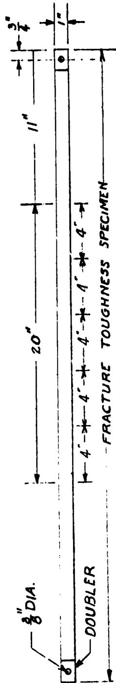
TANDEM CREEP SPECIMENS FOR MEASURING FRACTURE TOUGHNESS AFTER CREEP EXPOSURE
