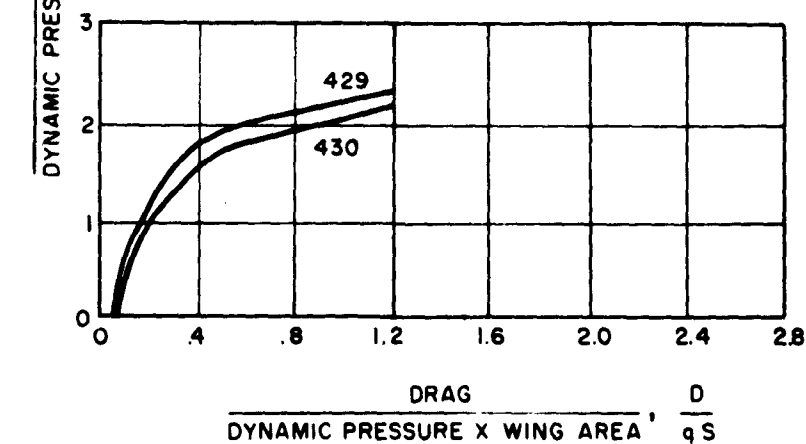
Figure 118. Configurations No. 55, \theta_F = -\theta_R = +60^\circ h/c = .33 , (Runs 429 - 430)
