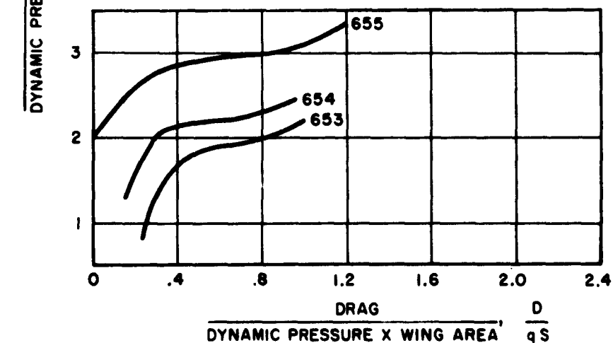
Figure 156. Configuration No. 46, \theta_F = -30^\circ , \theta_R = +30^\circ , h/c = .33 , (Runs 653-655)
