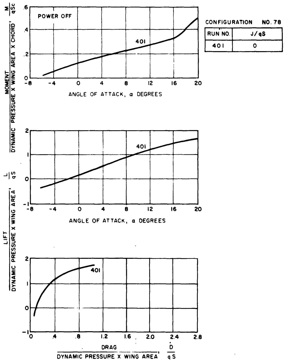
Figure 123. Configuration No. 78, \theta_F = -\theta_R = -h/c = .33 , (Run 401)
