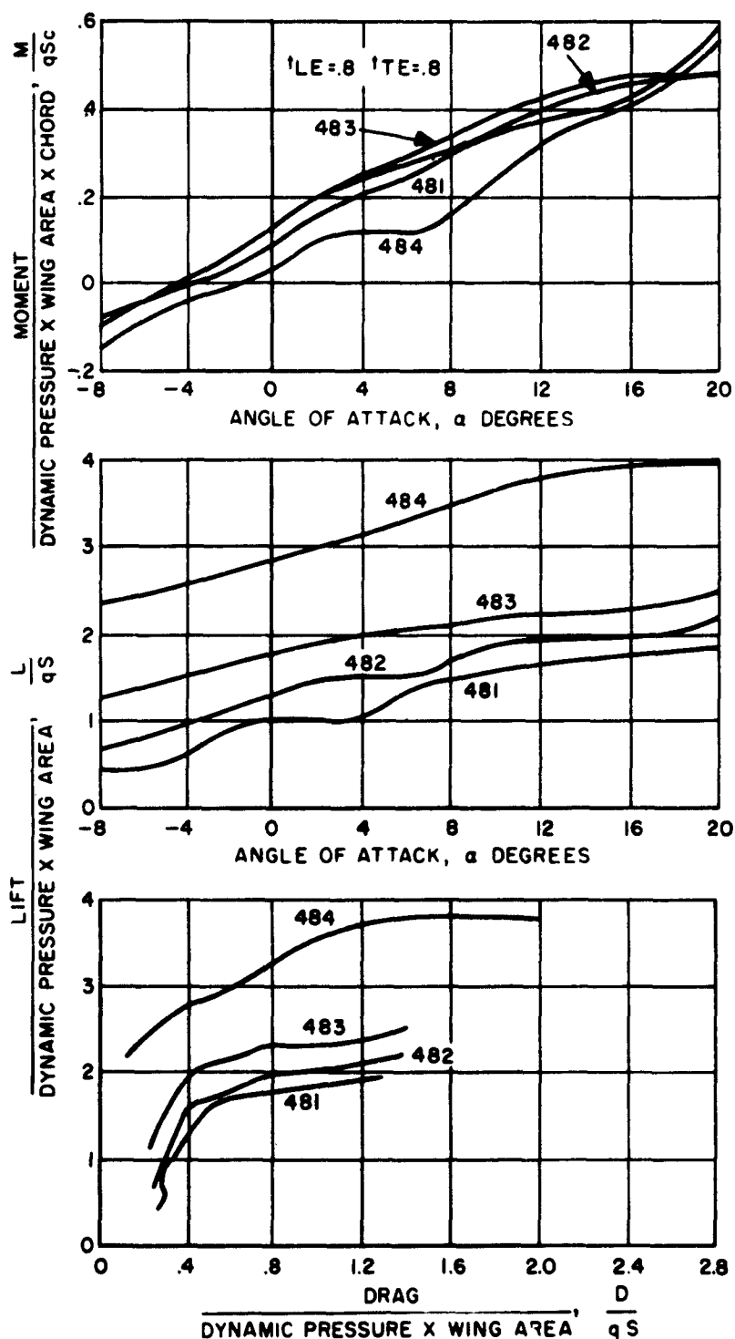
Figure 133. Configuration No. 28, \theta_F = -30^\circ , \theta_R = -30^\circ , h/c = .33 , (Runs 481 - 484)
