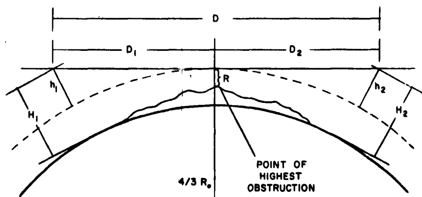
Figure 3-15. Line-of-sight path over curved earth including atmospheric refraction and first fresnal zone of radius R
