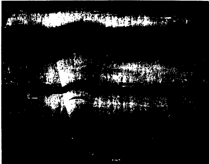
Figure 3. Pyrolytic Graphite Microstructure 14% CH 4 , 2000°C, Specimen 7-2 (45X).
