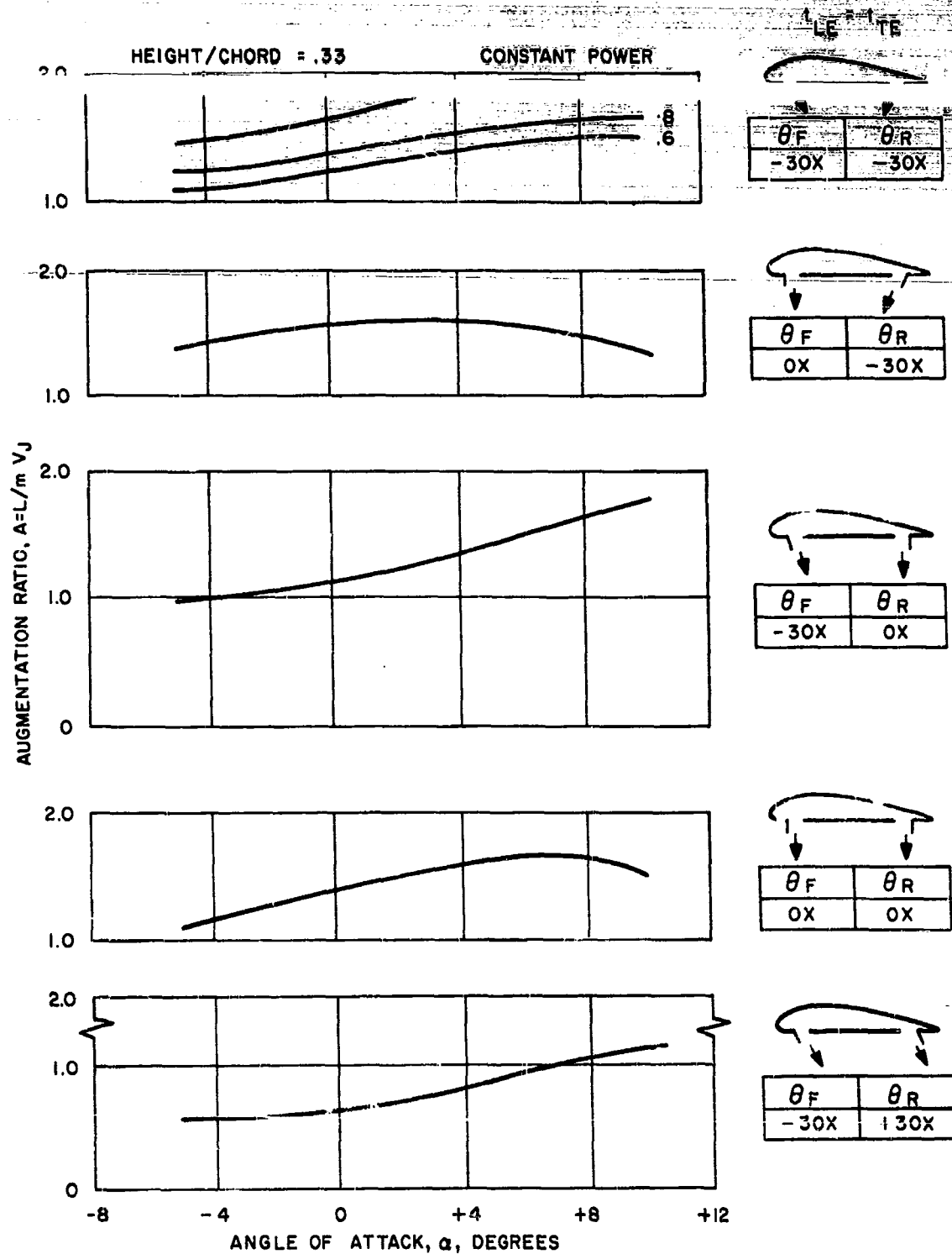
Figure 77. Variation of Augmentation Ratio with Angle of Attack for Various Slot Angle Configurations
