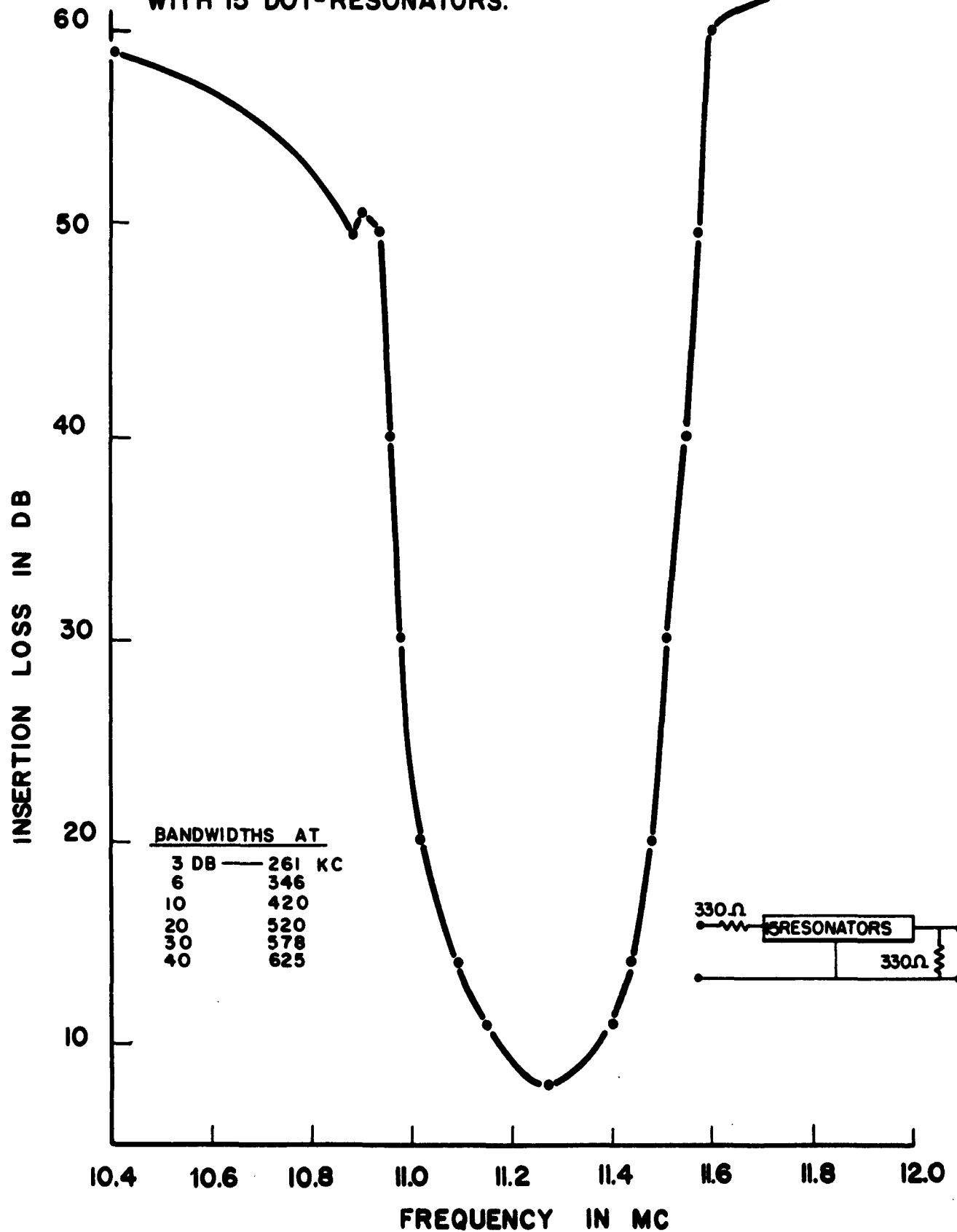
FIGURE 4. CERAMIC UNI-WAFER LADDER FILTER WITH 15 DOT-RESONATORS.
