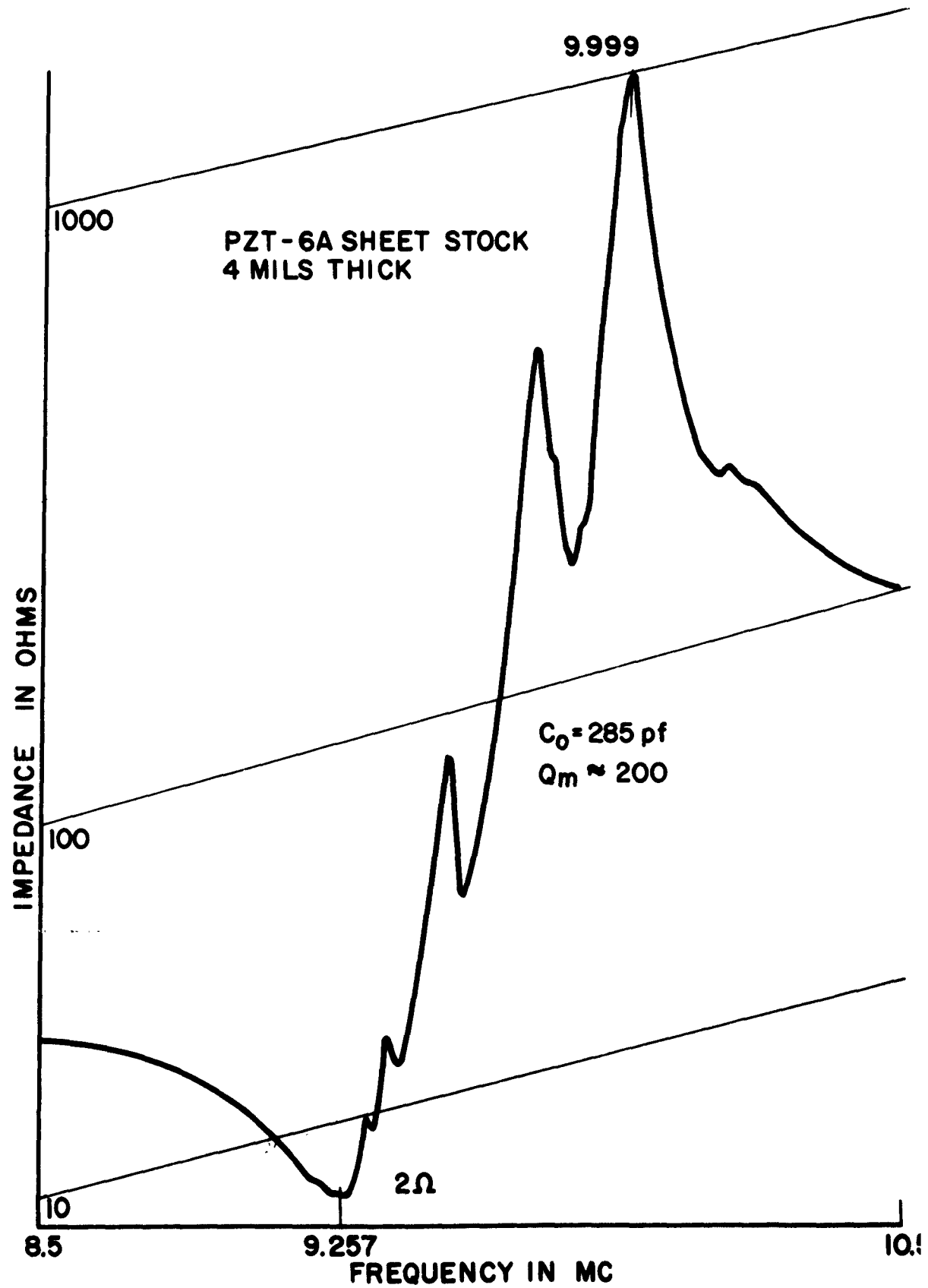
FIGURE 2 . CERAMIC FUNDAMENTAL THICKNESS SHEAR RESONATOR.
