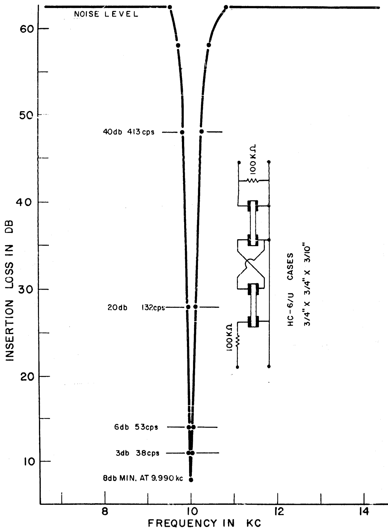
FIGURE I-2. CASCADED PAIR XT LF-S CERAMIC FILTERS.
