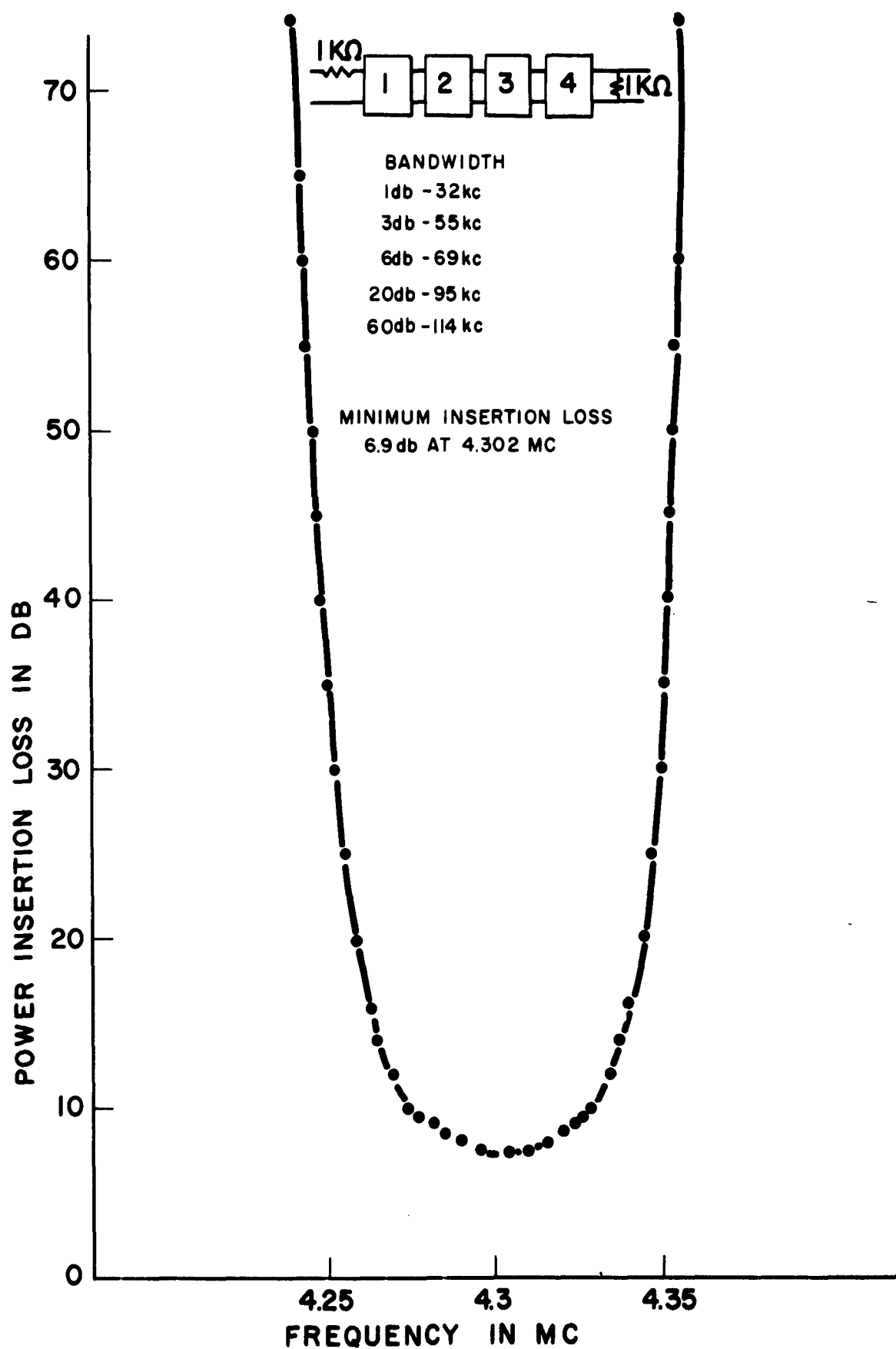
FIGURE I-5.4.3 MC MEDIUM BANDWIDTH LADDER FILTER.
