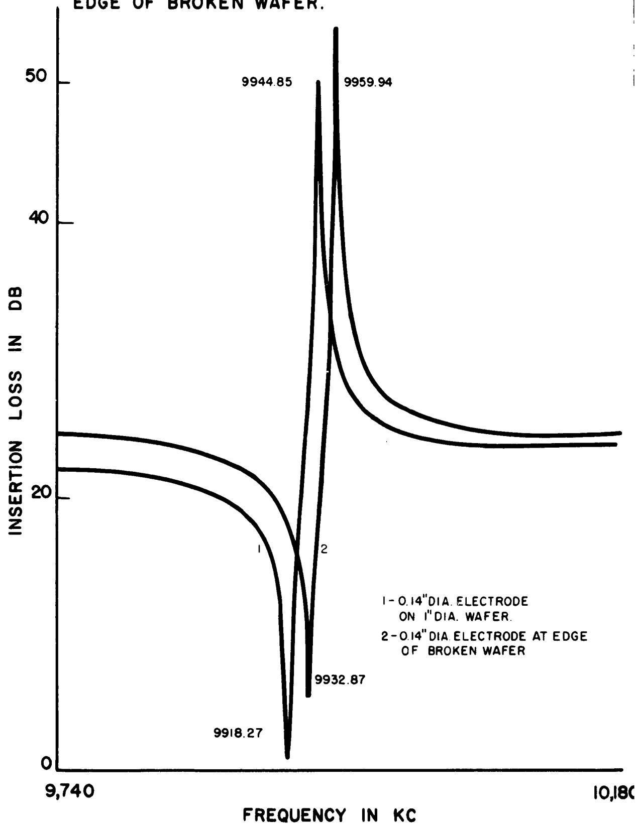
FIGURE 5 . RESPONSE OF AT-CUT QUARTZ RESONATOR AT EDGE OF BROKEN WAFER.
