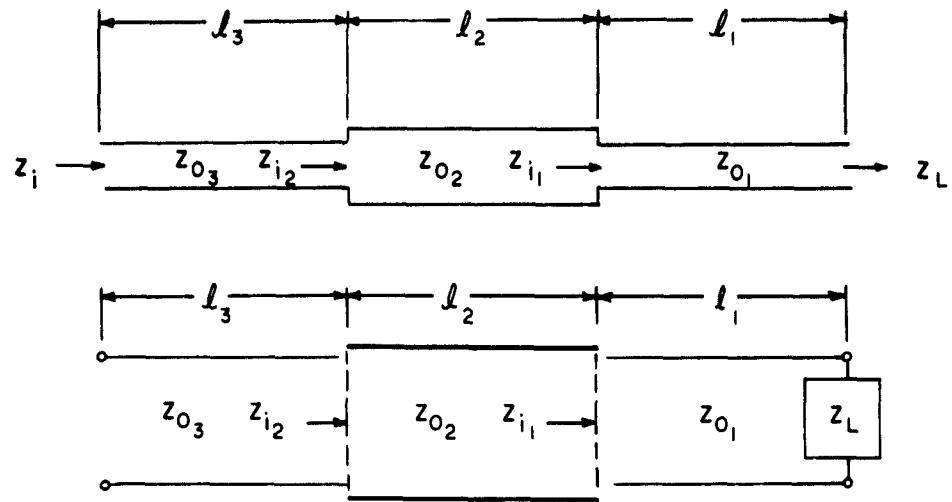
(a.) ACOUSTIC TRANSMISSION LINE WITH CHANGES IN z_0 AND ITS ACOUSTIC CIRCUIT REPRESENTATION
