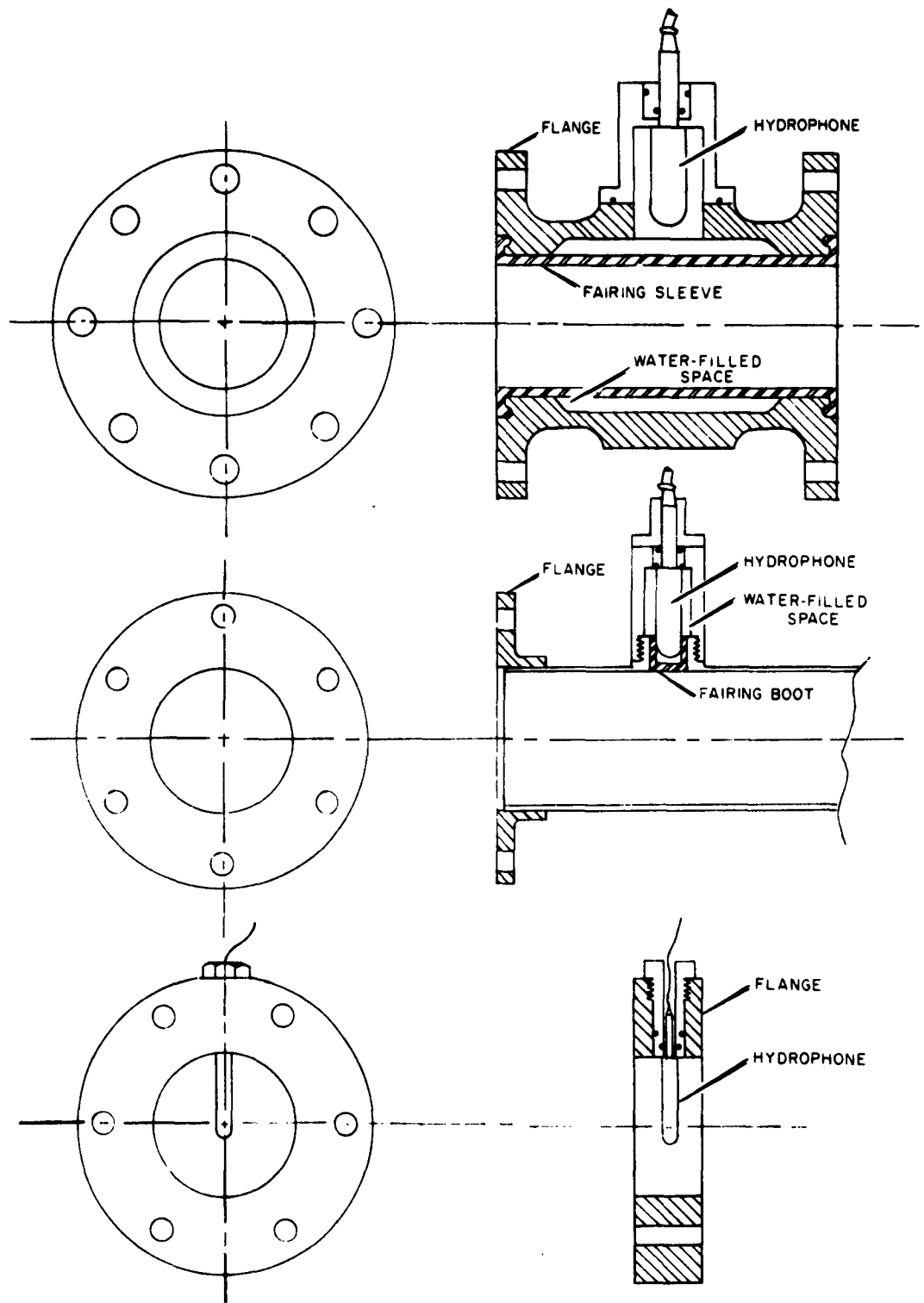
FIGURE 75 HYDROPHONE PORTS
