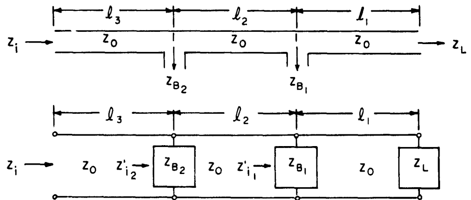
(b.) ACOUSTIC TRANSMISSION LINE WITH BRANCH IMPEDANCES AND ITS ACOUSTIC CIRCUIT REPRESENTATION
