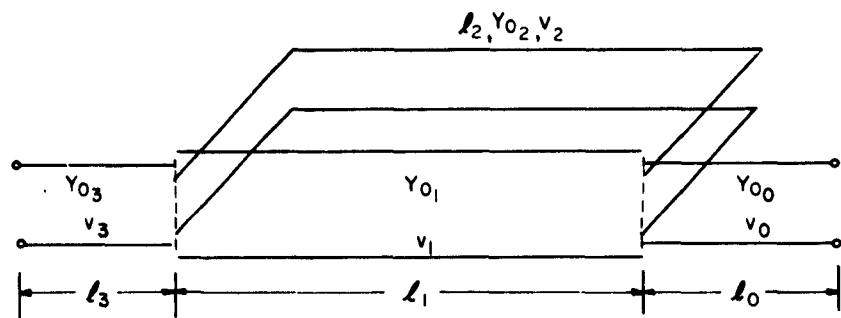
(b) TRANSMISSION LINE ACOUSTICAL CIRCUIT REPRESENTATION OF QUINCKE TUBE FILTER
