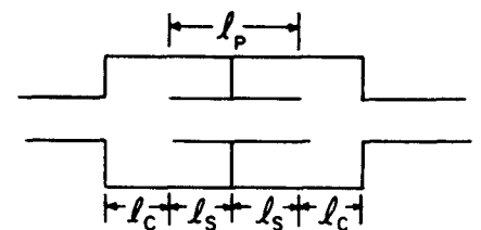
(d.) DOUBLE SECTION RE-ENTRANT CHAMBER
