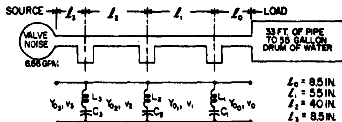
FIGURE 108 THREE ELEMENT SIDE-BRANCH FILTER WITH SPRING-PISTON BRANCH ELEMENTS
