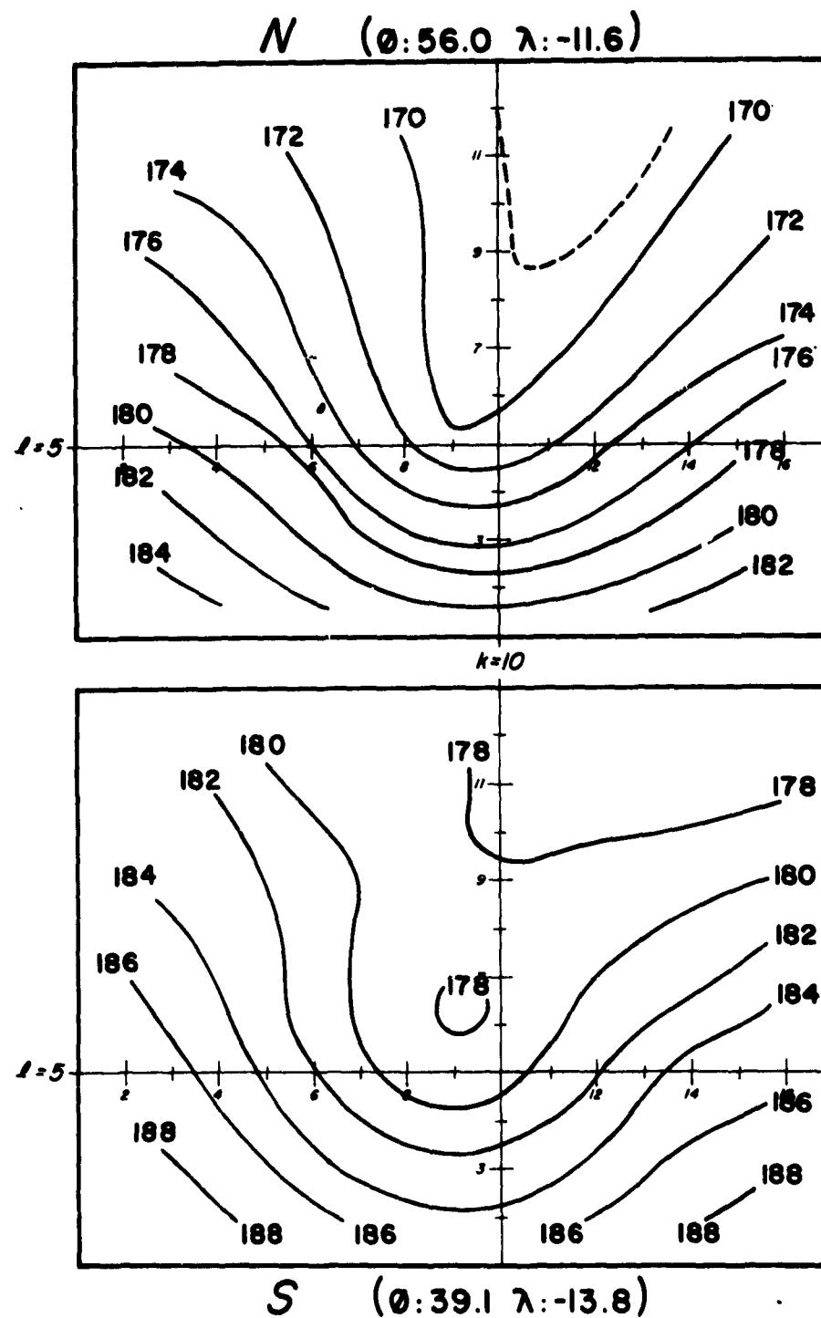
Fig. 3-4. Mean maps of 500-mb height for winter cyclones in Europe, 1955-1959 (dependent sample). Isohypsers are labeled in tens of feet.
