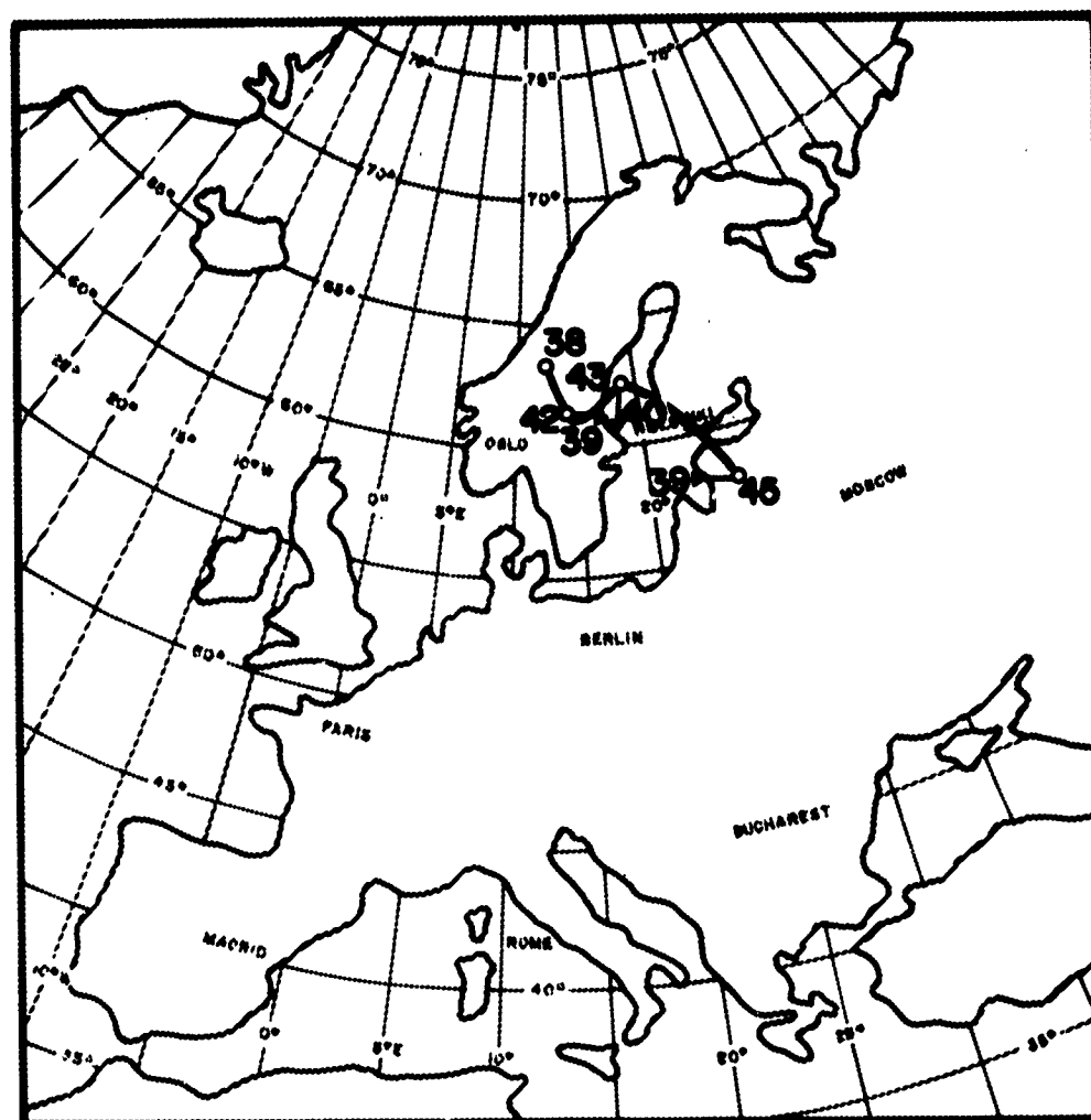
Fig. 4-5(b). Forecast verification. ○ Observed; △ unstratified prediction; □ stratified prediction; × surface predictors only.
