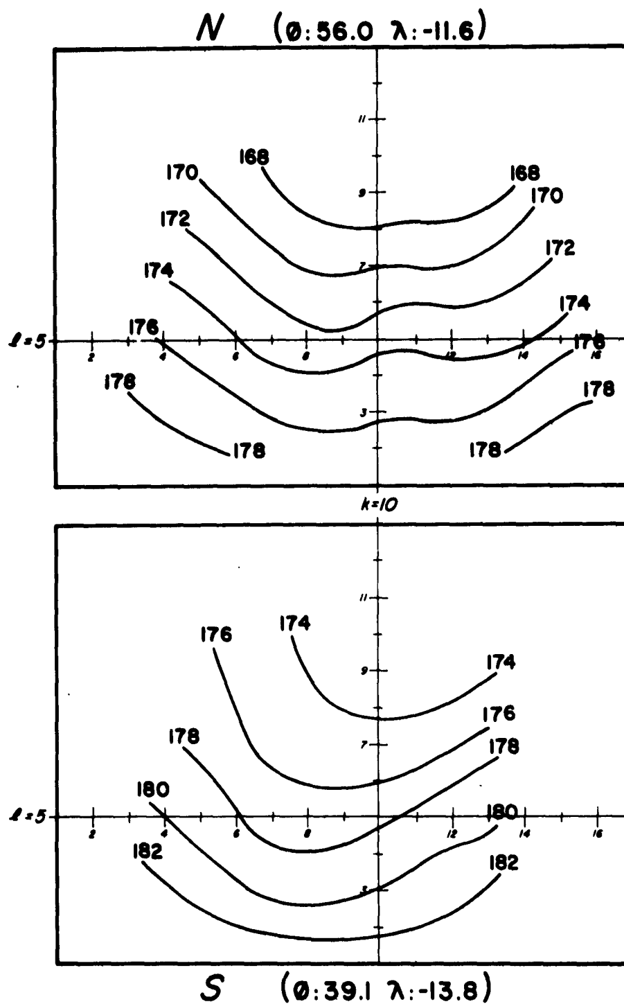
Fig. 3-6. Mean maps of 1000-500-mb thickness for winter cyclones in Europe, 1955-1959 (dependent sample). Isopachs are labeled in tens of feet.
