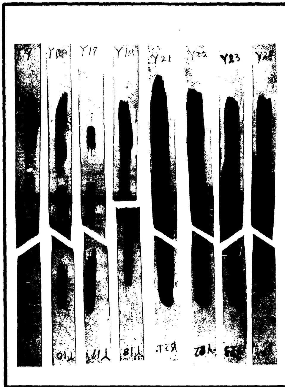
FIGURE 18 (continued) PHOTOGRAPH OF WELDED TENSILE SPECIMENS EXPOSED TO GASEOUS HYDROGEN ENVIRONMENT (.016, 6Al-4V ANNEALED TITANIUM, ROOM TEMPERATURE TEST)
