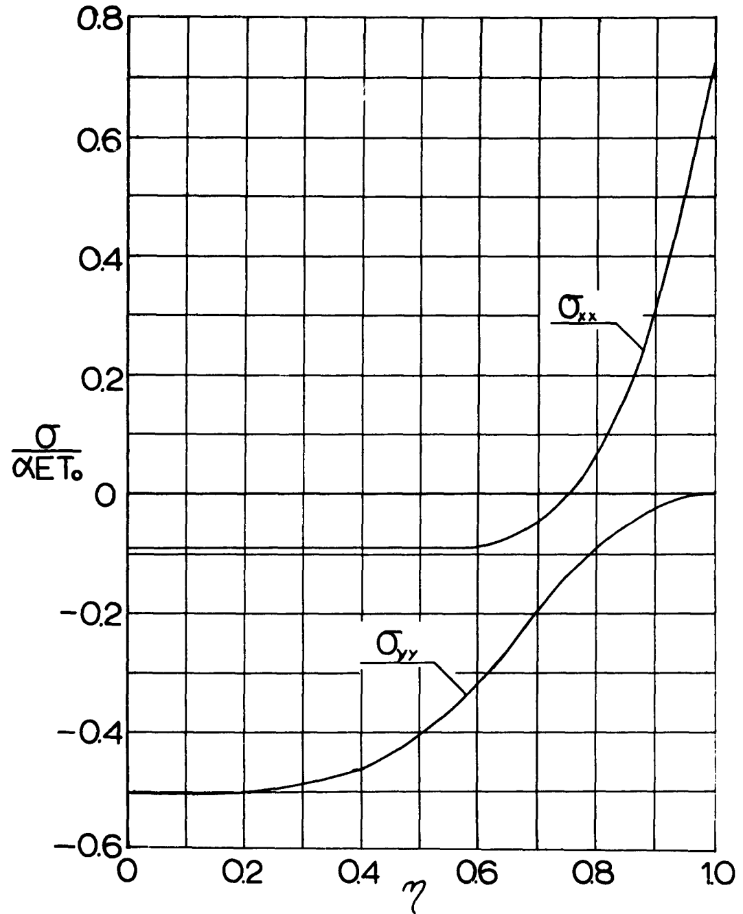
Figure 32: Calculated Stress Distribution Due to Approximating Temperature Distribution Along x = 0
