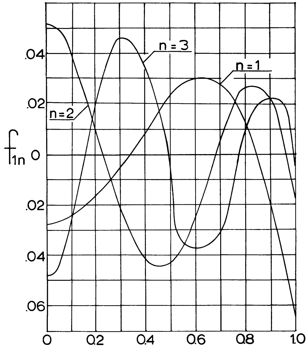
Figure 5: Graph of f_{1n}^{\eta}(\eta) vs \eta for n = 1, 2, 3
