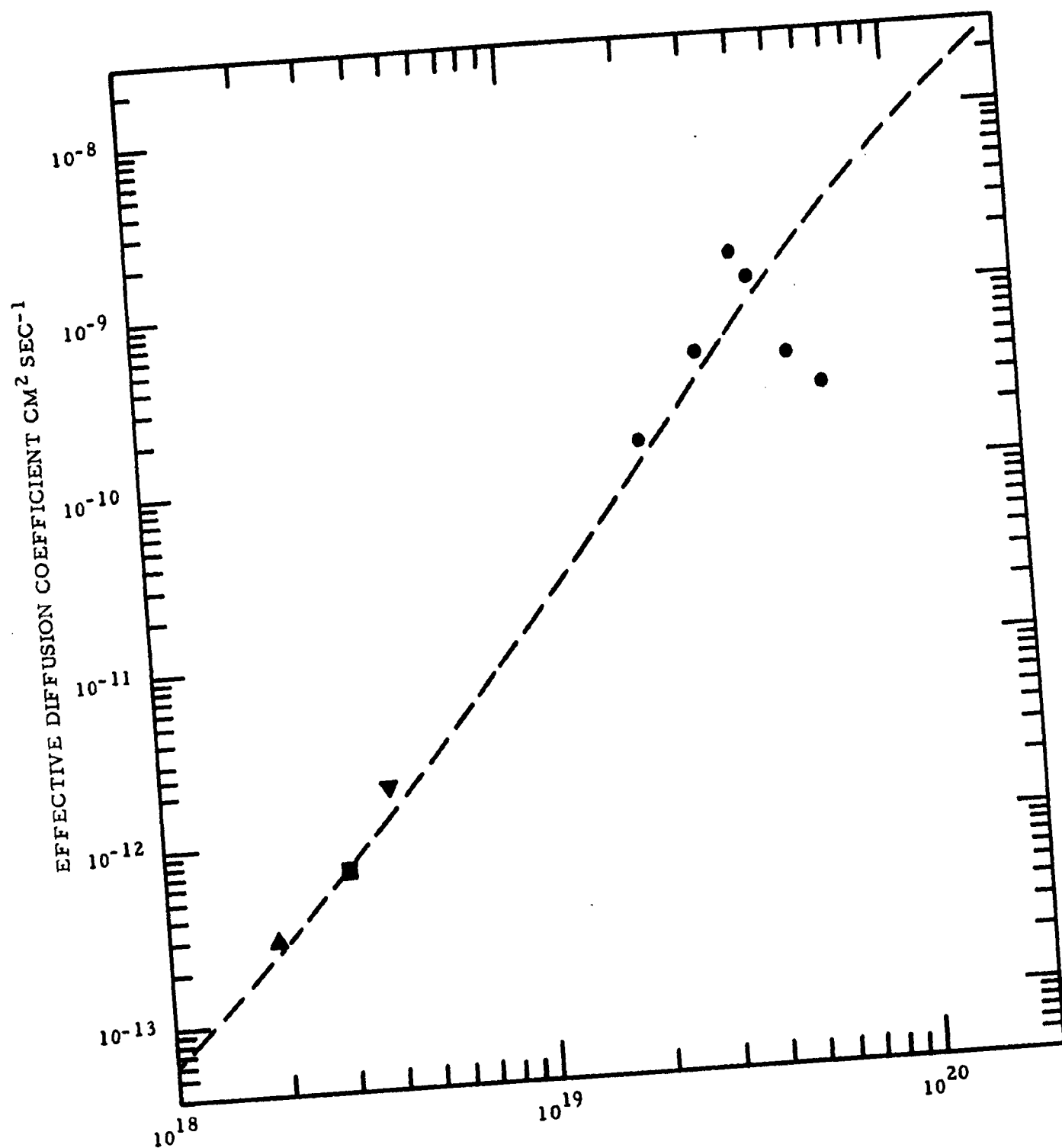
Fig. 18 Zinc diffusion in GaAs at 750°C
