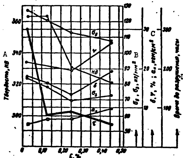
Fig. 18. Properties of EI787 alloy as functions of carbon content: heat treatment: 1180°, 4 hours, air + 1050°, 4 hours, air + 750°, 16 hours, air. Long-term-strength testing at [Key continued on next page]
