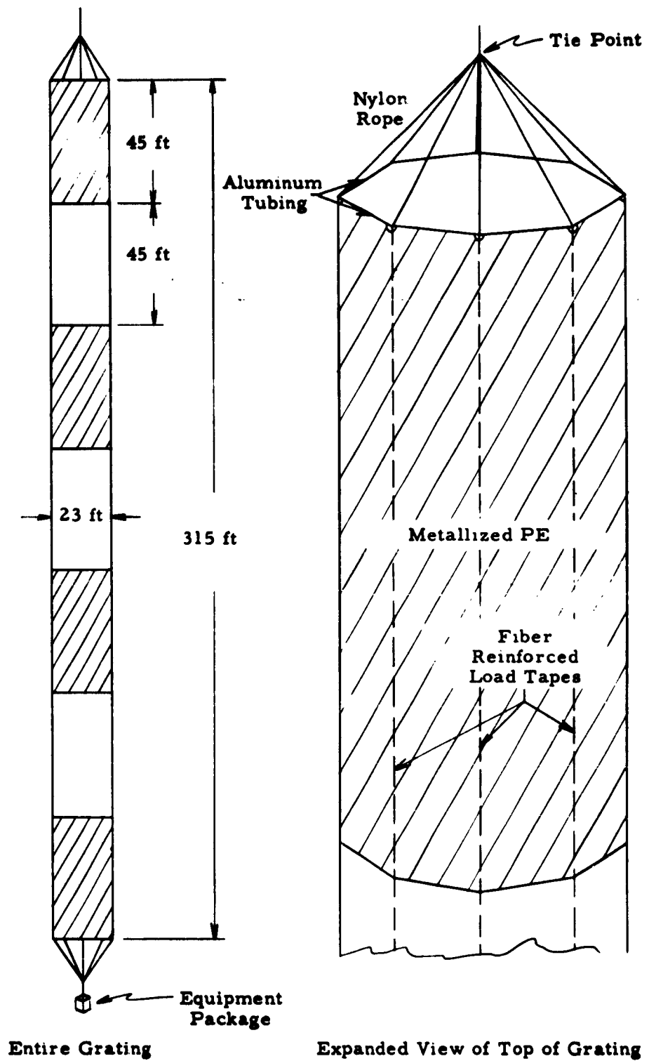
Figure 2-12. The Scatterloot Grated Array
