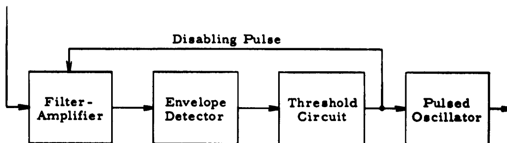
Figure 3-3. Transponder Diagram
