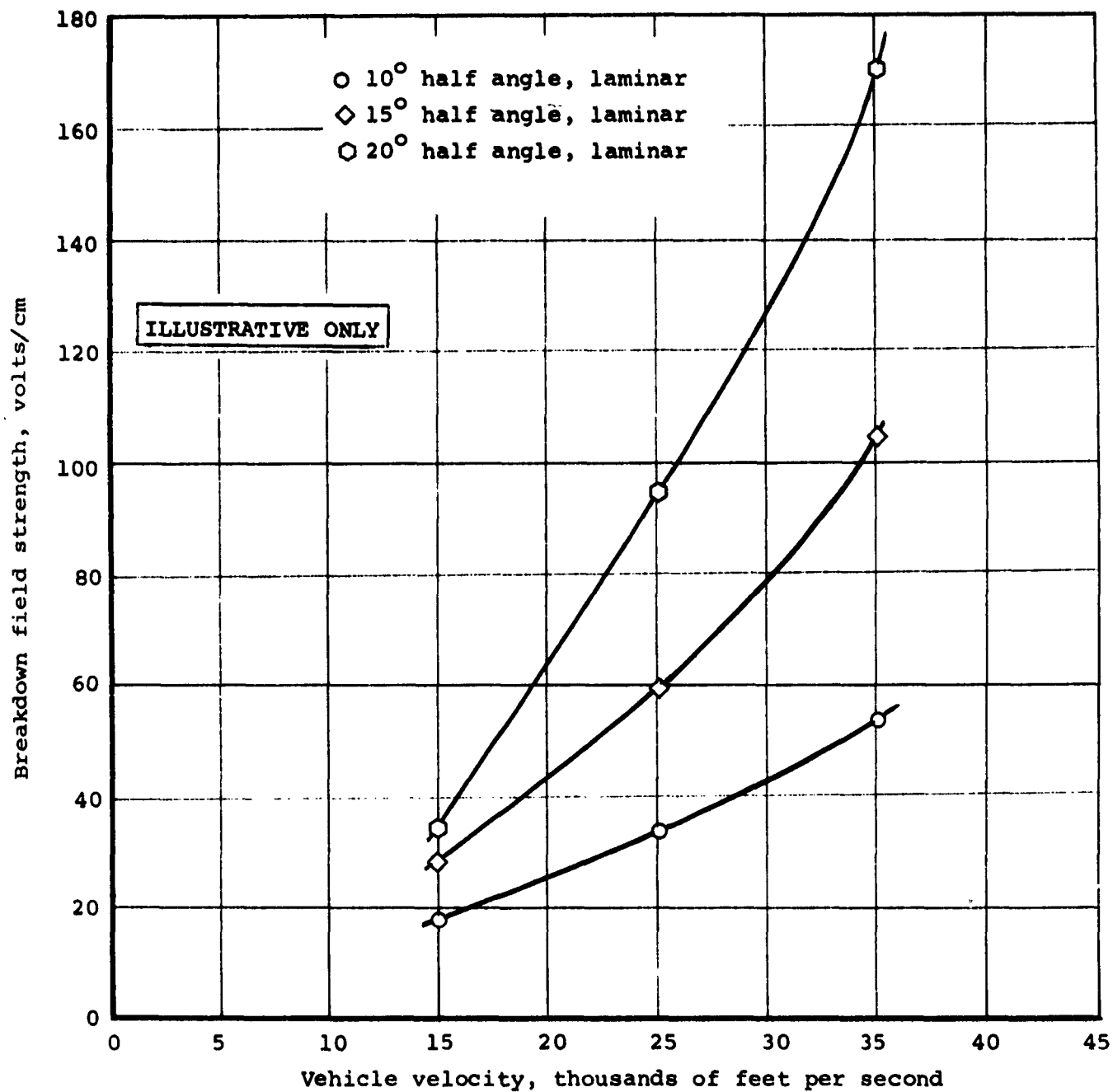
Figure 7.4.- Aperture breakdown field strength versus vehicle velocity for a wedge of 250,000-foot altitude at zero angle of attack. For purposes of illustration only. (Improper ionization frequency used. See Section 7.1.)
