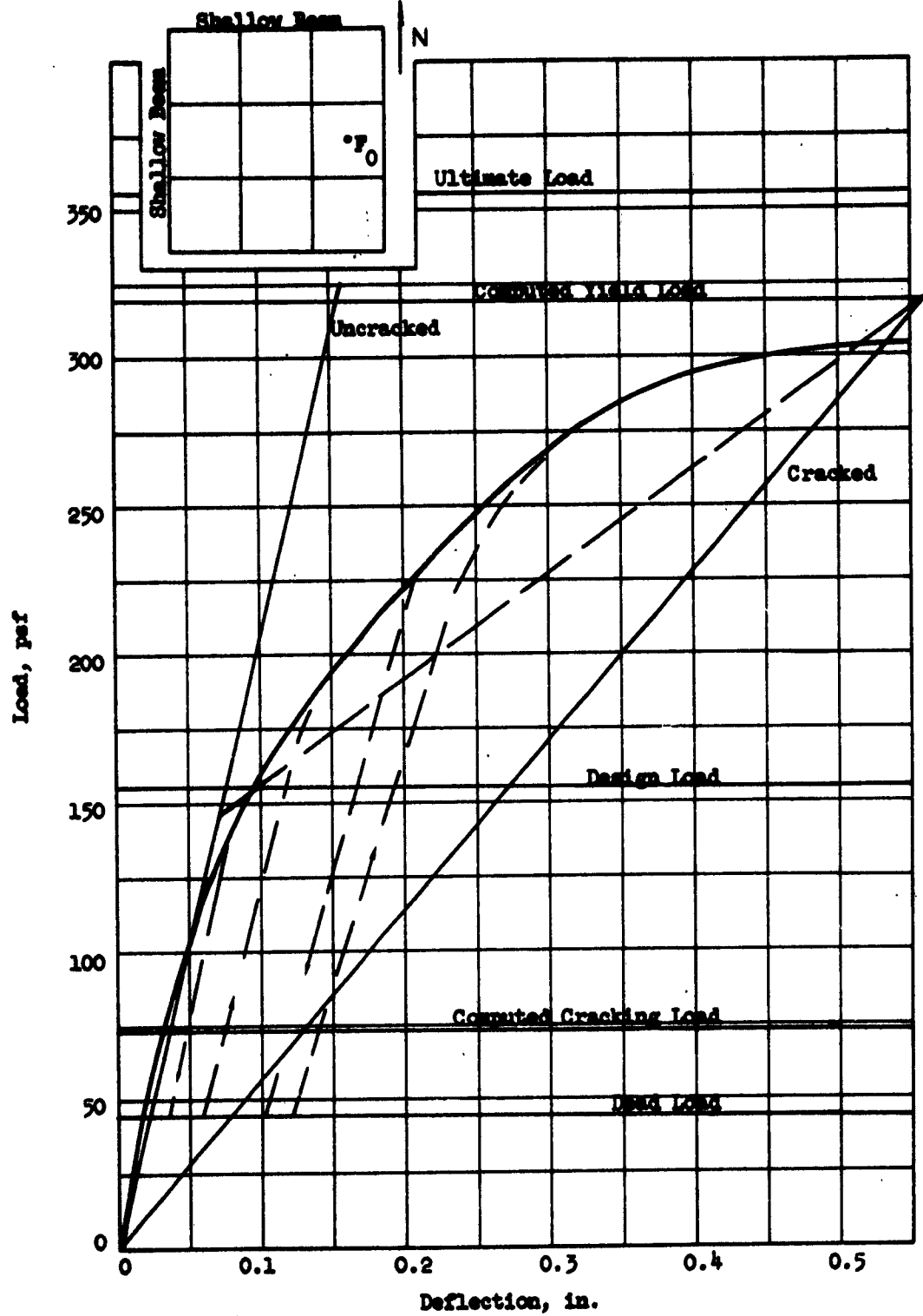
FIG. 5.47 LOAD-DEFLECTION CURVE, FLAT PLATE (F1), POINT F_0
