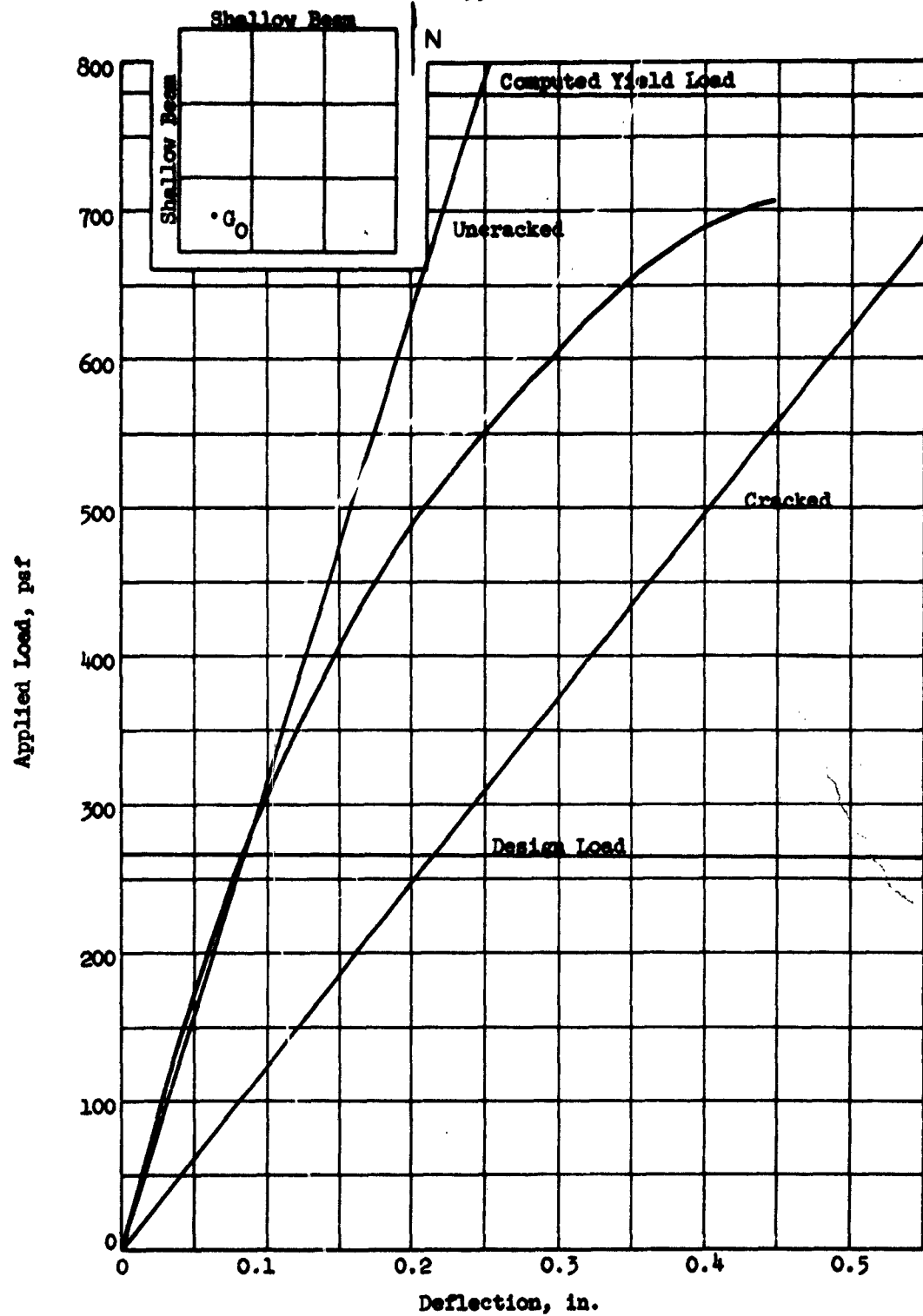
FIG. 5.36 LOAD-DEFLECTION CURVE, FLAT SLAB (F5), POINT G_0
