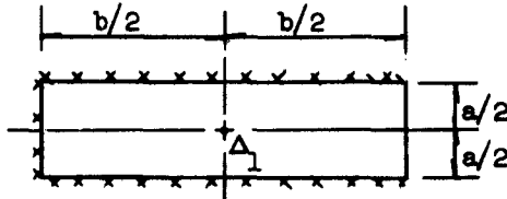
Case 4 One Edge Simply Supported, Three Edges Clamped
