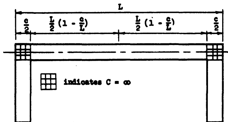
(a) BEAM-COLUMN COMBINATION
