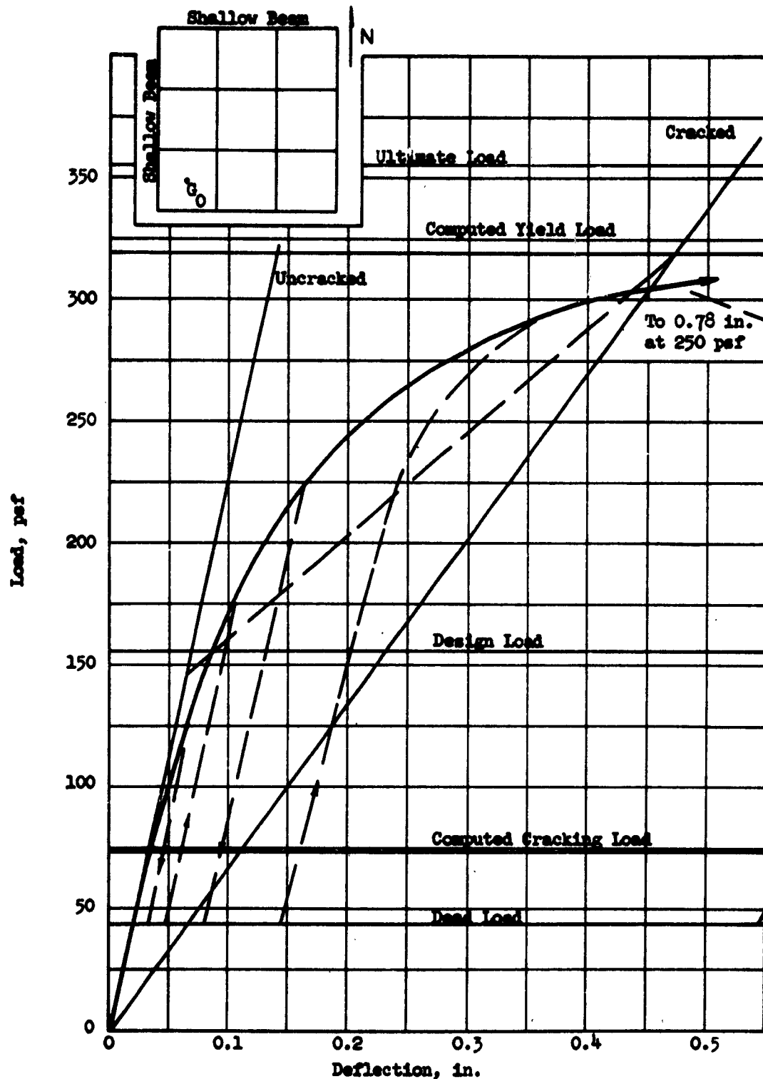
FIG. 5.51 LOAD-DEFLECTION CURVE, FLAT PLATE (F1), POINT G 0
