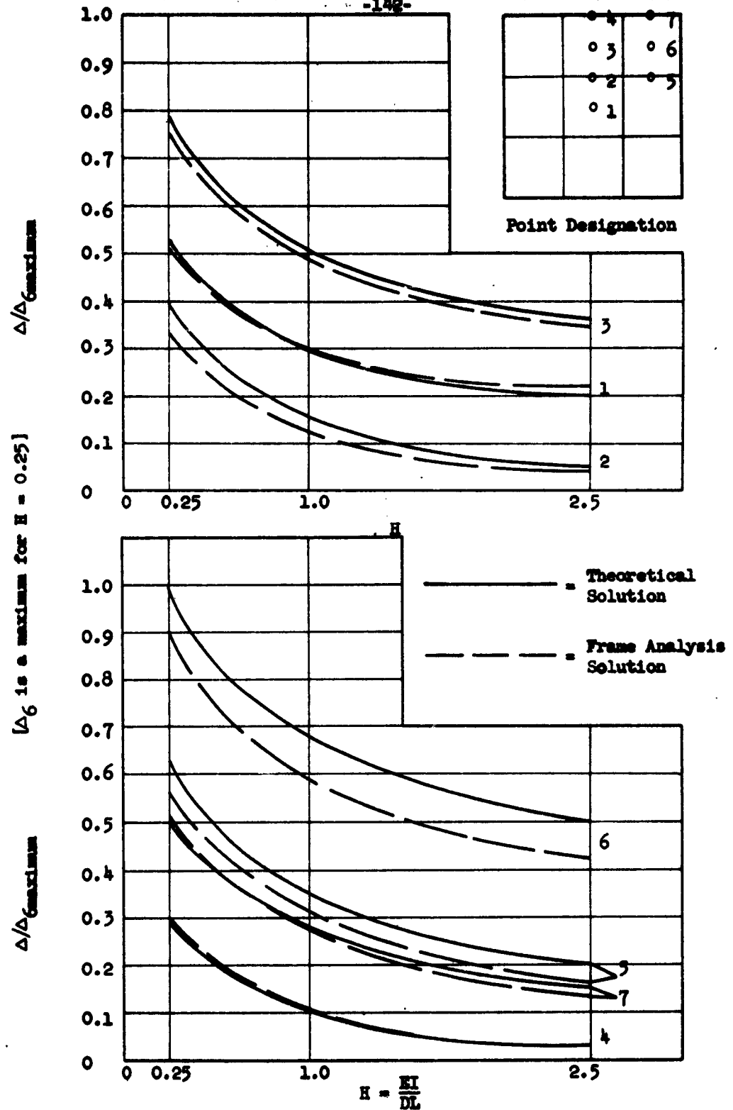
FIG. 4.8 COMPARISONS OF THEORETICAL AND FRAME ANALYSIS SOLUTIONS, J = 1.0 , K = 10 , ALL PANELS LOADED
