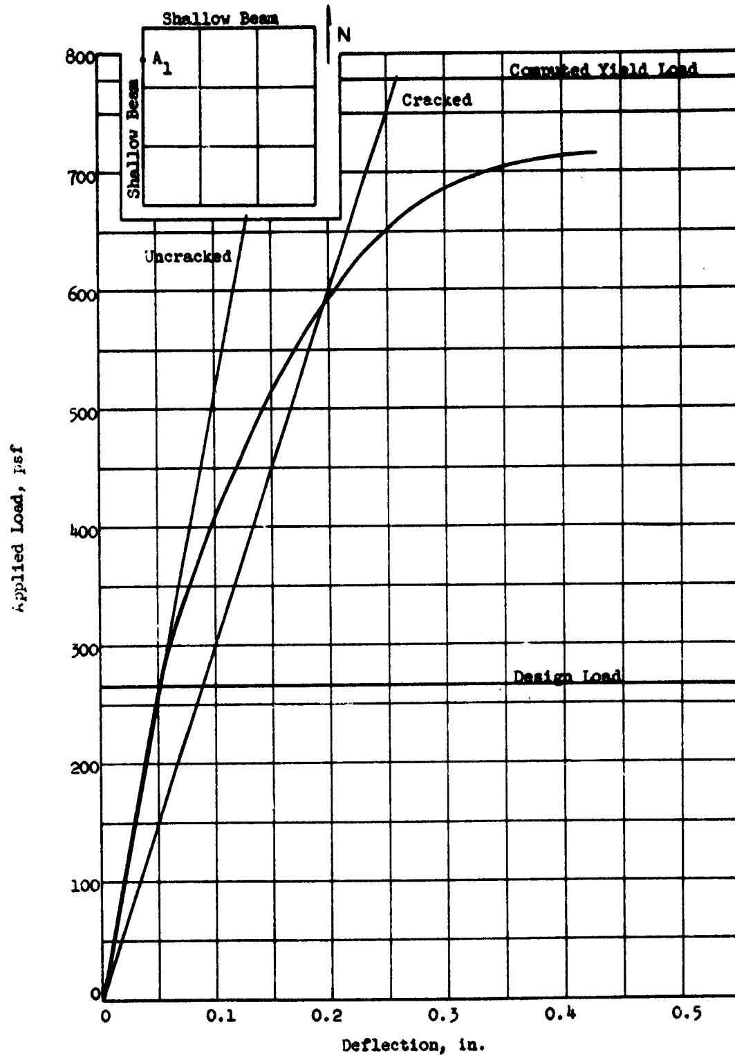
FIG. 5.33 LOAD-DEFLECTION CURVE, FLAT SLAB (F5), POINT A 1
