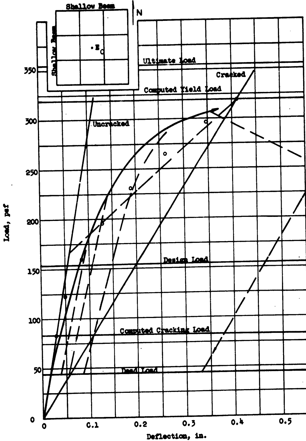
FIG. 5.45 LOAD-DEFLECTION CURVE, FLAT PLATE (F1), POINT E 0
