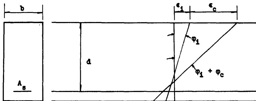
(b) Uncracked Section
