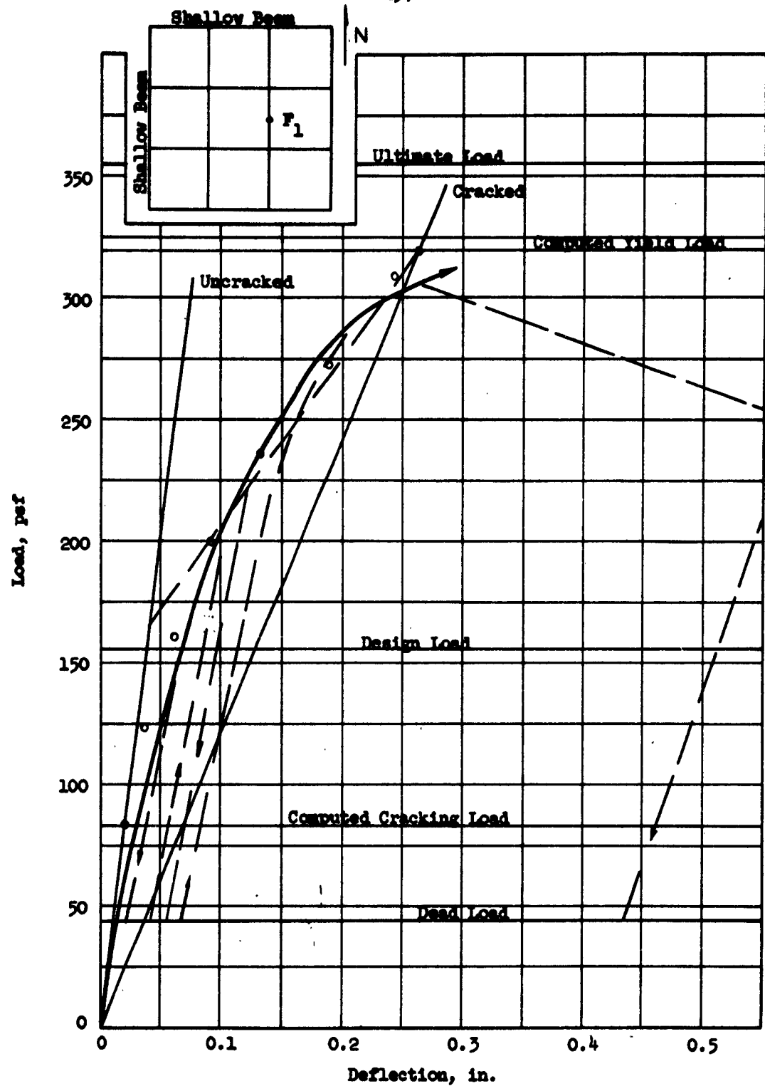
FIG. 5.48 LOAD-DEFLECTION CURVE, FLAT PLATE (F1), POINT F_1
