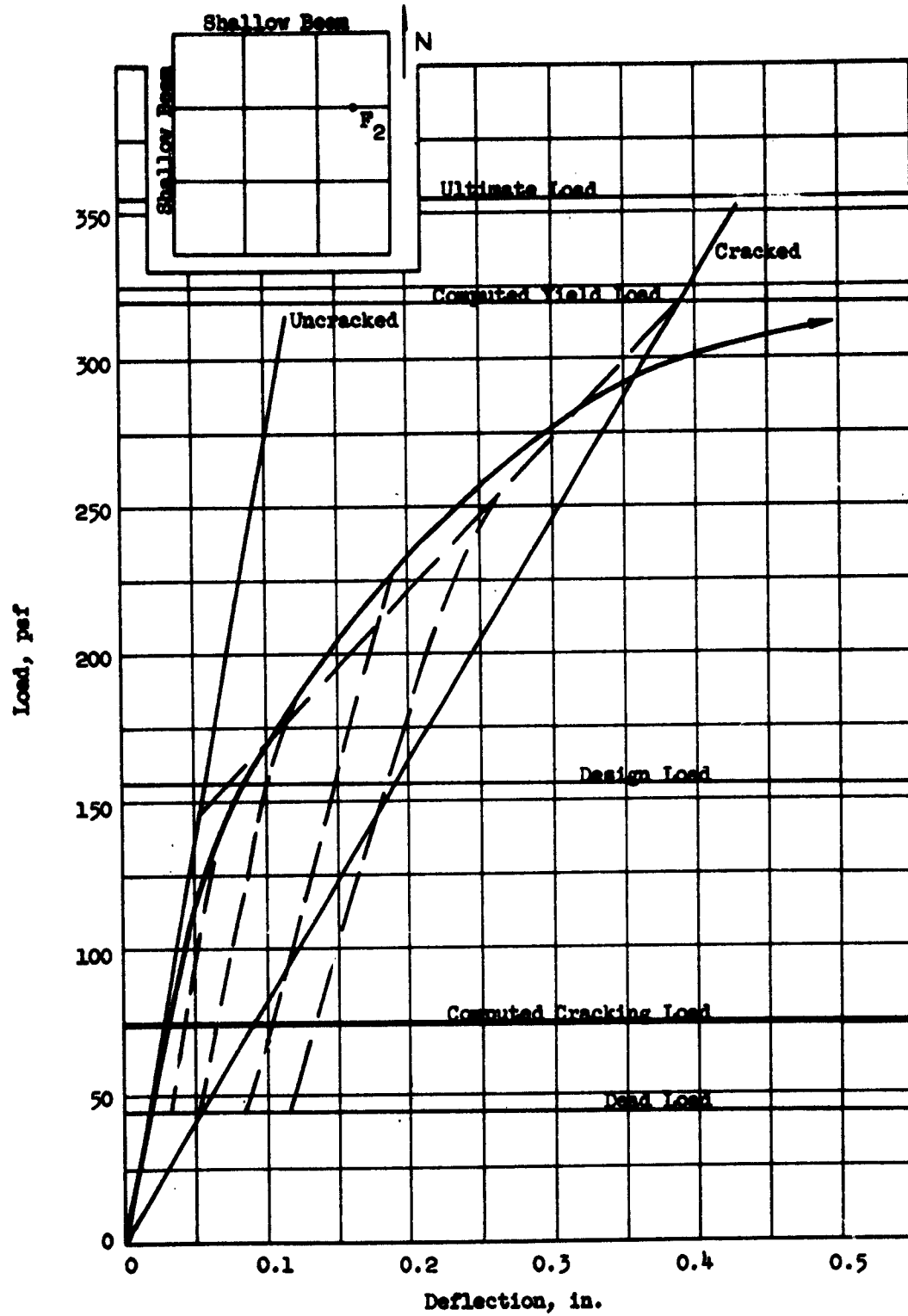
FIG. 5.49 LOAD-DEFLECTION CURVE, FLAT PLATE (F1), POINT F_2
