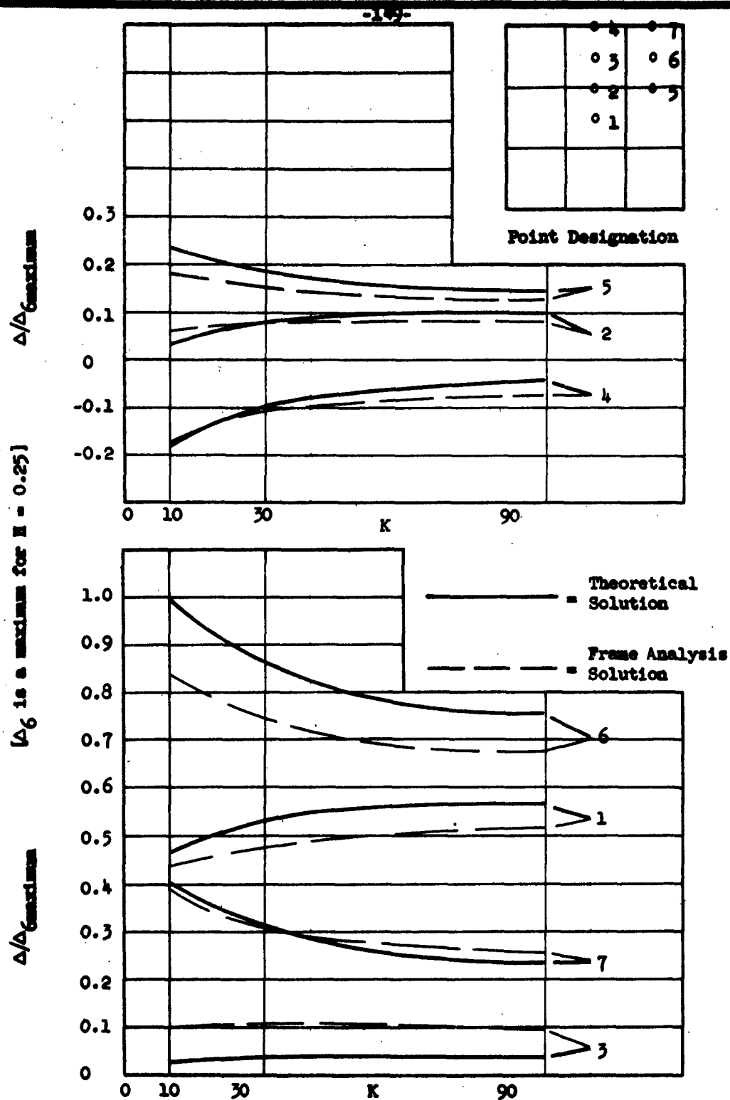
FIG. 4.15 COMPARISONS OF THEORETICAL AND FRAME ANALYSES SOLUTIONS, H = J = 2.5 , CORNER AND INTERIOR PANELS LOADED
