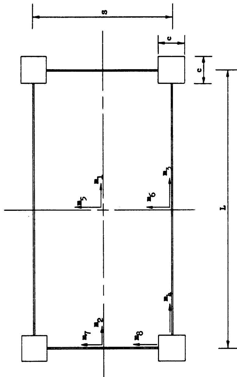
FIG. 3.6 DIRECTION AND DESIGNATION OF BENDING MOMENTS IN A TYPICAL INTERIOR PANEL
