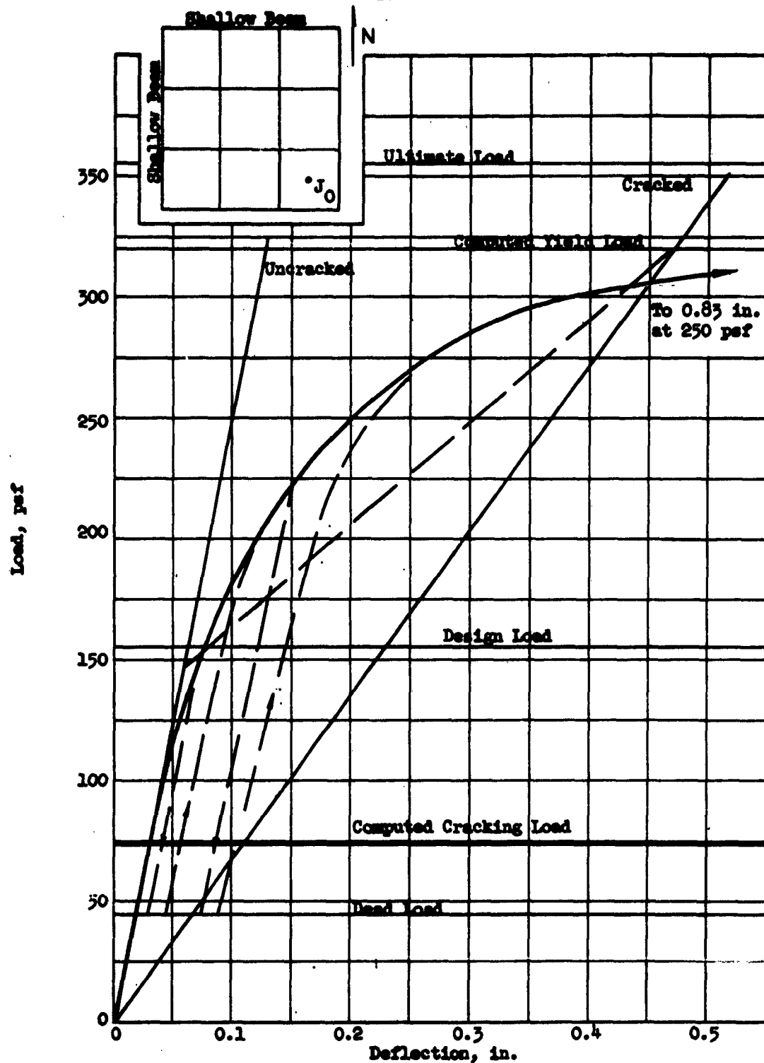
FIG. 5.52 LOAD-DEFLECTION CURVE, FLAT PLATE (F1), POINT J_0
