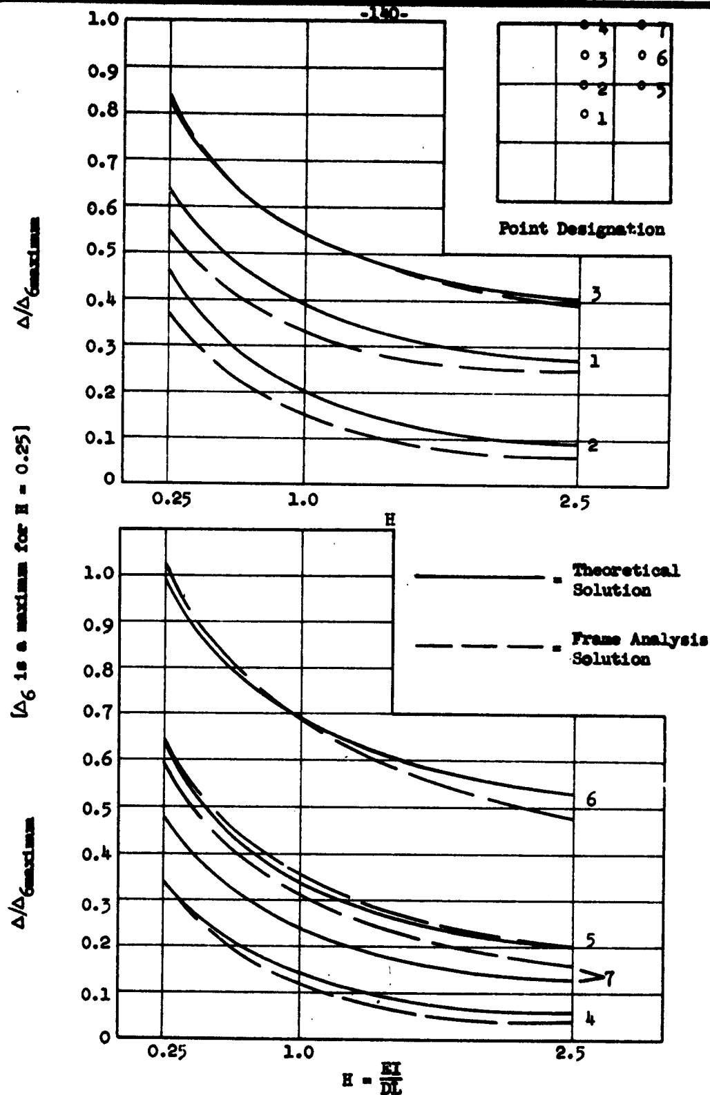
FIG. 4.6 COMPARISONS OF THEORETICAL AND FRAME ANALYSIS SOLUTIONS, J = 0.25 , K = 30 , ALL PANELS LOADED
