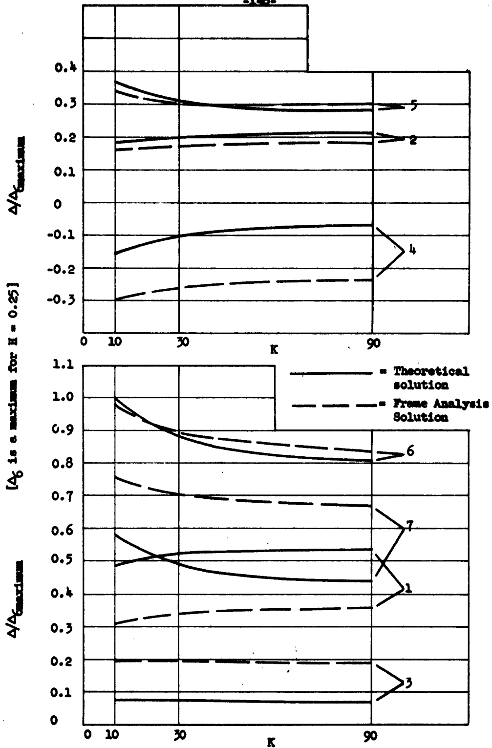
FIG. 4.14 COMPARISONS OF THEORETICAL AND FRAME ANALYSIS SOLUTIONS, H = J = 0.25 , CORNER AND INTERIOR PANELS LOADED
