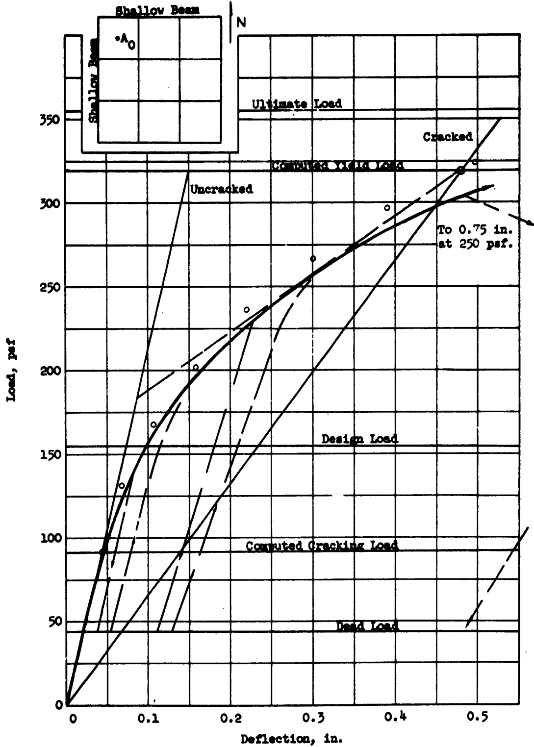
FIG. 5.39 LOAD-DEFLECTION CURVE, FLAT PLATE (F1), POINT A 0
