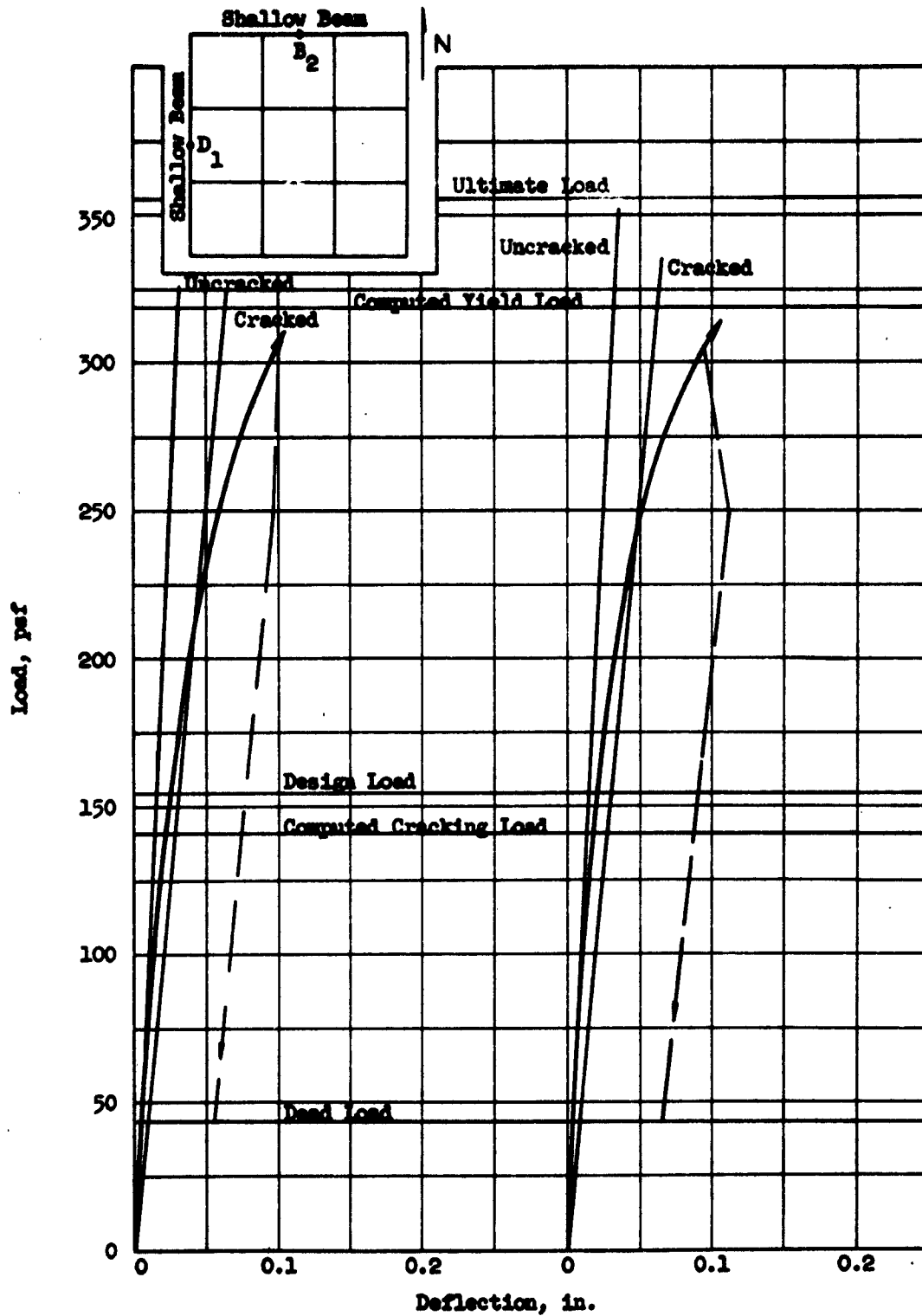
FIG. 5.43 LOAD-DEFLECTION CURVES, FLAT PLATE (F1), POINTS B_2 AND D_1
