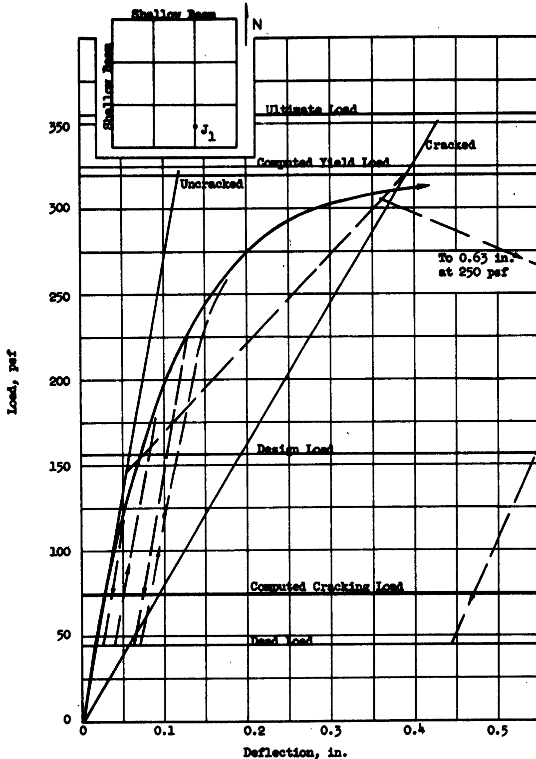
FIG. 5.53 LOAD-DEFLECTION CURVE, FLAT PLATE (F1), POINT J 1
