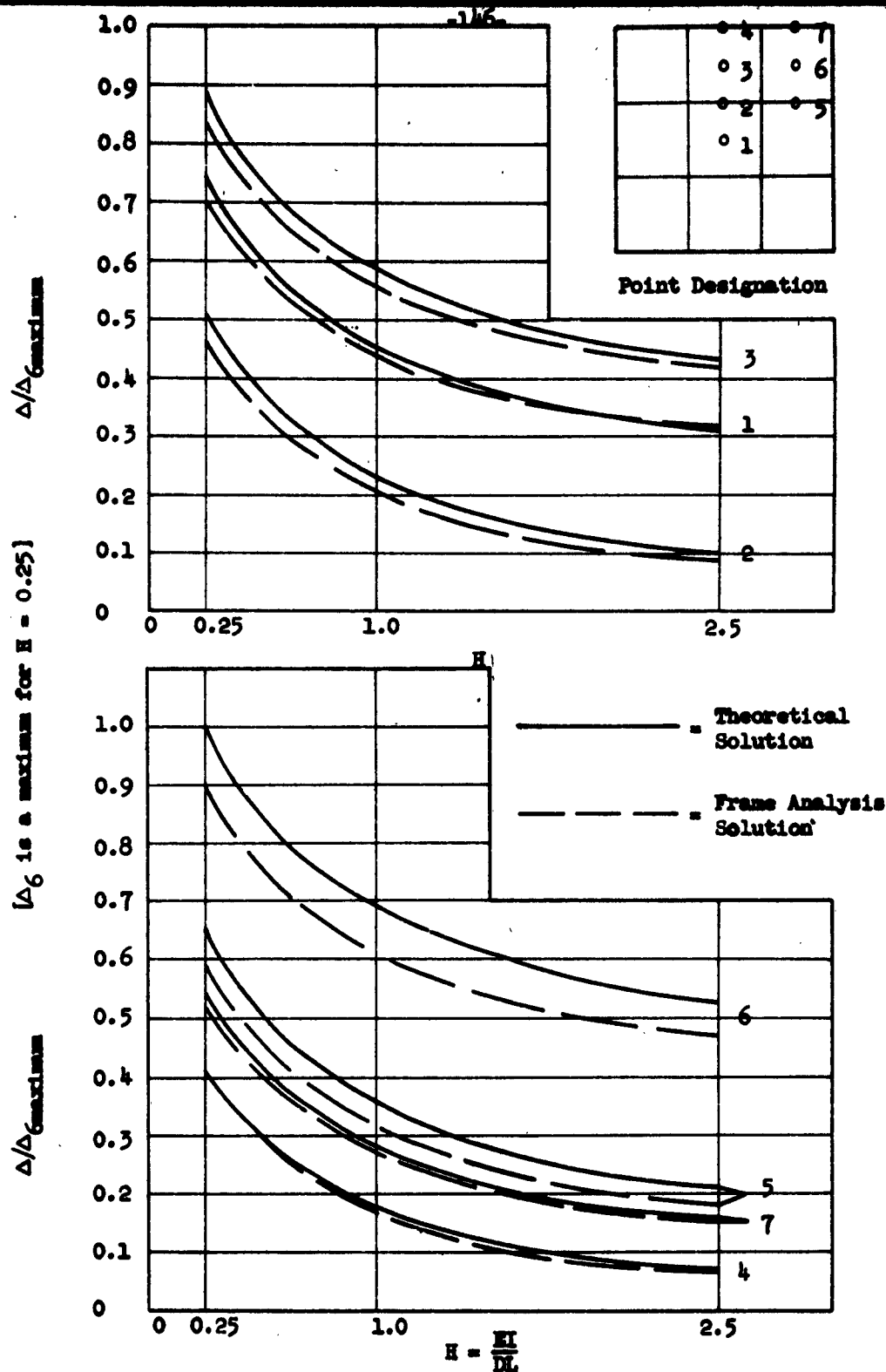
FIG. 4.12 COMPARISONS OF THEORETICAL AND FRAME ANALYSES SOLUTIONS, J = 2.5 , K = 30 , ALL PANELS LOADED
