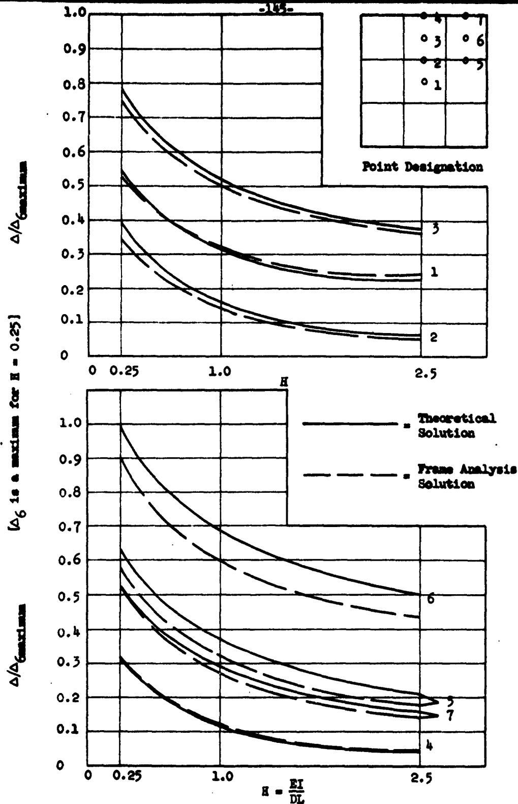
FIG. 4.11 COMPARISONS OF THEORETICAL AND FRAME ANALYSIS SOLUTIONS, J = 2.5 , K = 10 , ALL PANELS LOADED
