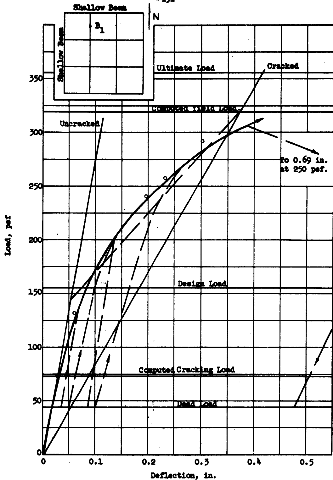
FIG. 5.42 LOAD-DEFLECTION CURVE, FLAT PLATE (F1), POINT B 1
