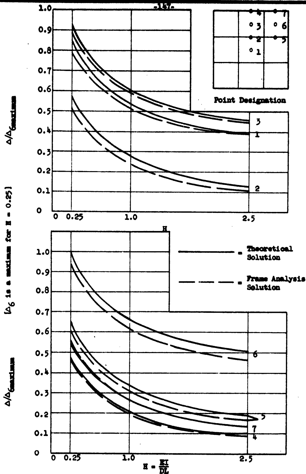
FIG. 4.13 COMPARISONS OF THEORETICAL AND FRAME ANALYSES SOLUTIONS, J = 2.5 , K = 90 , ALL PANELS LOADED
