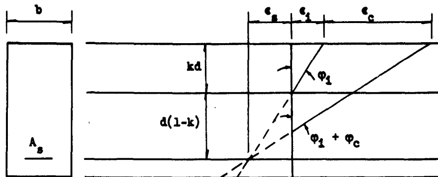
(a) Fully Cracked Section
