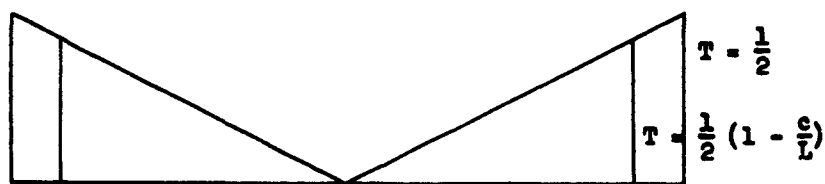
(c) TWISTING MOMENT DIAGRAM
