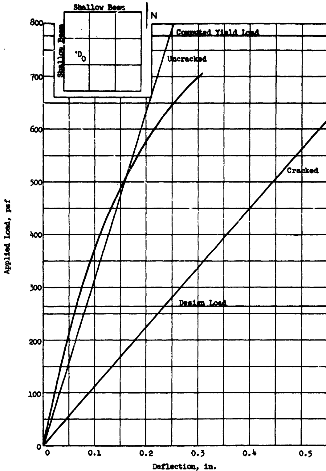
FIG. 5.85 LOAD-DEFLECTION CURVE, FLAT SLAB (F5), POINT D 0
