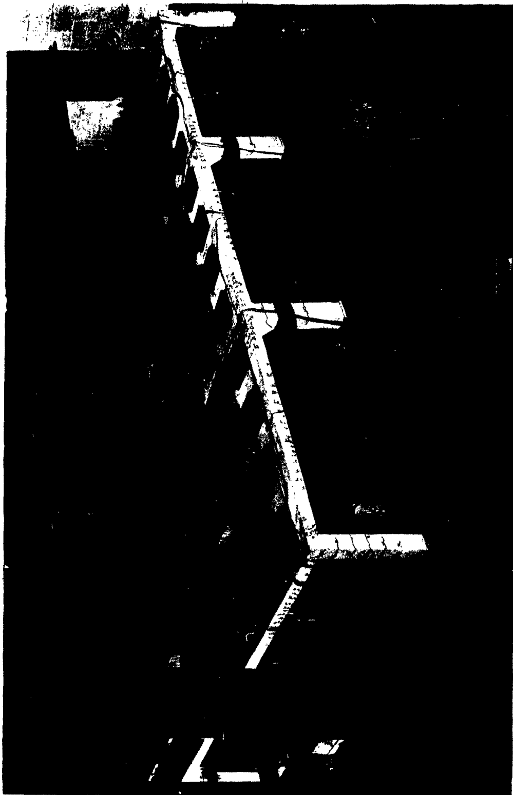
FIG. 5.1 VIEW OF FLAT SLAB (F2)
