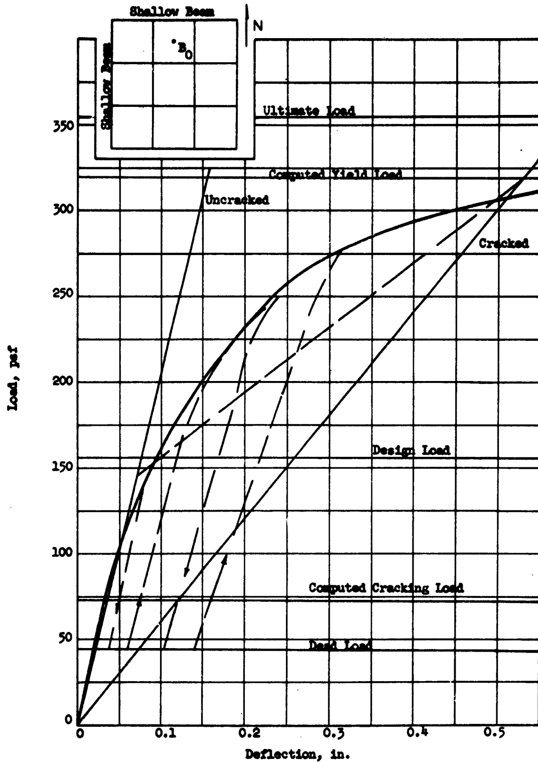
FIG. 5.41 LOAD-DEFLECTION CURVE, FLAT PLATE (F1), POINT B 0
