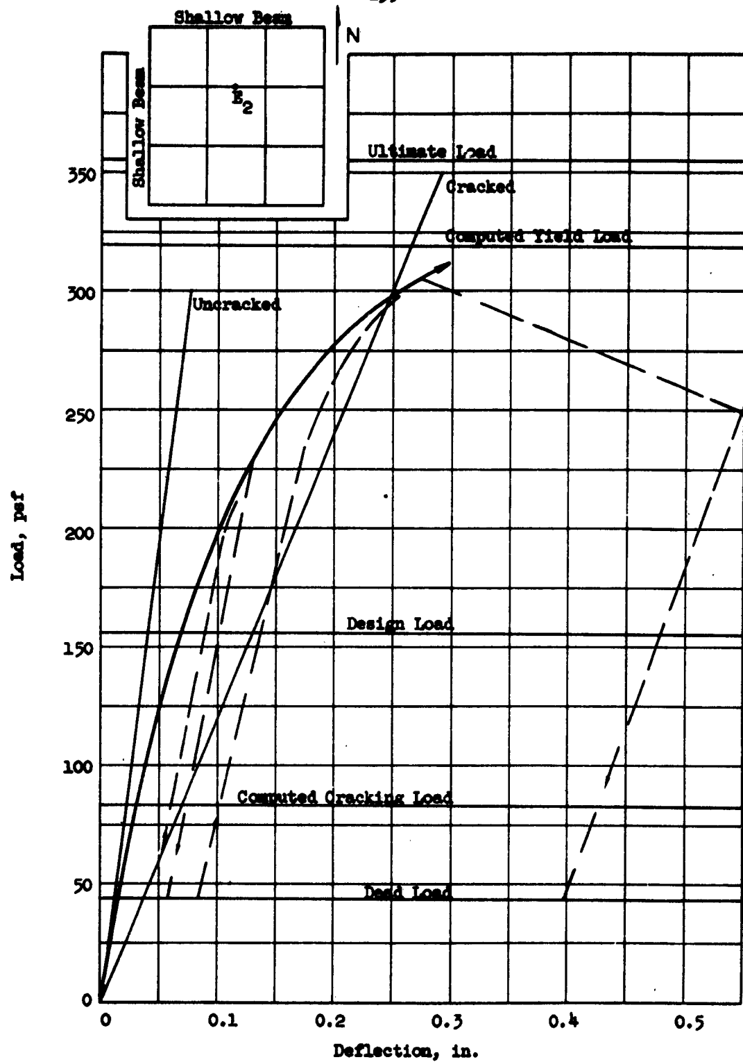
FIG. 5.46 LOAD-DEFLECTION CURVE, FLAT PLATE (F1), POINT E_2
