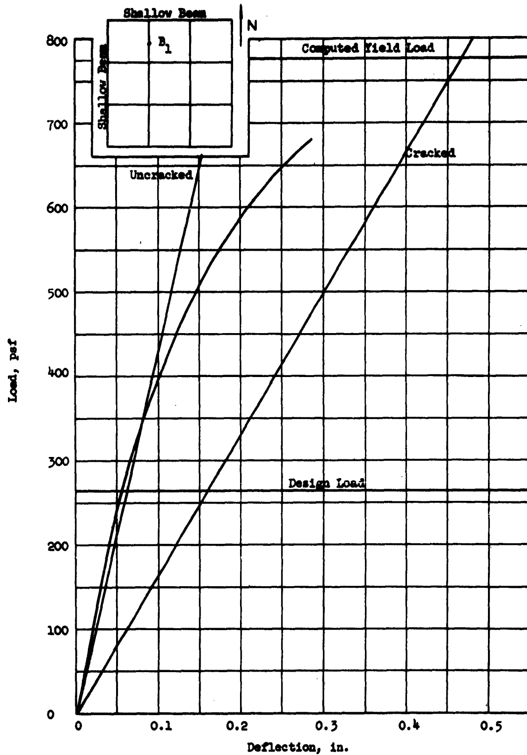
FIG. 5.84 LOAD-DEFLECTION CURVE, FLAT SLAB (F5), POINT B_1
