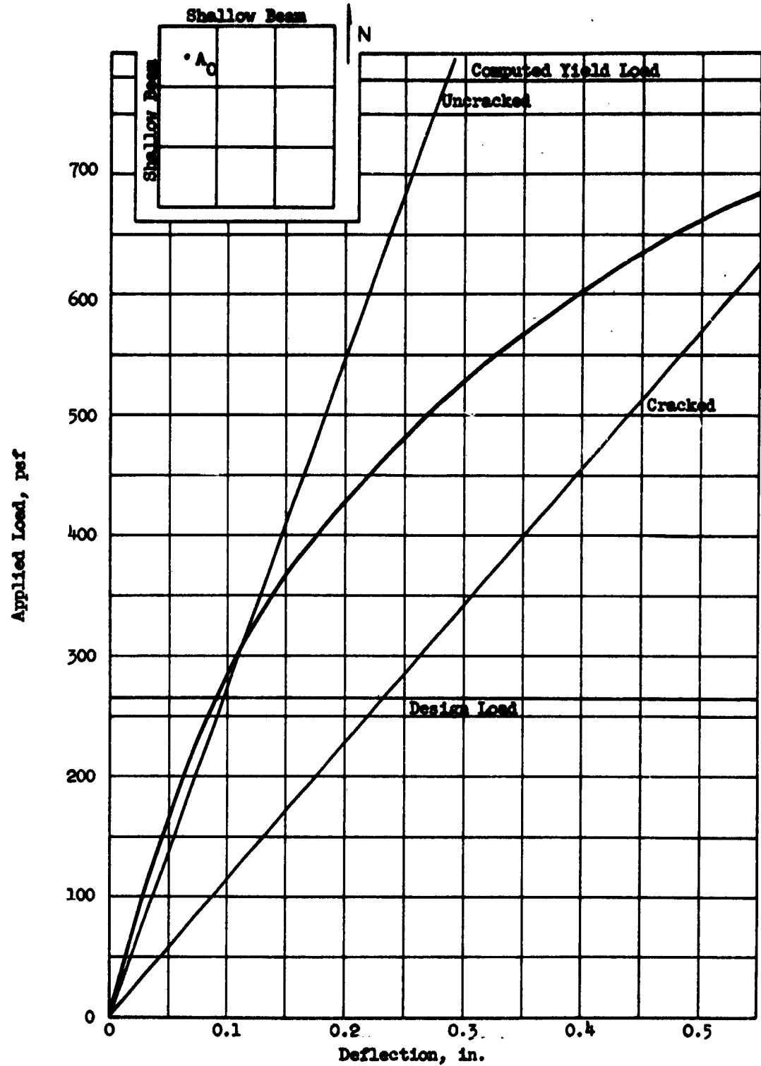
FIG. 5.82 LOAD-DEFLECTION CURVE, FLAT SLAB (F5), POINT A 0
