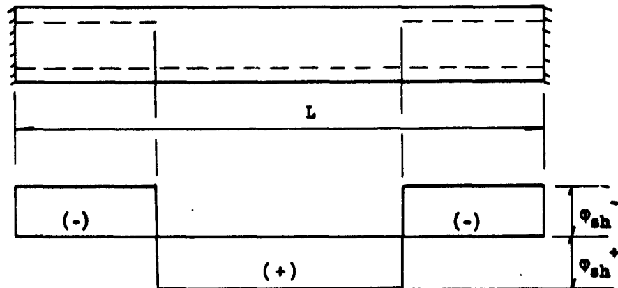
(b) Fixed-Ended Beam
