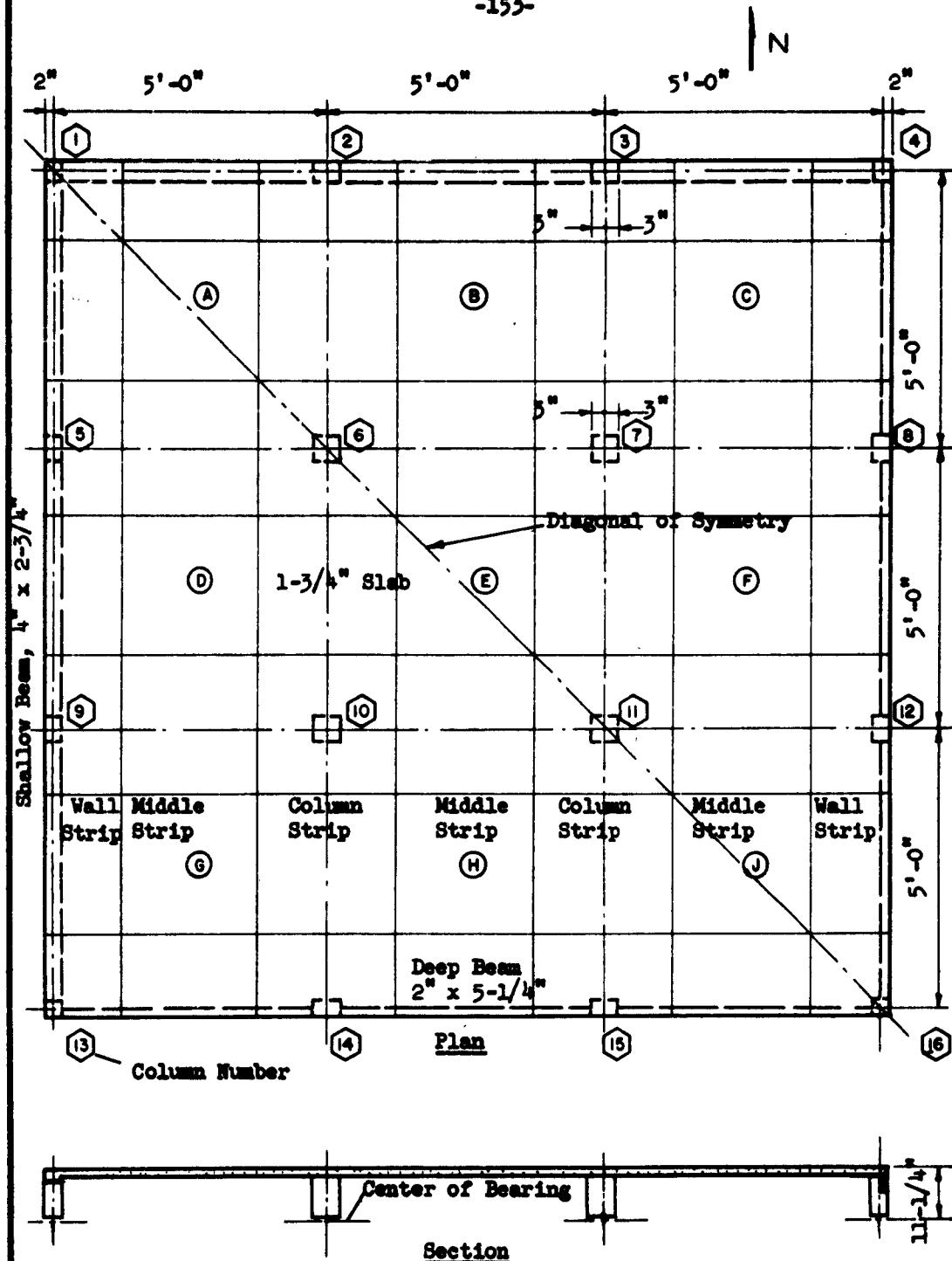
FIG. 5.4 LAYOUT OF FLAT PLATE TEST STRUCTURE (F1)
