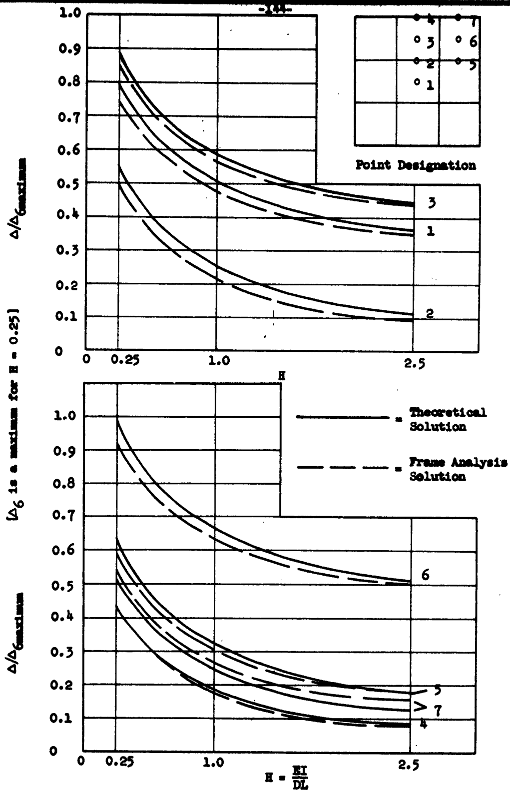
FIG. 4.10 COMPARISONS OF THEORETICAL AND FRAME ANALYSES SOLUTIONS, J = 1.0 , K = 90 , ALL PANELS LOADED
