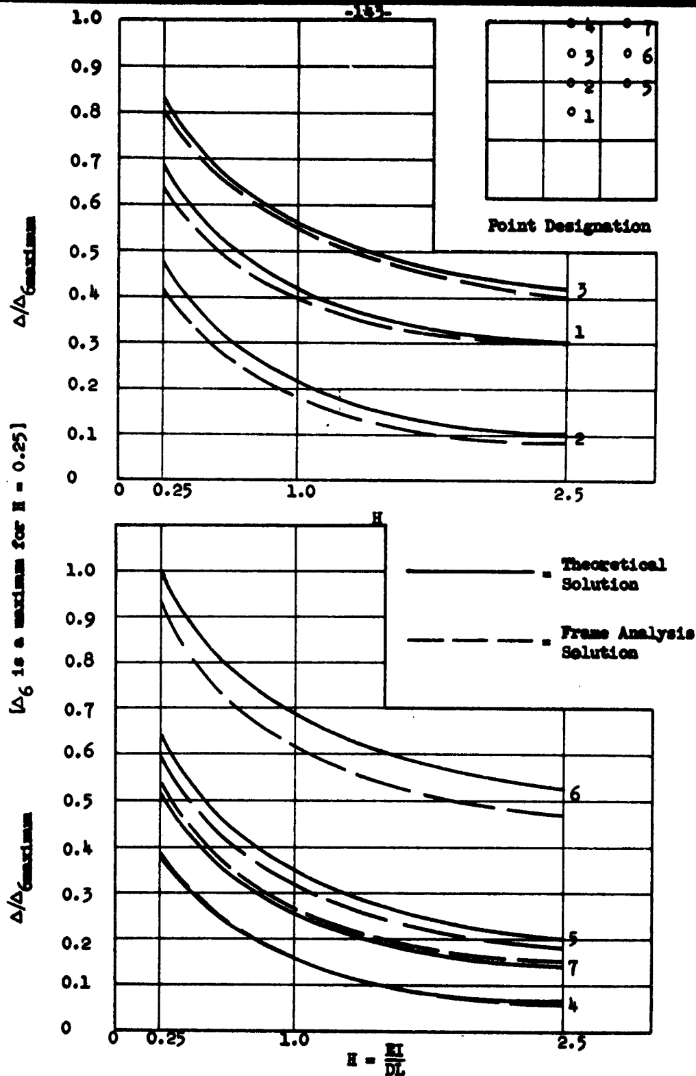
FIG. 4.9 COMPARISONS OF THEORETICAL AND FRAME ANALYSIS SOLUTIONS, J = 1.0 , K = 30 , ALL PANELS LOADED
