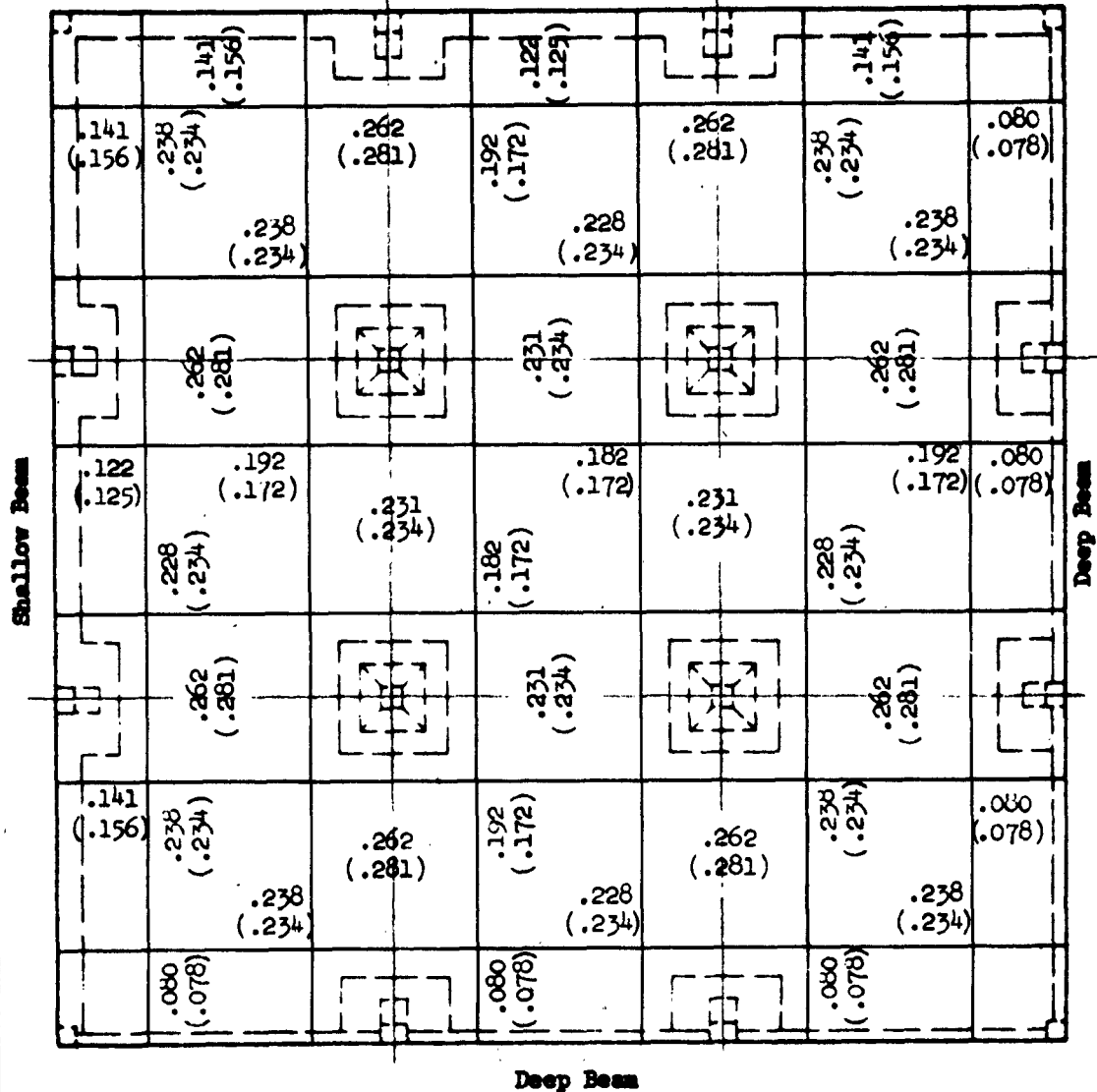
FIG. 5.14 COMPARISON OF CROSS-SECTIONAL AREAS OF SLAB POSITIVE REINFORCEMENT PROVIDED IN TEST STRUCTURES NO. 2 AND NO. 5
