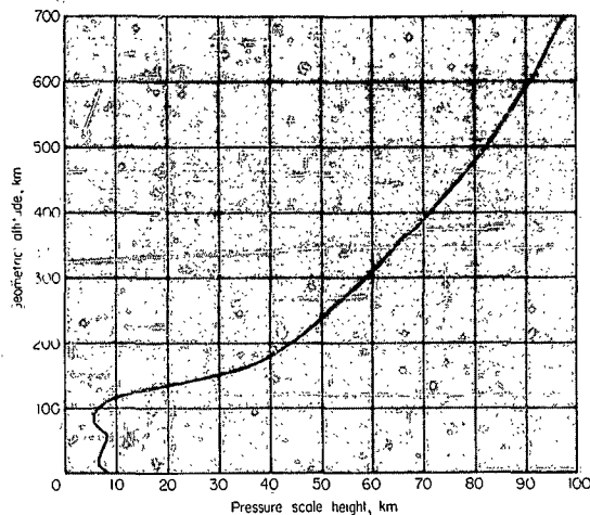
FIGURE I.3.2.—Pressure scale height H_P as a function of geometric altitude Z .
