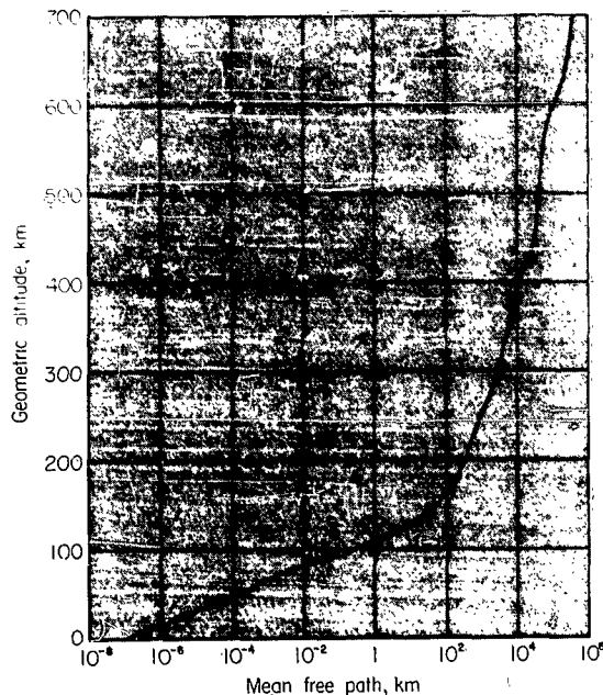
FIGURE I.3.5.—Mean free path L as a function of geometric altitude Z .
