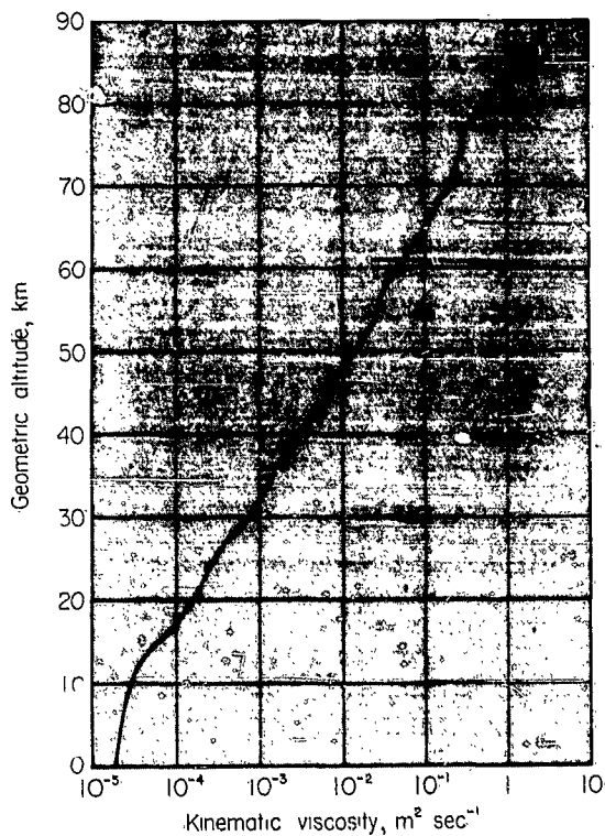
FIGURE I.3.9.—Kinematic viscosity \eta as a function of geometric altitude Z .
