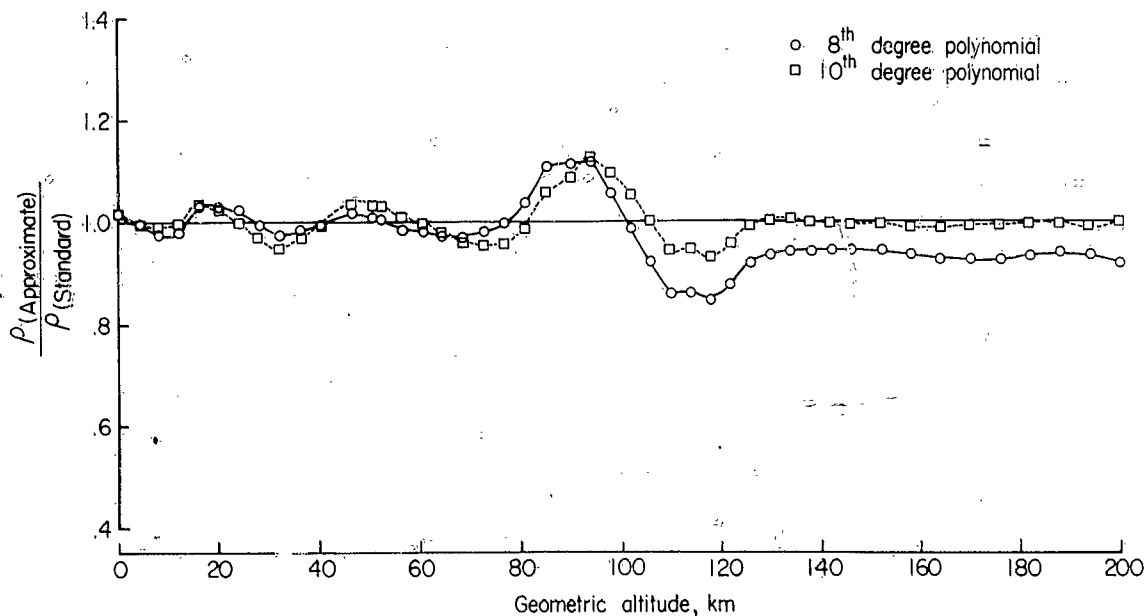
FIGURE II.3(c).—Ratio of approximate density to standard density for various altitudes.
