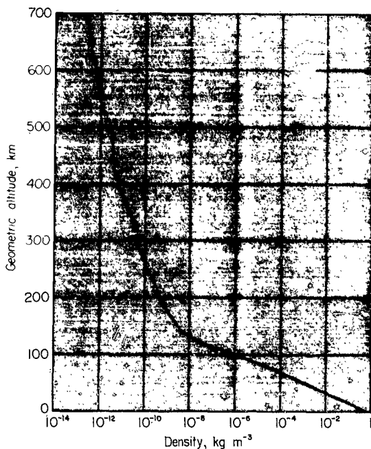
FIGURE I.2.11.—Density \rho as a function of geometric altitude Z .
