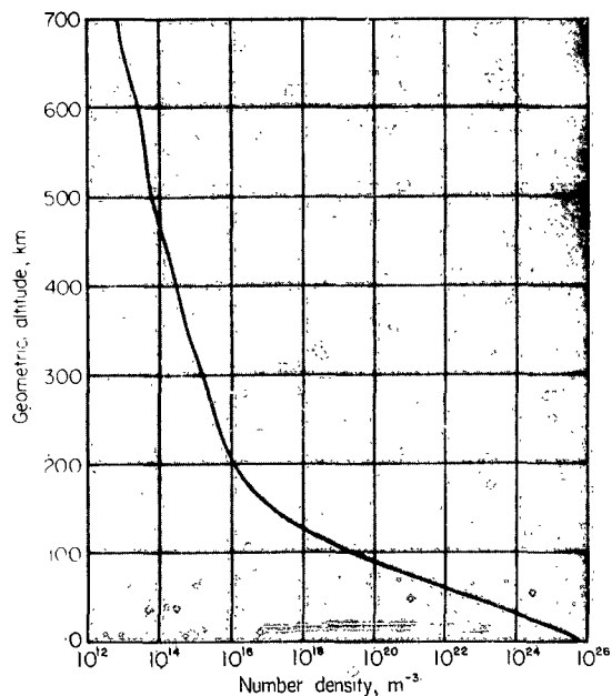
FIGURE I.3.3.—Number density n as a function of geometric altitude Z .
