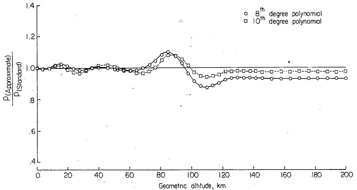
FIGURES II.3(b).—Ratio of approximate pressure to standard pressure for various altitudes.
