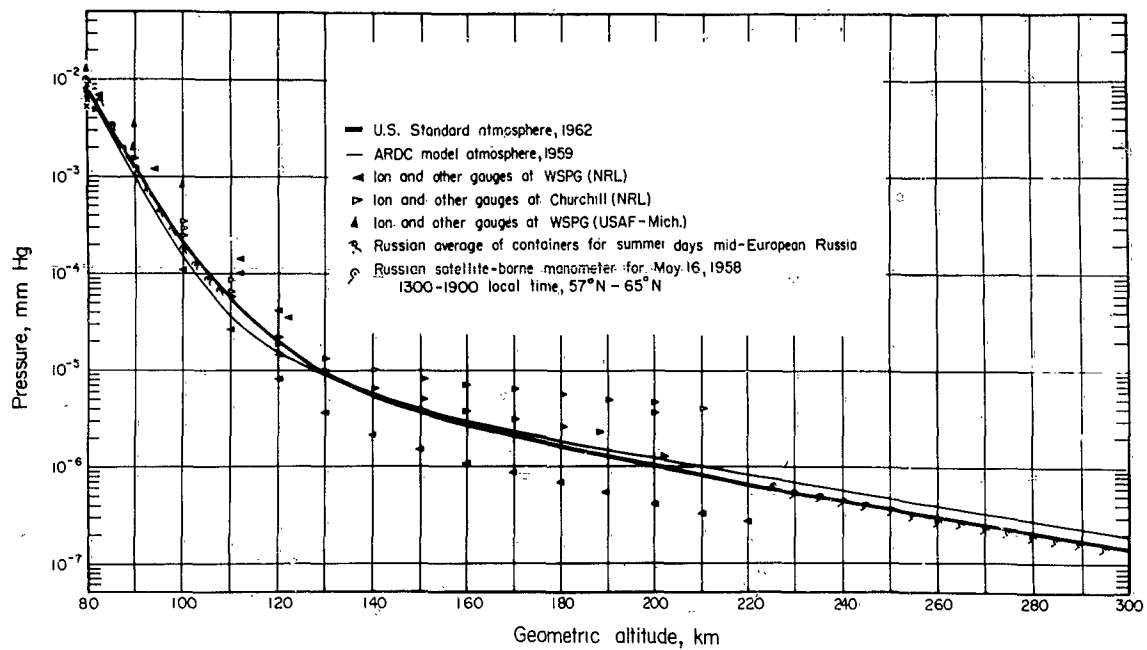
FIGURE II.2.2(c).—Pressures of U.S. Standard Atmosphere, 1962 compared with ARDC Model Atmosphere, 1959 and with available data.
