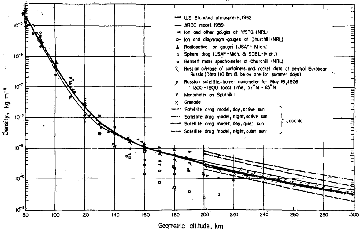
FIGURE II.2.2(b).—Density of U.S. Standard Atmosphere, 1962 compared with ARDC Model Atmosphere, 1959 and with available data.
