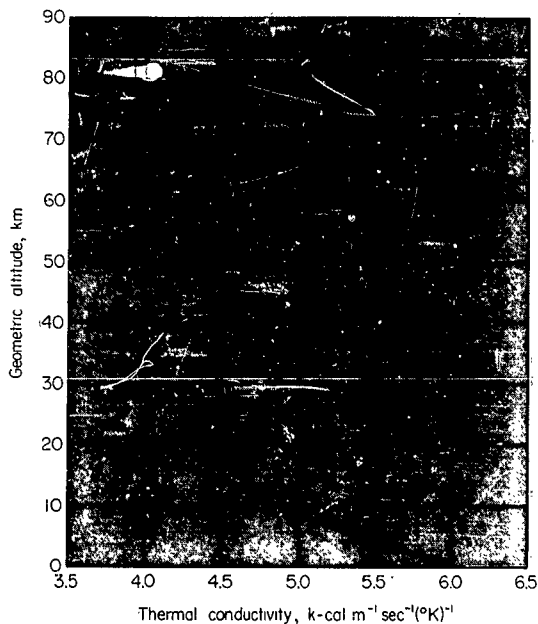
FIGURE I.3.10.—Coefficient of thermal conductivity k as a function of geometric altitude Z .
