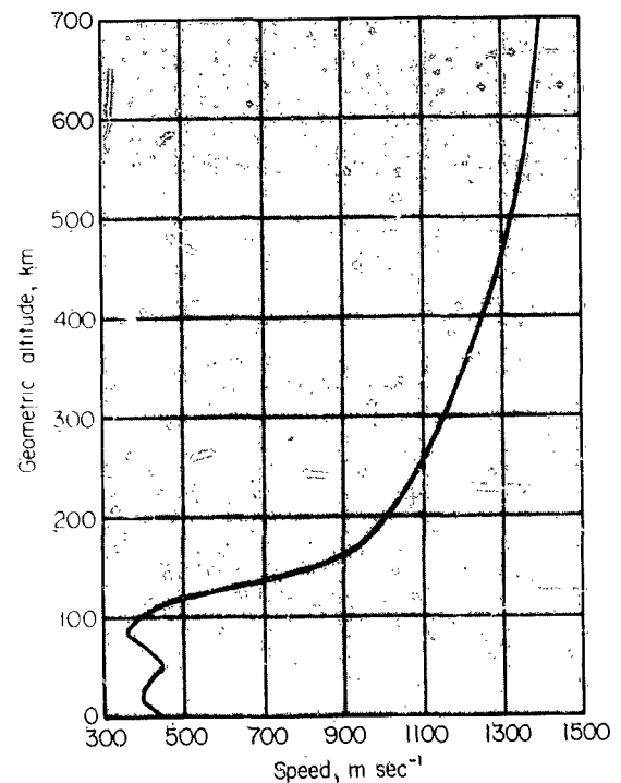
FIGURE I.3.4.—Mean particle speed \bar{V} as a function of geometric altitude Z .
