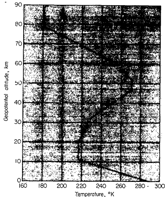
FIGURE I.2.6(b).—Temperature T as a function of geopotential altitude H . ( T_M=T below Z=90 km or H=88.743 km.)
