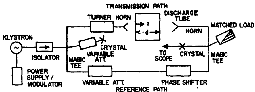
Fig. 4. Simplified block diagram of experimental set-up.
