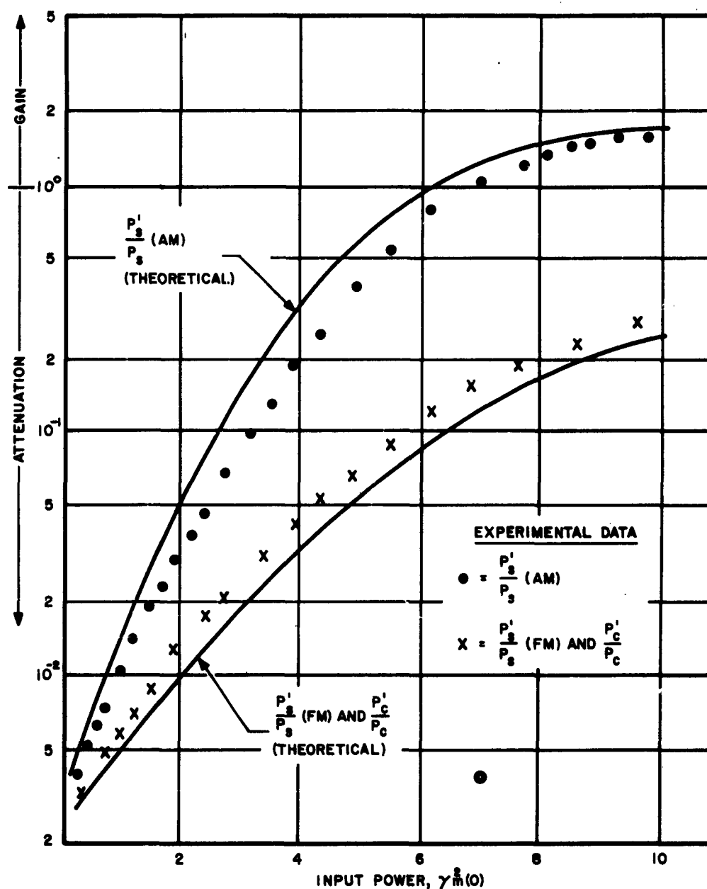
Figure No. 3. Gain and attenuation characteristics showing the sideband power ratio for amplitude modulation, P'_s/P_s (AM), for frequency modulation, P'_s/P_s (FM), and saturating component ratio, P'_c/P_c , as a function of the normalized saturating component input power, \gamma_m^2(0) . The modulation frequency, \Delta\nu , is 70 cps and \alpha L = 6.0 .
