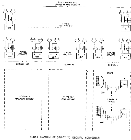
Figure 11 - Block Diagram of B to D Converter
