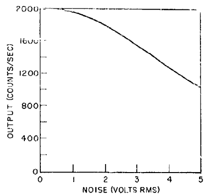
TIME-GATED SYSTEM OUTPUT FALL-OFF with NOISE (3V RMS SIGNAL)
