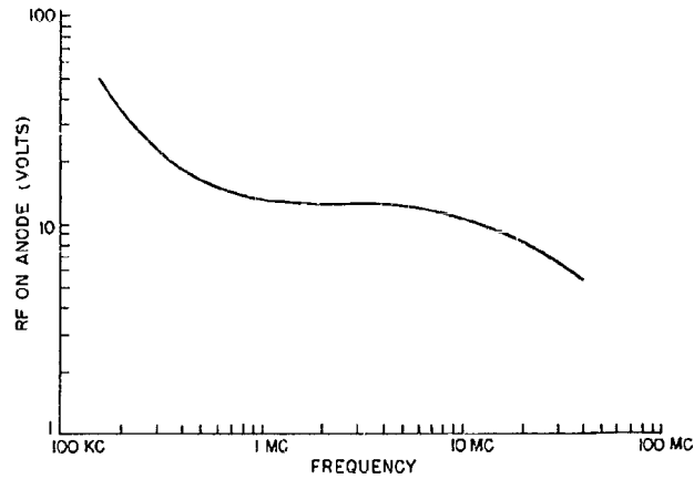
FIRING OF 2N1882 BY RF ON ANODE
