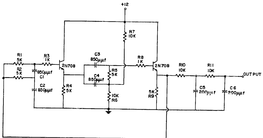
Figure 6 - RC Oscillator
