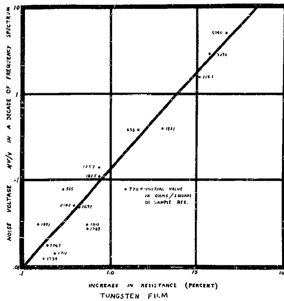
Fig. 17 - Current Noise Tungsten Film Resistors
