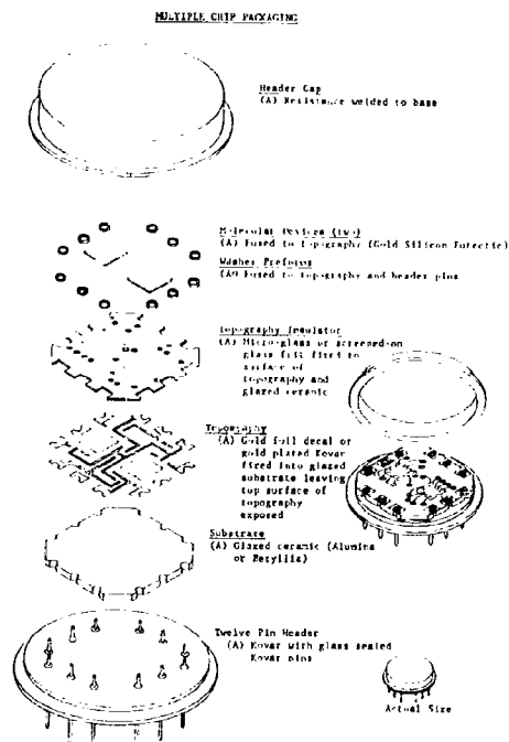
Figure 18 - Westinghouse Double- KAND Circuit Mounting
