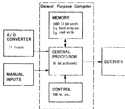
Figure 1 - Film Electronics Computer (Block Diagram)
