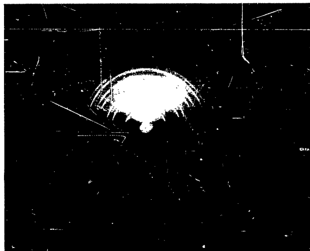
Figure 3-21. Electron Diffraction Pattern of Silicon Film Substrate Temperature 581°C
