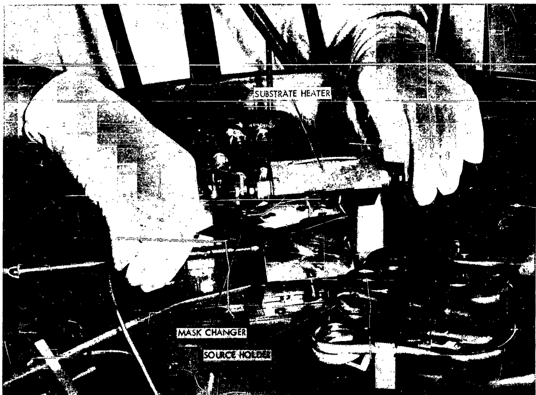
Figure 3-5. View of Vacuum Chamber Showing Substrate Heater, Mask Changer, and Source Holders
