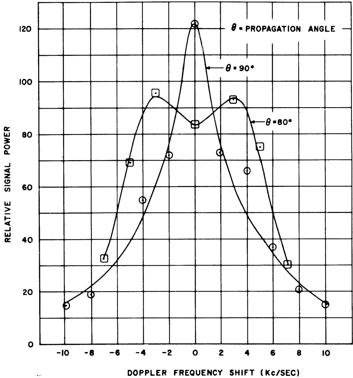
Figure 6. Effect of the Earth's Magnetic Field on the Spectrum of Incoherent Backscatter Observed at 425 Megacycles at Trinidad, 26 January 1961 (after Pineo, Kraft, Briscoe and Hynek)
