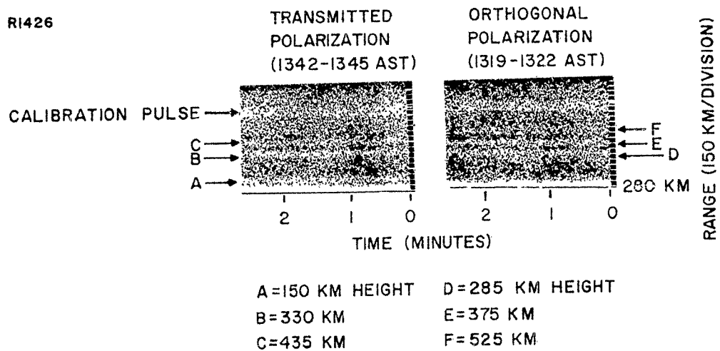
Figure 10. Range vs. Time Photographs of Incoherent Backscatter Echoes Showing Faraday Rotation. Observations Taken at Trinidad at 10° Elevation Angle in the Direction of Bogota, Colombia, on 2 February 1961
