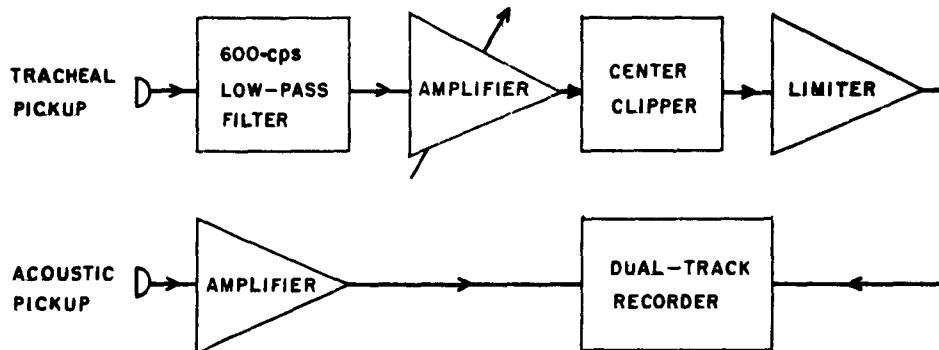
FIG. 10. Block diagram of the test setup.
