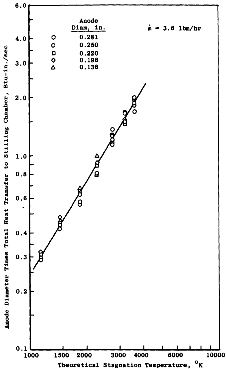
Fig. 10 Effect of T_o on Stilling Chamber Heat Transfer without Heat Shield
