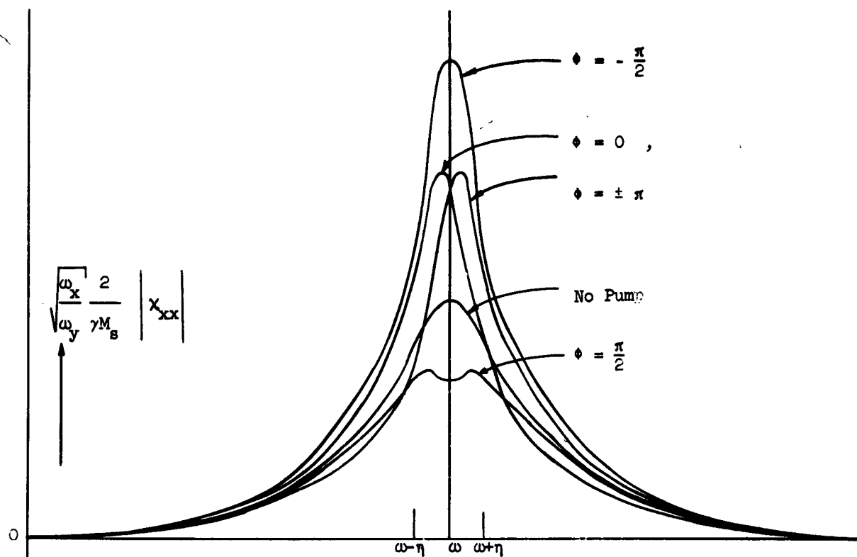
FIG. 2a--Magnitude of \chi for \frac{h_{\parallel}}{h_{\text{crit}}} = \frac{1}{2} .
