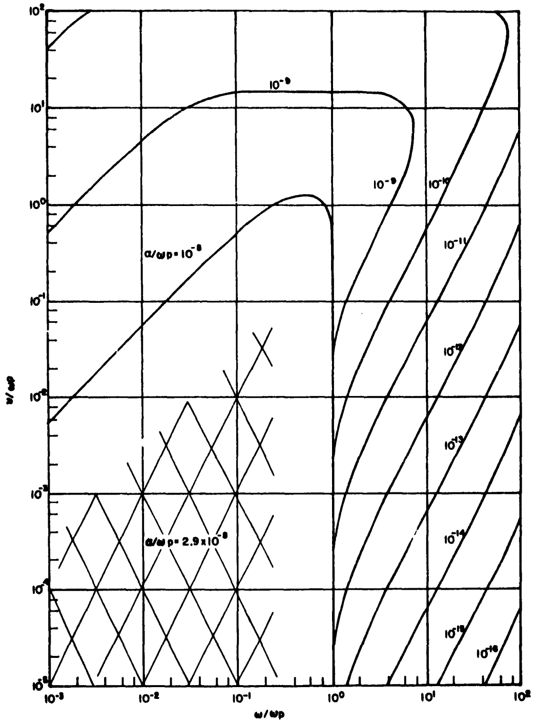
Fig. 2-1 Normalized Attenuation Constant
