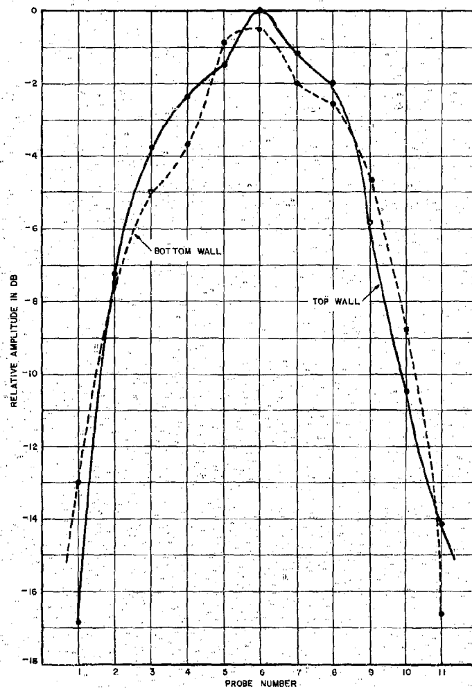
FIGURE 18. MEASURED TE 10 ELECTRIC-FIELD AMPLITUDE AT 4.3 GC
