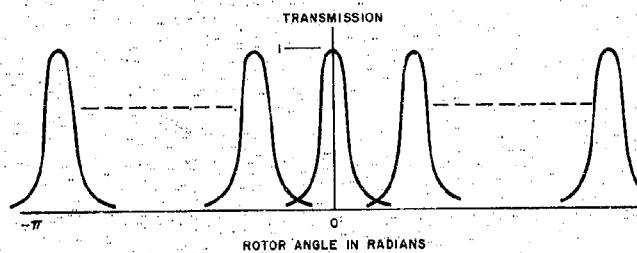
FIGURE IV-2. TRANSMISSION AS A FUNCTION OF ROTOR ANGLE FOR ALL COMMUTATOR SEGMENTS.
