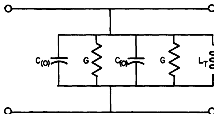
ASSUMED LOW POWER EQUIVALENT CIRCUIT
