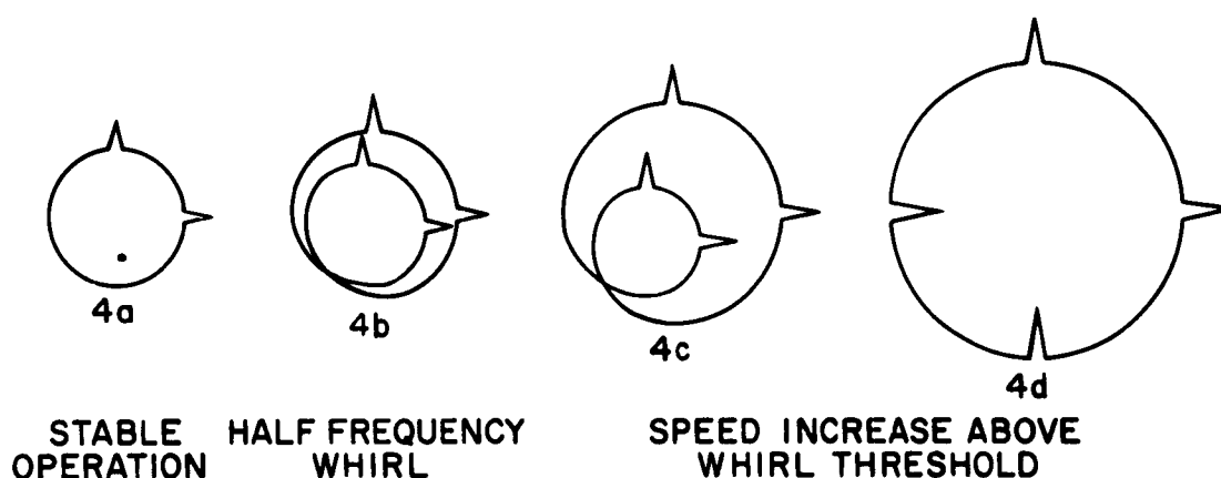
Figure 4 Rotor Center Whirl Paths Through Half-Frequency
