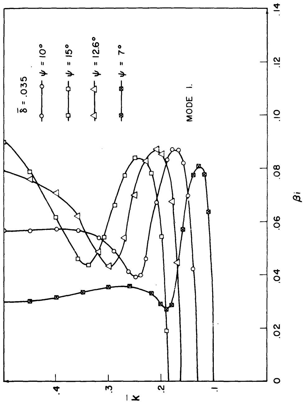
Figure 4.4b. The k - \beta_i diagram for the tape helix: Mode 1; \bar{\delta} = .035 , \psi = 7^\circ, 10^\circ, 12.6^\circ, 15^\circ .
