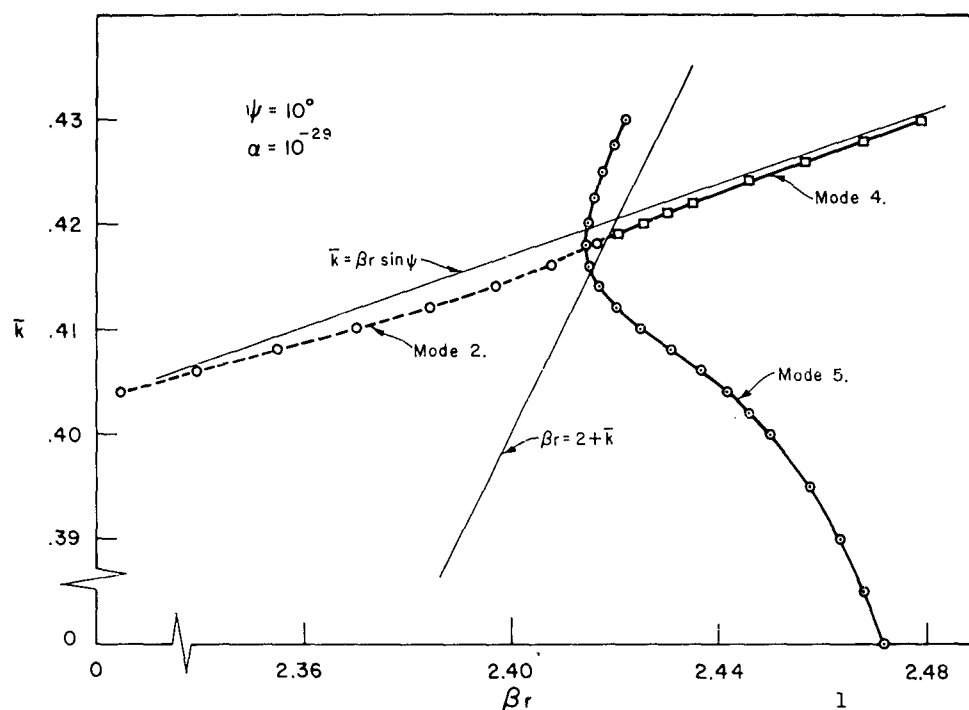
Figure 4.15a. The \bar{k} - \beta_r diagram for the tape helix near \bar{k}_{c4}^1 : Modes 2, 4 and 5; \psi = 10^\circ , \alpha = 10^{-29} .
