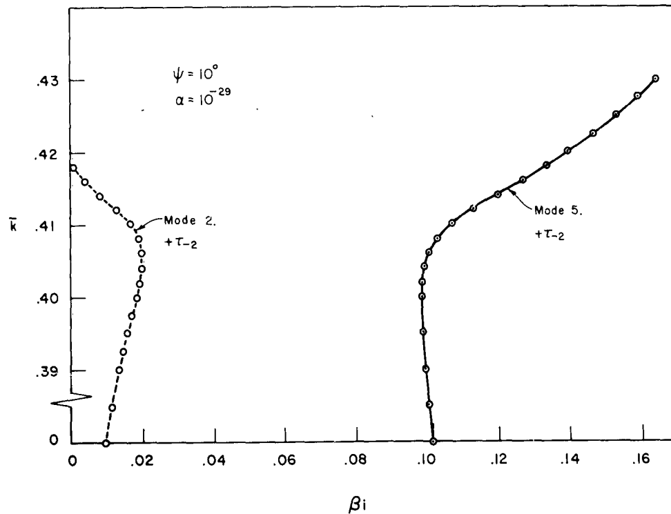
Figure 4.15b. The \bar{k} - \beta_i diagram for the tape helix near \bar{k}_{c4}^1 : Modes 2, 4 and 5; \psi = 10^\circ , \alpha = 10^{-29} .
