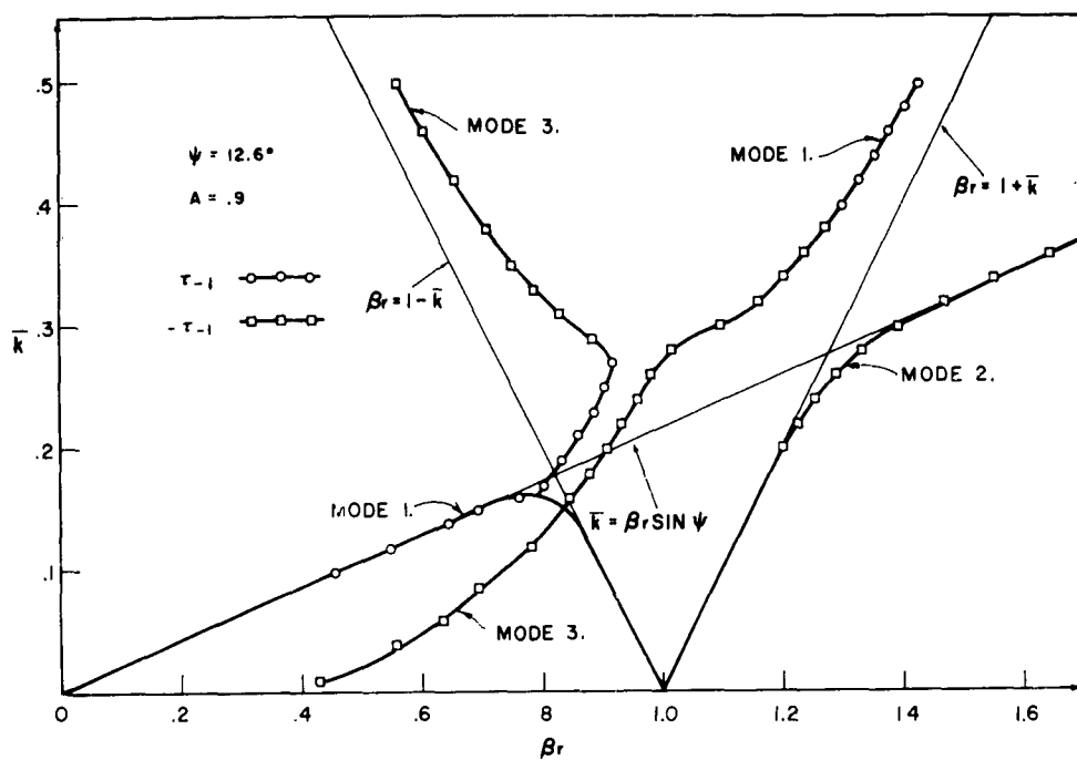
Figure 3.1a. The \bar{k} - \beta_r diagram for simplified equation one; A = .9 , \psi = 12.6^\circ .
