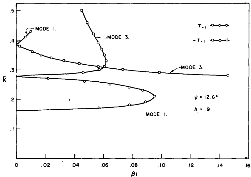
Figure 3.1b. The \bar{k} - \beta_l diagram for simplified equation one; A = .9 , \psi = 12.6^\circ .
