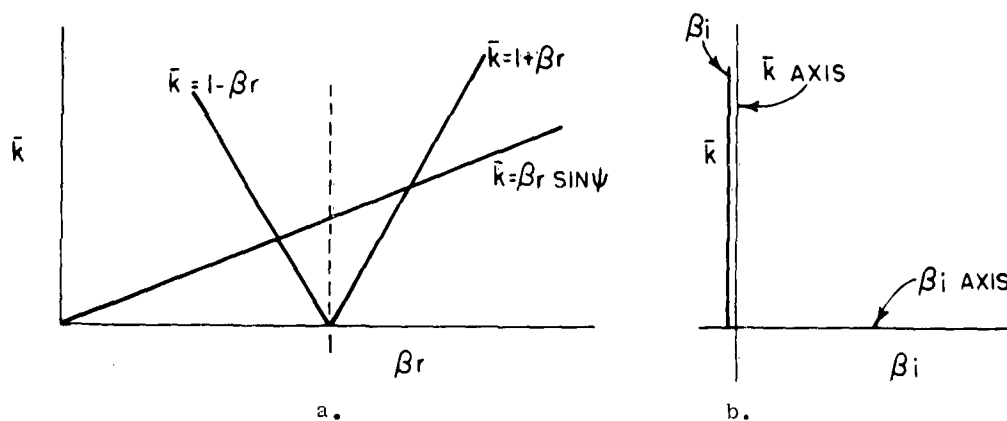
Figure 2.2. A k - \beta diagram for consideration of T_{-1} .
