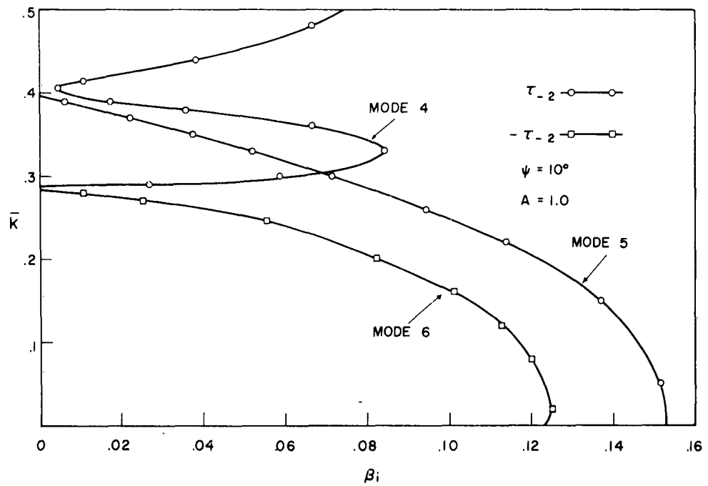
Figure 3.11b. The k - \beta_i diagram for simplified equation two; A = 1.0 , \psi = 10^\circ .
