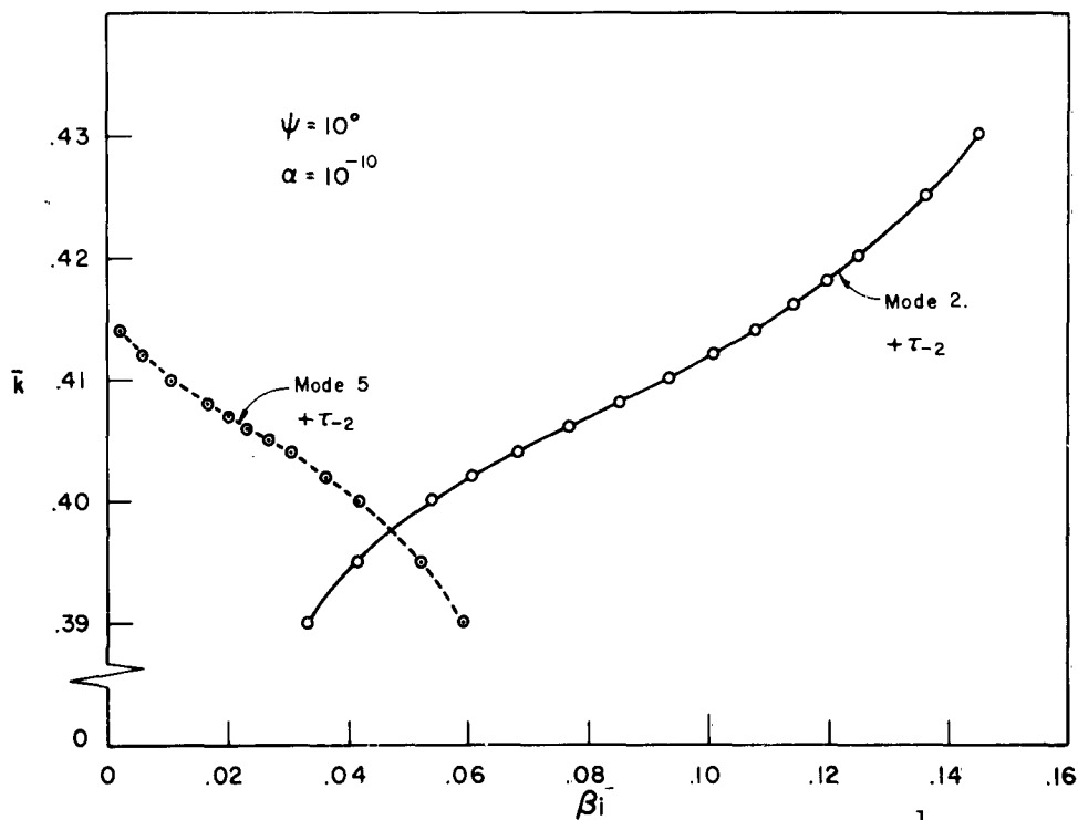
Figure 4.11b. The k - \beta_i diagram for the tape helix near k_{c4}^1 : Modes 2, 4 and 5; \psi = 10^\circ , \alpha = 10^{-10} .
