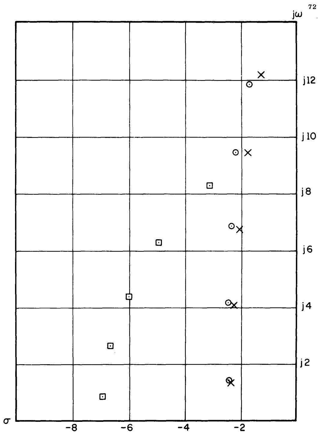
Figure 21. The upper half-plane pole distributions for x weighted ripple, \epsilon_1 = 0.01 , \epsilon_2 = 0.16 ; \odot equiripple, \epsilon = 0.01 ; \square Bessel. All configurations unity delay
