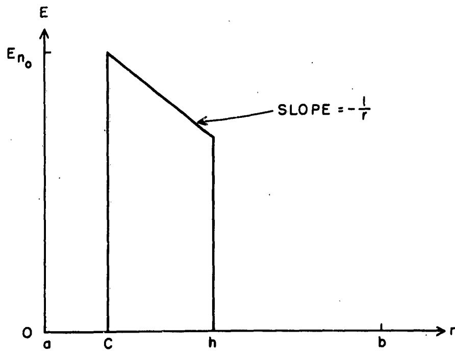
Figure 3. Assumed Coupling Iris Field ( z = L ).
