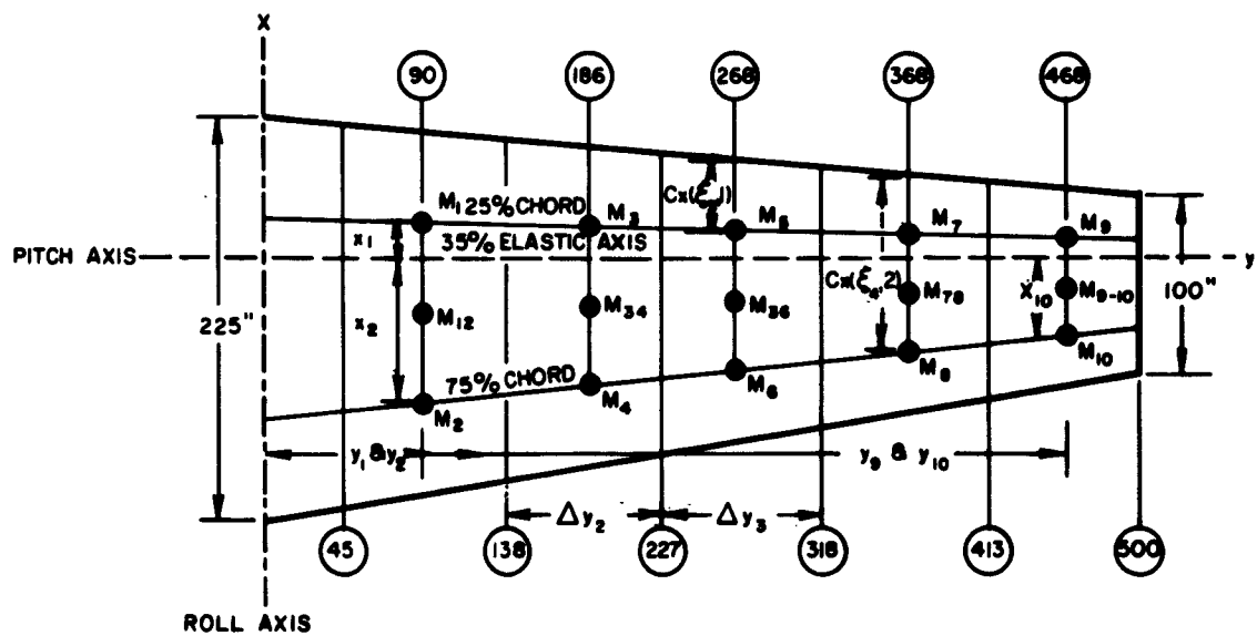
Fig. 1. Jet transport wing geometry.
