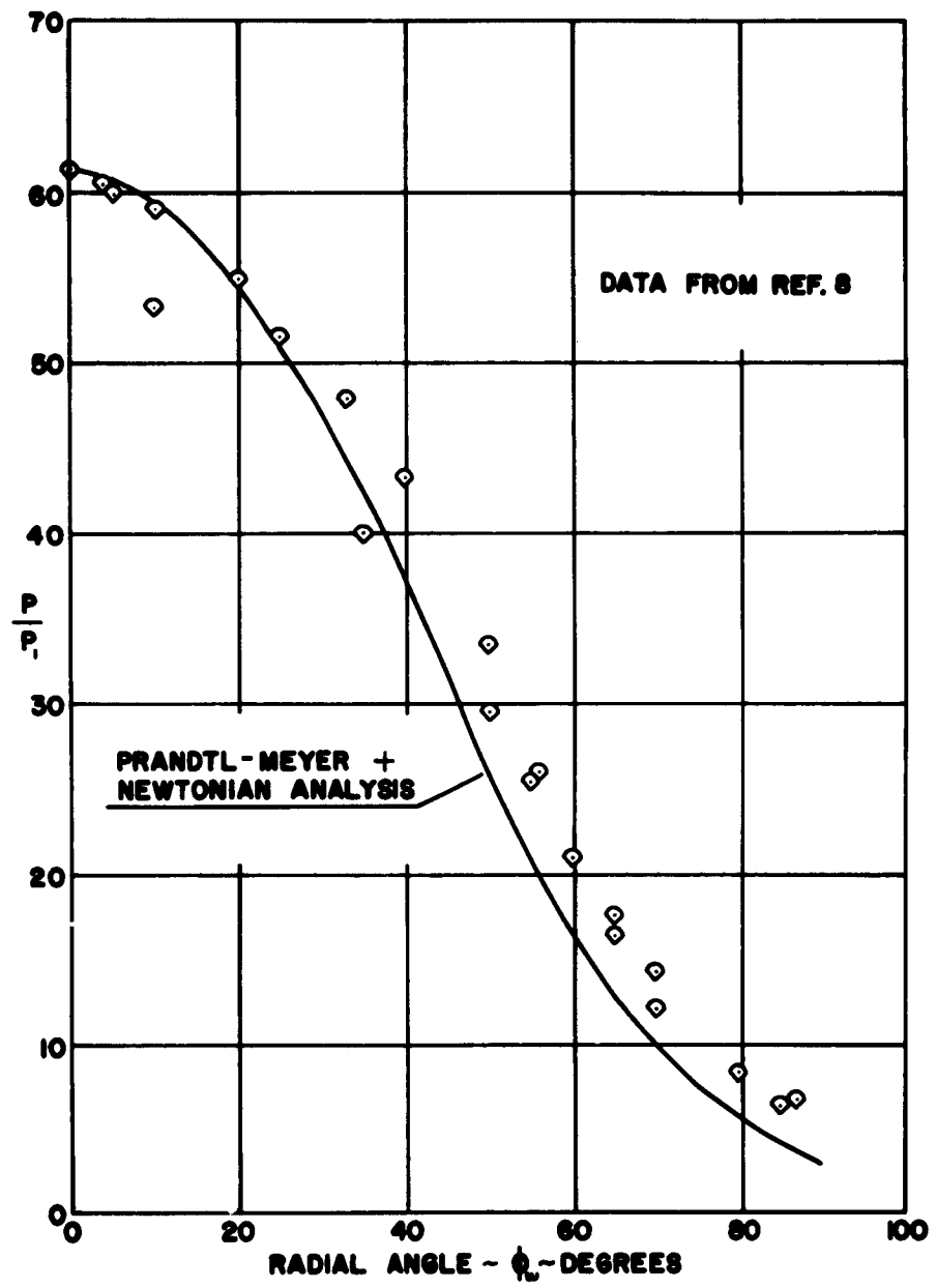
FIGURE 1. PRESSURE DISTRIBUTION OVER A CYLINDRICAL BODY AT M_i = 6.86
