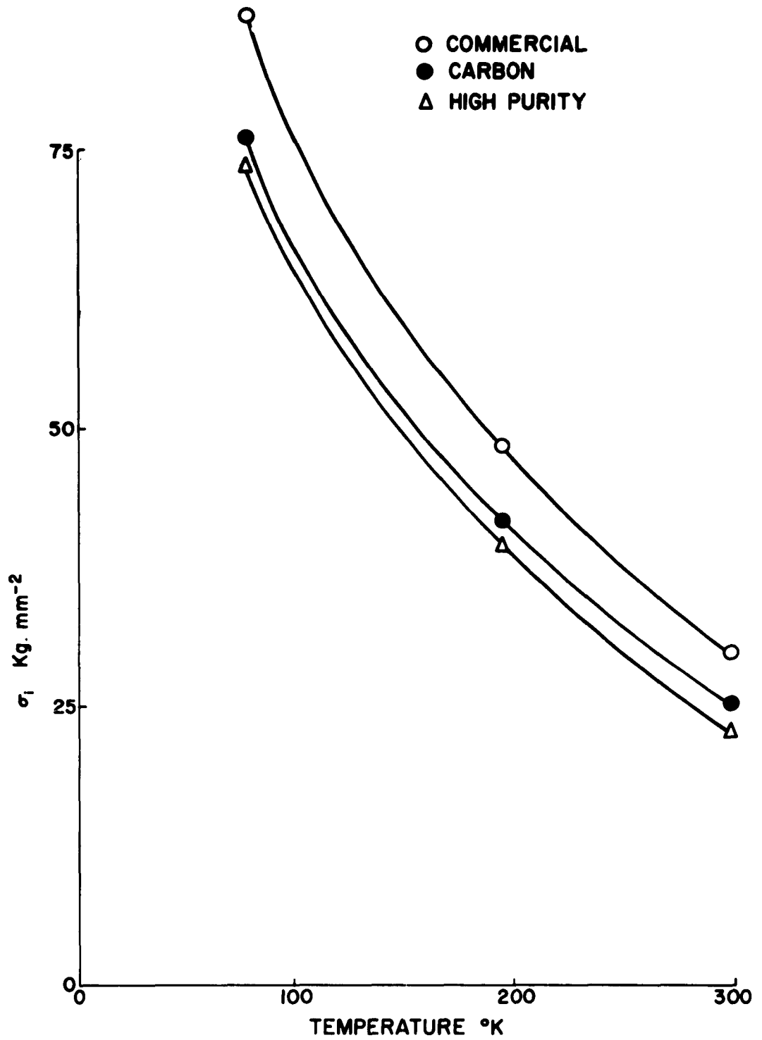
FIG. 17. COMPARATIVE \sigma_1 TEMPERATURE BEHAVIOR FOR A STRAIN RATE OF 10^{-1}/\text{sec} .
