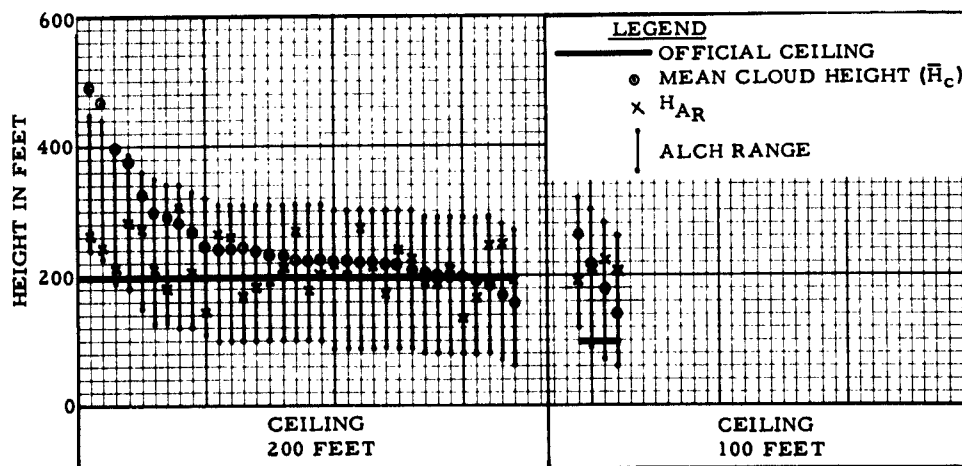
FIG. 27e OFFICIAL CEILINGS SHOWING \bar{H}_C , H_{AR} , AND ALCH RELATIONSHIPS - DAY - (CEILINGS OF 200 FEET AND 100 FEET)
