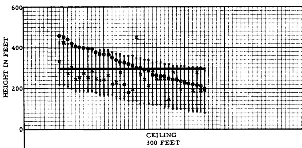
FIG. 27d OFFICIAL CEILINGS SHOWING \bar{H}_C , H_{AR} , AND ALCH RELATIONSHIPS - DAY - (CEILINGS OF 400 FEET AND 300 FEET)
