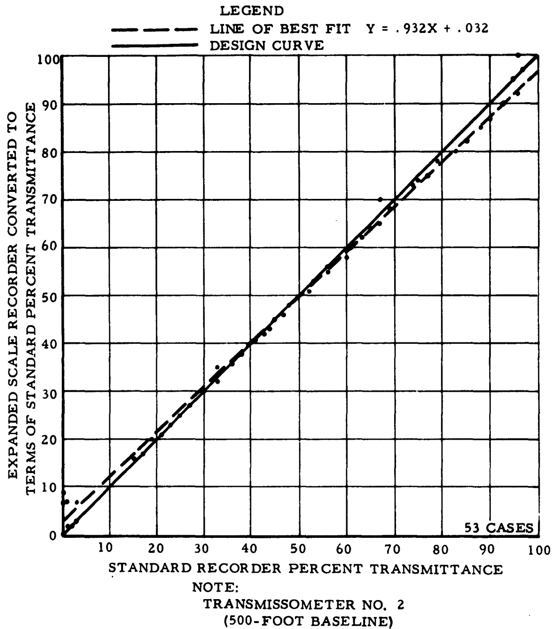
FIG. 45 PLOT OF DATA OBTAINED WITH RESPECT TO STIPULATION OF INSTRUMENTAL EQUILIBRIUM
