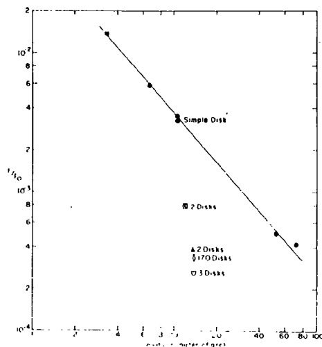
Fig. 6. Reduction of the flux into an objective aperture 1.2-mm diameter placed 76 cm behind various occulting disks. Here F is the flux observed with the occulting disk in place, while F_0 is the flux in the unobstructed beam. The reduction is plotted as a function of the difference between the diameter of the occulting disk and the diameter of the sun in min of arc. The synthetic sun was a ribbon filament lamp whose objective lens subtended an angle of 32 min of arc from the objective aperture.
